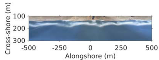
FIGURE 1. Planview of 10 June 2013 (11h) made of 5 time-exposure video images. The dry beach is in the upper part and white stripes (due to predominant wave breaking) correspond to shallow areas.
