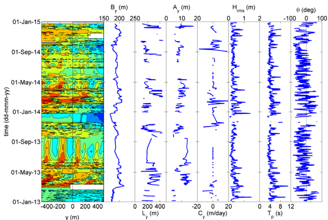
FIGURE 3. Time series during 2013-2014 of (from left to right) the cross-shore bar crest positions B_y(t) (timestack), sandbar position B_y (shoreline position was located around 150 m), wavelength L_y , amplitude A_y , alongshore migration speed C_y (positive for eastward migration), root-mean-square wave height H_{rms} , peak period T_p and angle of incidence \theta_{mean} with respect to the shore normal (positive angles are westerly wave). In the timestack, red colours denote bays (seaward perturbations) whilst blue colours denote horns (shoreward perturbations). The wave conditions are daily-averaged at 10 m depth.
