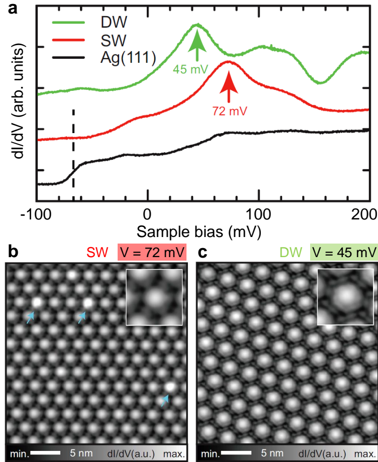
FIGURE 5.3: Local electronic structure of the SW and DW networks. (a) Conductance ( dI/dV ) spectra on the pristine Ag(111) ( black ), on the pore centers of the SW network ( red ) and DW network ( green ). (b, c) dI/dV maps on the SW and DW networks acquired on the peak maxima in (a), enlarged in the corresponding insets. Measurement parameters: I = 10 pA, V = 72 mV, modulation voltage V_{ac} = 10 mV, oscillation frequency f_{ac} = 513 Hz (b); I = 10 pA, V = 45 mV, V_{ac} = 10 mV, f_{ac} = 515 Hz (c).
