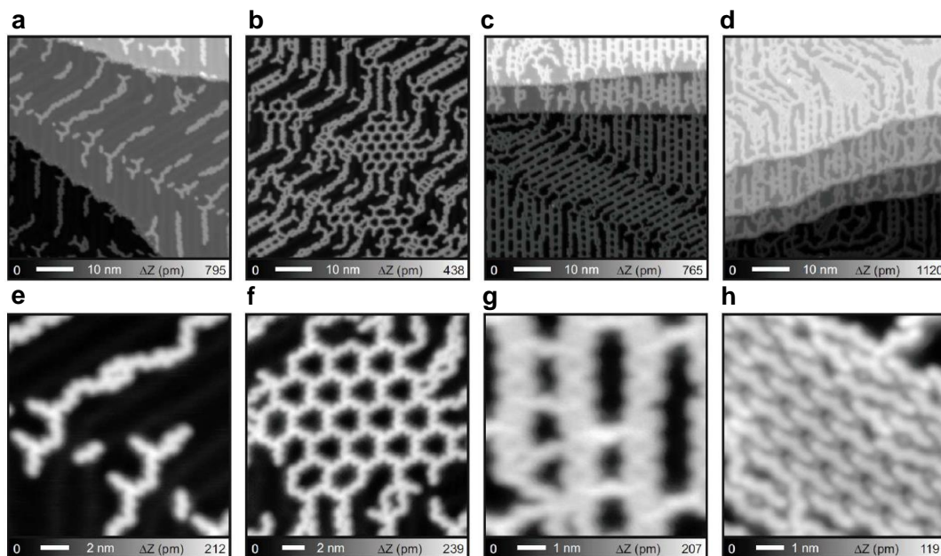
FIGURE 5.10: Molecular arrangements of Br-DNT deposited on Au(111) at 130 K. (a-d) A series of STM topographic images, with increasing molecular coverage and (e-h) corresponding close views. The surface corrugation prevents the long-range formation of 2D hexagonal molecular networks, facilitating chain structures following the herringbone reconstruction. We stress that if an ideally regular 2D porous network as the one observed in (f) would fully extend over the whole surface, the obtained band structure would be different from the SW and DW cases shown for Ag(111) because the pores have different symmetries (three-fold vs six-fold) and exhibits different inter-pore dimensions. Measurement parameters: V_{tip} = -200 mV for all images, I = 10 pA in (a) and (b); I = 2 pA in (c) and (d); I = 5 pA in (e); I = 20 pA in (f); I = 2 pA in (g); I = 20 pA in (h).
