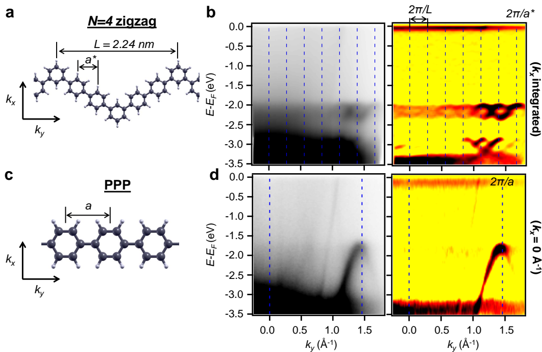
FIGURE 10.12: N=4 zigzag chain ARPES band structure comparison with that of PPP. Schematic representations of the N=4 zigzag chains (a) and the poly-( para -phenylene) chains (c). (b) and (d) show their respective raw (left) and second derivative (right) of the ARPES spectral intensity ( E vs k_y ) along the chain axis. These plots follow the periodicity of the chain unit cells ( \frac{2\pi}{L} and \frac{\pi}{a} ) marked with vertical dashed blue lines. For the PPP polymer film the substrate used is a Ag(544) vicinal crystal.
