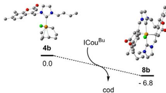
Figure 7. Energy profile for the formation of 8b from 4b and coumarin-functionalized NHC ( \Delta G , kcal mol -1 ).
