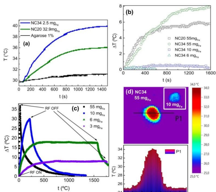
Figure 7: Heating curves of NCs measured in the portable applicator at 100 kHz and 9.3 \text{ kA m}^{-1} in a) homogenously dispersed in 700 \mu\text{L} of agarose-gel-phantoms and b) in tumour tissue, displayed as temperature increase relative to control. c) Heating curve of NC34 in tumour tissue at 265 kHz and 40 \text{ kA m}^{-1} . d) Thermal image of heated tumour after recording the heating curve shown in b). Inset in d): thermal image of a tumour injected with 10 mg Fe of NC34, no heating was observed after RF application with optical fiber (panel b) nor with thermal image.
