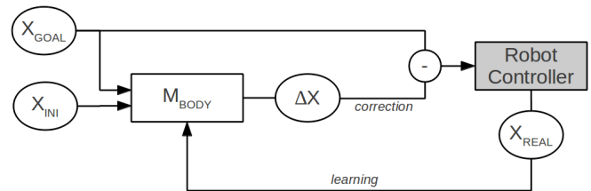
Fig. 13. Schematic of the action correction mechanism using the body model. The desired action and the current position of the end-effector is fed into the model, which provides corrections for the position, as well as an estimate of the temporal error in reaching that position.
