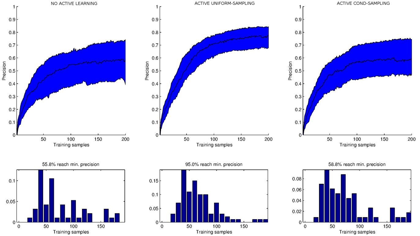
Fig. 6. Results for the three strategies applied to discover goal sound regions. NO ACTIVE LEARNING consists in taking a random sample from the distribution conditioned on the goals. The active learning strategies are UNIFORM-SAMPLING, which takes the sample candidates from the prior distribution on locations, and COND-SAMPLING, which uses the distribution conditioned on the goals to obtain the candidates.
