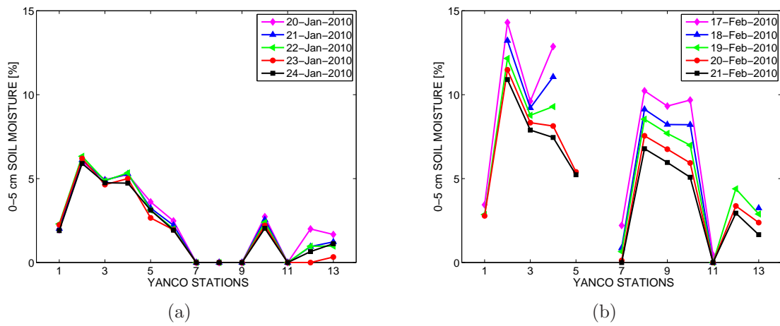
Figure 6.12 Spatial variability of 0-5 cm soil moisture measurements (6 am) of the 13 Yanco stations on days (a) January 20-24, 2010, and on (b) February 17-21, 2010.
