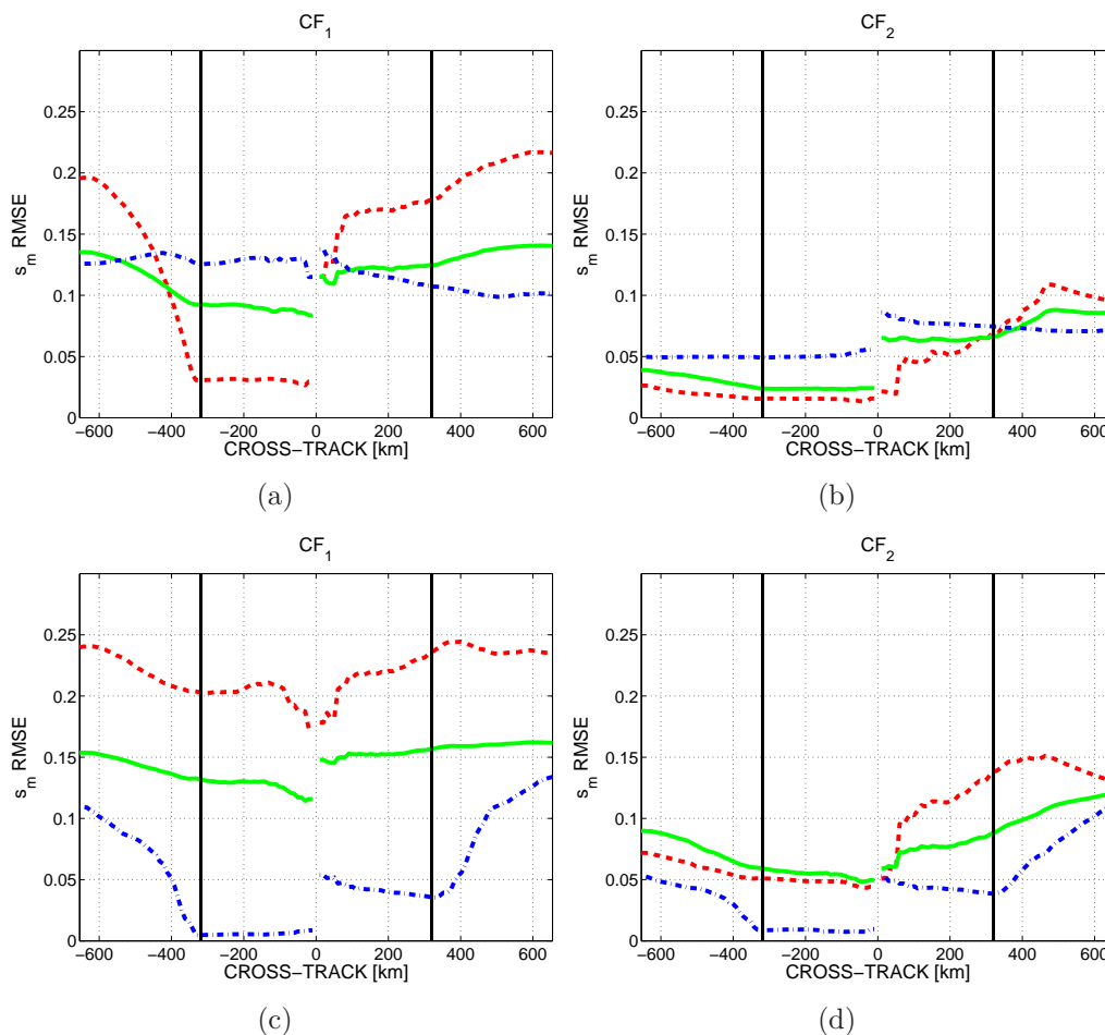
Figure 4.5 Retrieved soil moisture RMSE of simulated SMOS observations versus pixel position in the swath. Simulations over the dry (red, dashed lines), moist (green, solid lines), and wet (blue, dashed-dotted lines) scenarios of Table 4.1. First row: bare soil scenarios, second row: vegetation-covered scenarios. Left column: with no constraints on the cost-function ( CF_1 ), right column: adding constraints on all parameters, except s_m ( CF_2 ). In each plot: first Stokes parameter (left side of swath) and Earth’s reference frame (right side of swath). Vertical lines denote the Narrow Swath.
