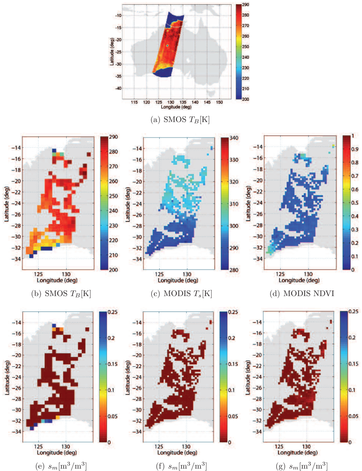
Figure 6.10 As for Fig. 6.6, but using an SMOS image over central Australia from December 8, 2009 (6 pm).
