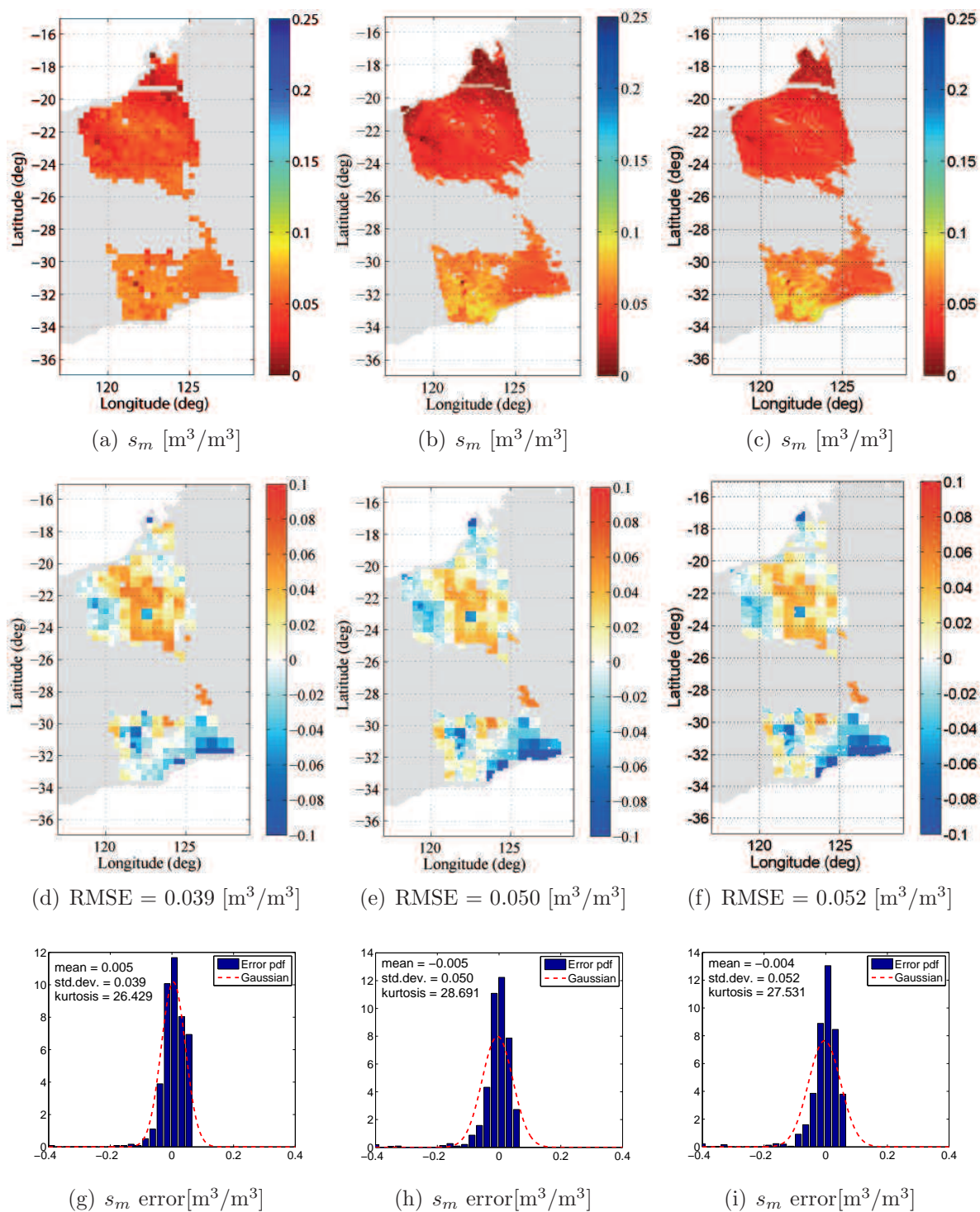
Figure A.3 As for Fig. 6.16, but using the linking model in (6.3).
