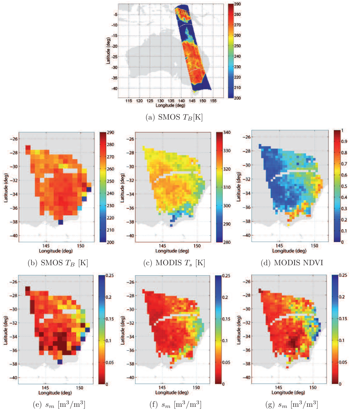
Figure 6.14 As for Fig. 6.6, but using an SMOS image covering the Murrumbidgee catchment, from January 22, 2010 (6 am).
