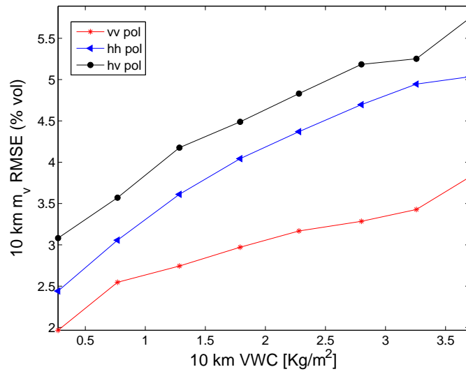
Figure 7.7 Plots of change detection RMSE at 10 km stratified by 0.5 \text{ kg/m}^2 vegetation water content values
