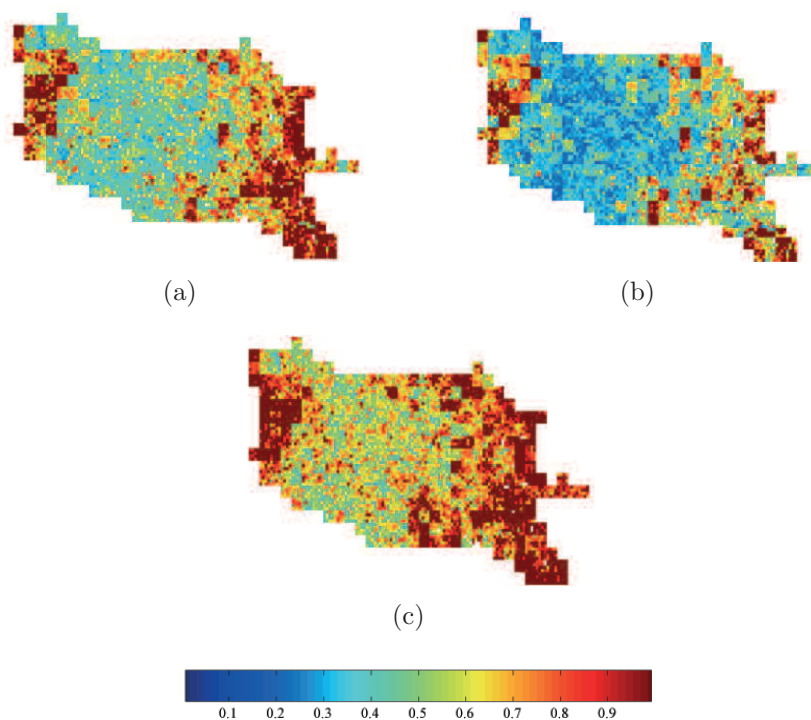
Figure 7.6 Ratio of change detection RMSE to radiometer only RMSE using (a) \sigma_{hh}^0 , (b) \sigma_{vv}^0 and (c) \sigma_{hv}^0 .
