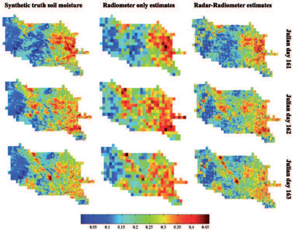
Figure 7.4 Sample results (three days) from the Observation System Simulation Experiment for the comparison of higher resolution (10 km) soil moisture estimates obtained using the active-passive method with synthetic ground truth soil moisture and with lower resolution (40 km) estimates obtained from a typical radiometer.
