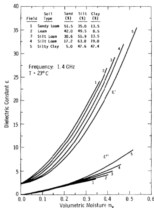
Figure 2.5 Measured dielectric constant at 1.4 GHz for five soils with different textural composition, from Hallikainen et al. [1985]
