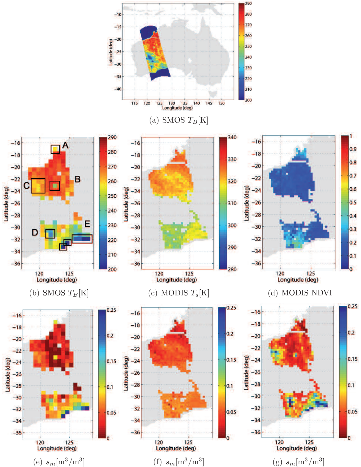
Figure 6.6 Sample results of the application of the algorithm to a SMOS image over western Australia, from December 8, 2009 (6 am). SMOS T_B image [K] on a 16 x 16 km grid (a). SMOS T_B image [K] on a 64 x 64 km grid (b). MODIS-derived T_s [K] (c) and NDVI (d) maps aggregated to 32 km. SMOS-derived soil moisture map [m 3 /m 3 ] at 64 km (e). SMOS-derived soil moisture maps [m 3 /m 3 ] at 32 km using the linking model in (6.3) (f), and using the linking model in (6.9) (g). Empty areas in the images correspond to clouds masking MODIS T_s measurements.
