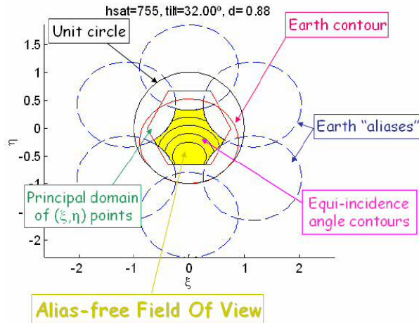
Figure 1.5 SMOS observation geometry, from Camps et al. [2005]
