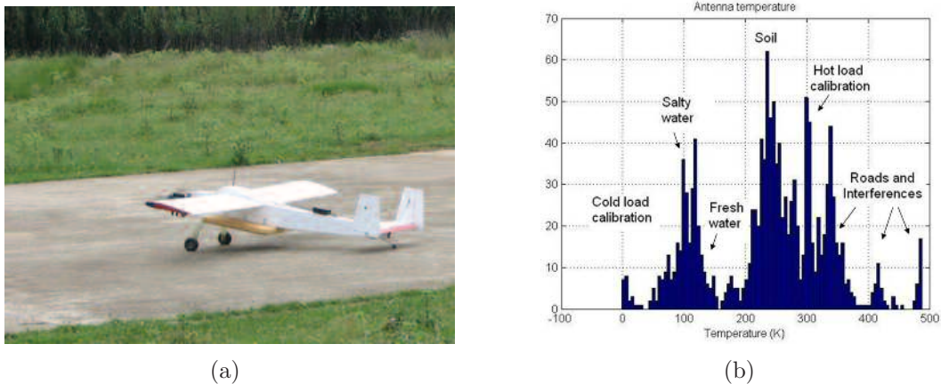
Figure 5.7 The aircraft with the ARIEL radiometer after a test flight (a). Retrieved antenna temperature histogram (b).
