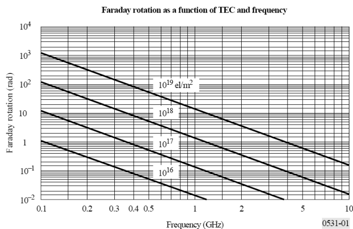
Figure 2.4 Typical values of Faraday rotation angle as a function of TEC and frequency, from ITU-R P.531-6 [2001].
