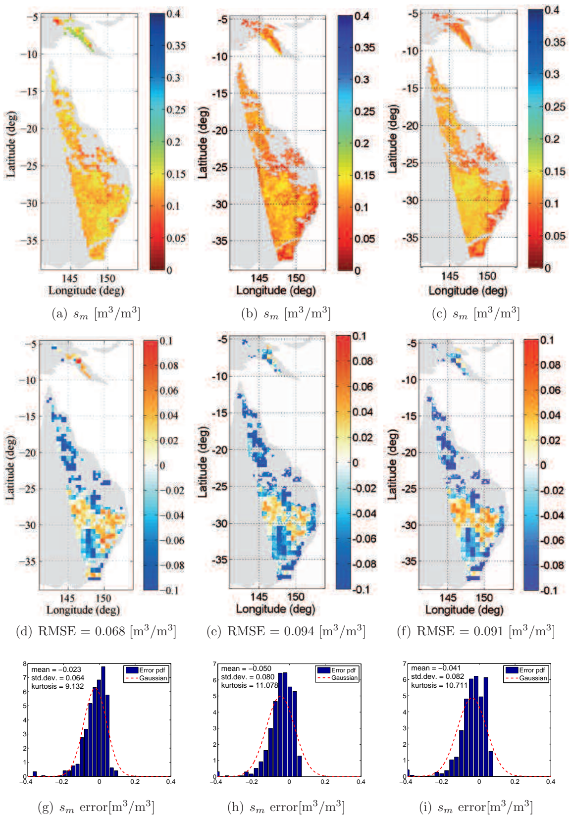
Figure A.5 As for Fig. 6.16, but using the linking model in (6.3), and an SMOS image over eastern Australia, from February 17, 2009 (6 am).
