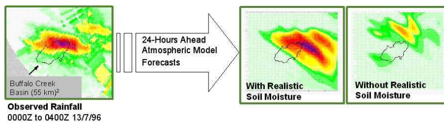
Figure 1.2 Soil moisture initialization of Numerical Weather Prediction models leading to an improved precipitation forecast (adapted from Chen et al. [2001])
