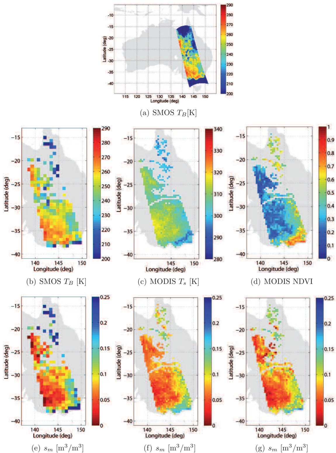
Figure 6.15 As for Fig. 6.6, but using an SMOS image covering the Murrumbidgee catchment, from February 19, 2010 (6 am).
