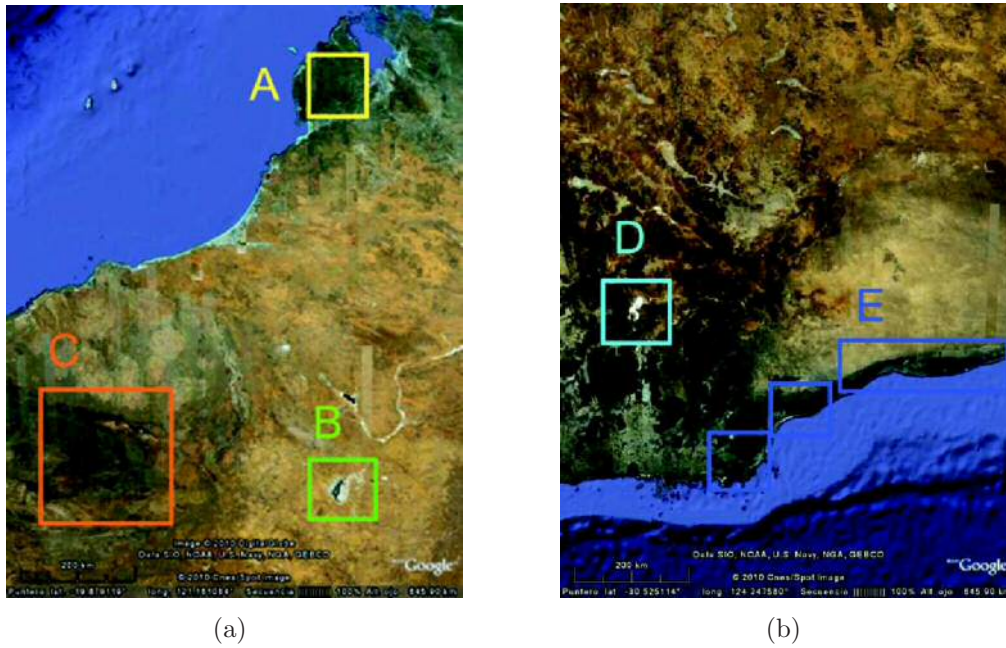
Figure 6.7 Aerial photographs covering the regions above (a) and below (b) the cloud mask in Fig. 6.6(b), from Google Earth.
