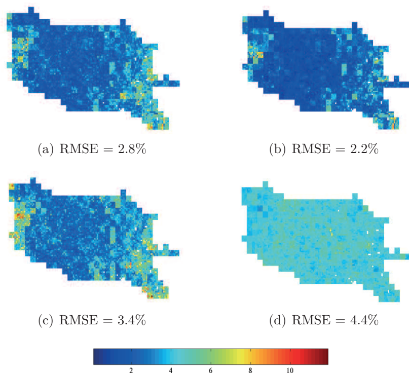
Figure 7.5 Spatial distribution of the soil moisture error retrieved using the change detection method with (a) \sigma_{hh}^0 , (b) \sigma_{vv}^0 , (c) \sigma_{hv}^0 , and (d) the radiometer only technique.
