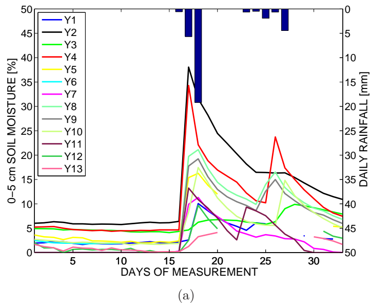
Figure 6.13 Temporal evolution of 0-5 cm continuous soil moisture measurements (6 am) and mean daily rainfall observed at 13 Yanco monitoring stations.
