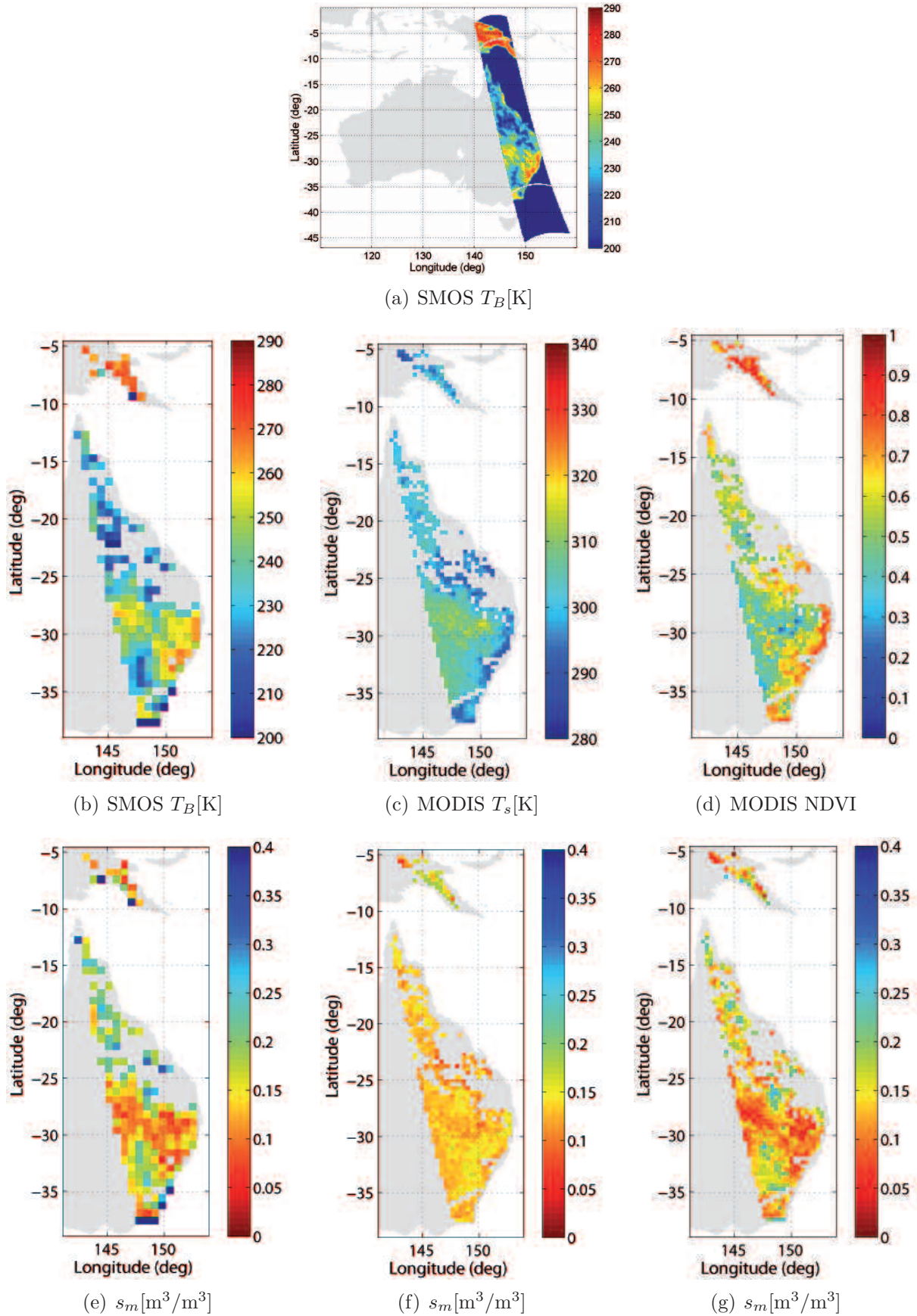
Figure 6.8 As for Fig. 6.6, but using an SMOS image over eastern Australia from February 17, 2010 (6 am).
