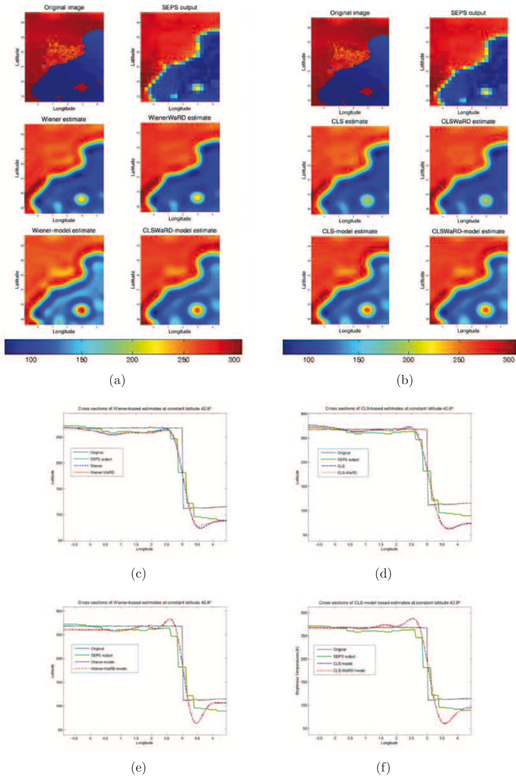
Figure 5.6 As for Fig. 5.5, except for using an SMOS simulated image covering the north-east of Spain as original.
