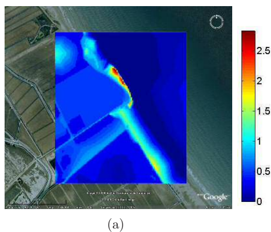
Figure 5.9 Digital Elevation Model [m] of the Marquesa beach area at 5 m spatial resolution, geo-referenced on Google Earth.
