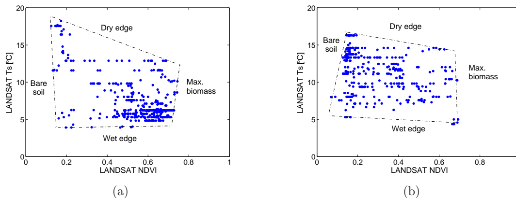
Figure 6.2 Scatter plots of LANDSAT surface radiant temperature vs. LANDSAT NDVI of the areas corresponding to (a) Flight 1, and (b) Flight 2.
