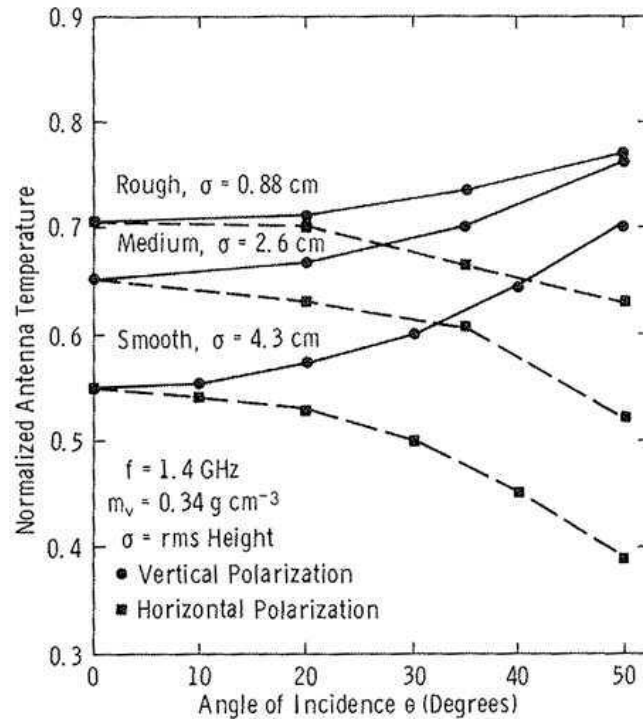
Figure 2.6 Measured normalized antenna temperature (emissivity) vs. incidence angle at 1.4 GHz for three bare soil fields with different surface roughnesses, from Newton and Rouse [1980]
