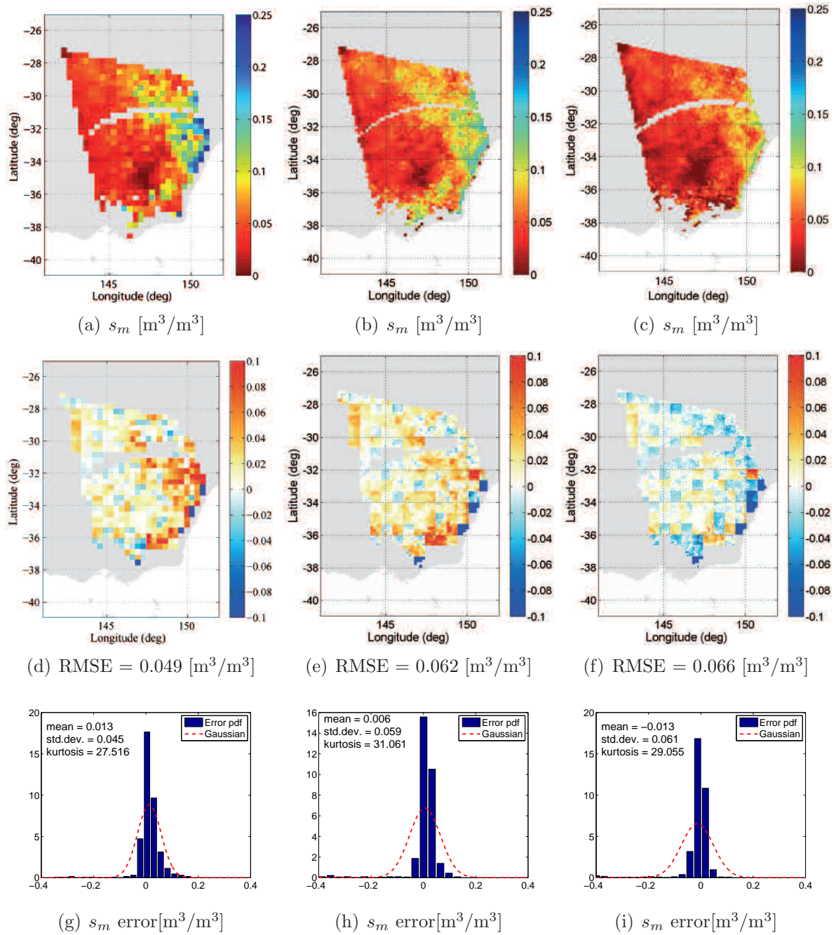
Figure 6.17 As for Fig. 6.16, but using an SMOS image over eastern Australia from January 22, 2010 (6 am).
