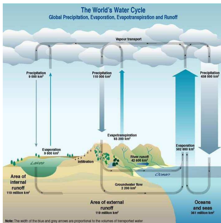
Figure 1.1 Precipitation, evaporation, evapotranspiration and runoff are the processes that move water through the water cycle. Values in the diagram show the volume of water that moves along each path in a year ( www.unep.org )
