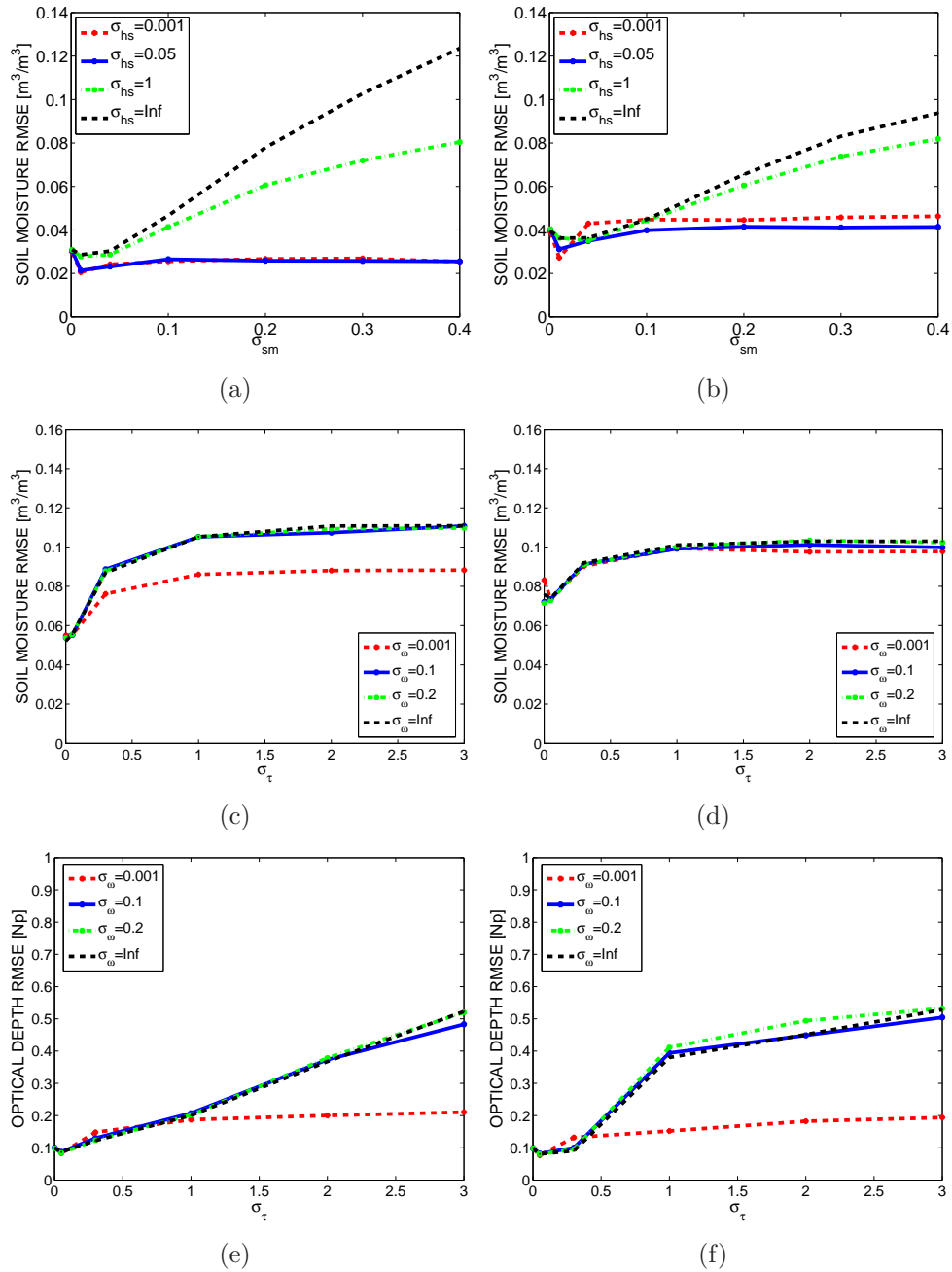
Figure 3.2 As for Fig. 3.1, except for retrievals formulated using the first Stokes parameter ( T_I ).
