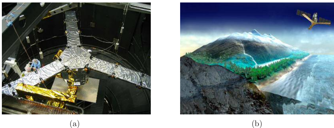
Figure 1.4 SMOS-MIRAS undergoing testing in the Large Space Simulator at ESA-ESTEC (a), and SMOS-MIRAS artist's view (b), from www.esa.int
