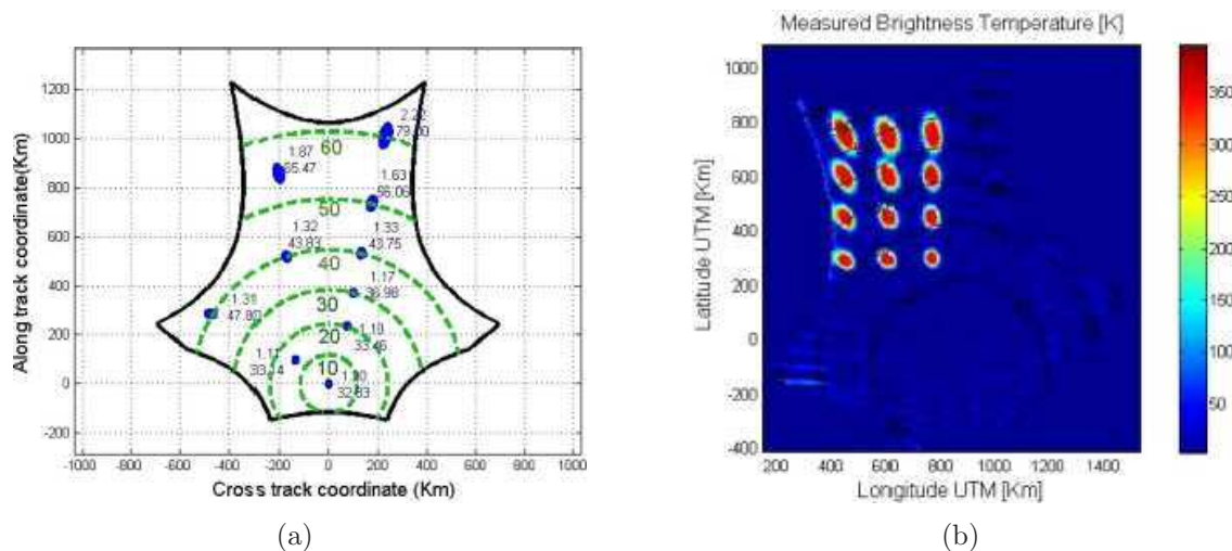
Figure 5.1 SMOS observations with varying incidence angles, pixel spatial resolutions, and axial ratios (a). Reconstructed synthetic image with point sources over the area under study processed by SEPS (b)
