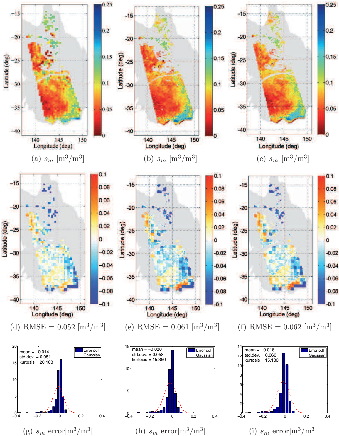
Figure A.2 As for Fig. 6.16, but using an SMOS image over eastern Australia from February 19, 2010 (6 am).
