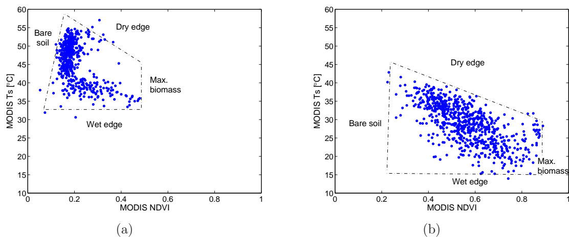
Figure 6.9 Scatter plots of MODIS surface radiant temperature vs. MODIS NDVI, from (a) Fig. 6.6, and (b) Fig. 6.8.
