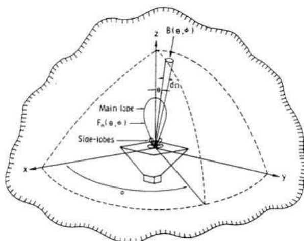
Figure 2.1 Geometry of the incident radiation from an extended source on an antenna, from Ulabiy et al. [1981]
