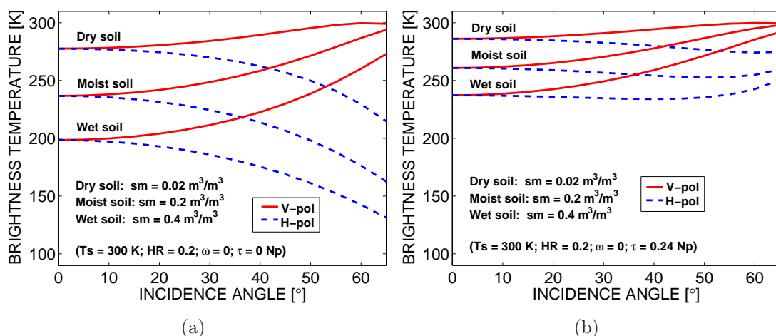
Figure 2.7 Plots illustrating the brightness temperature dependence with incidence angle of (a) bare, and (b) vegetation-covered dry, moist and wet soils, from (2.32) (from Piles et al. [2010]).
