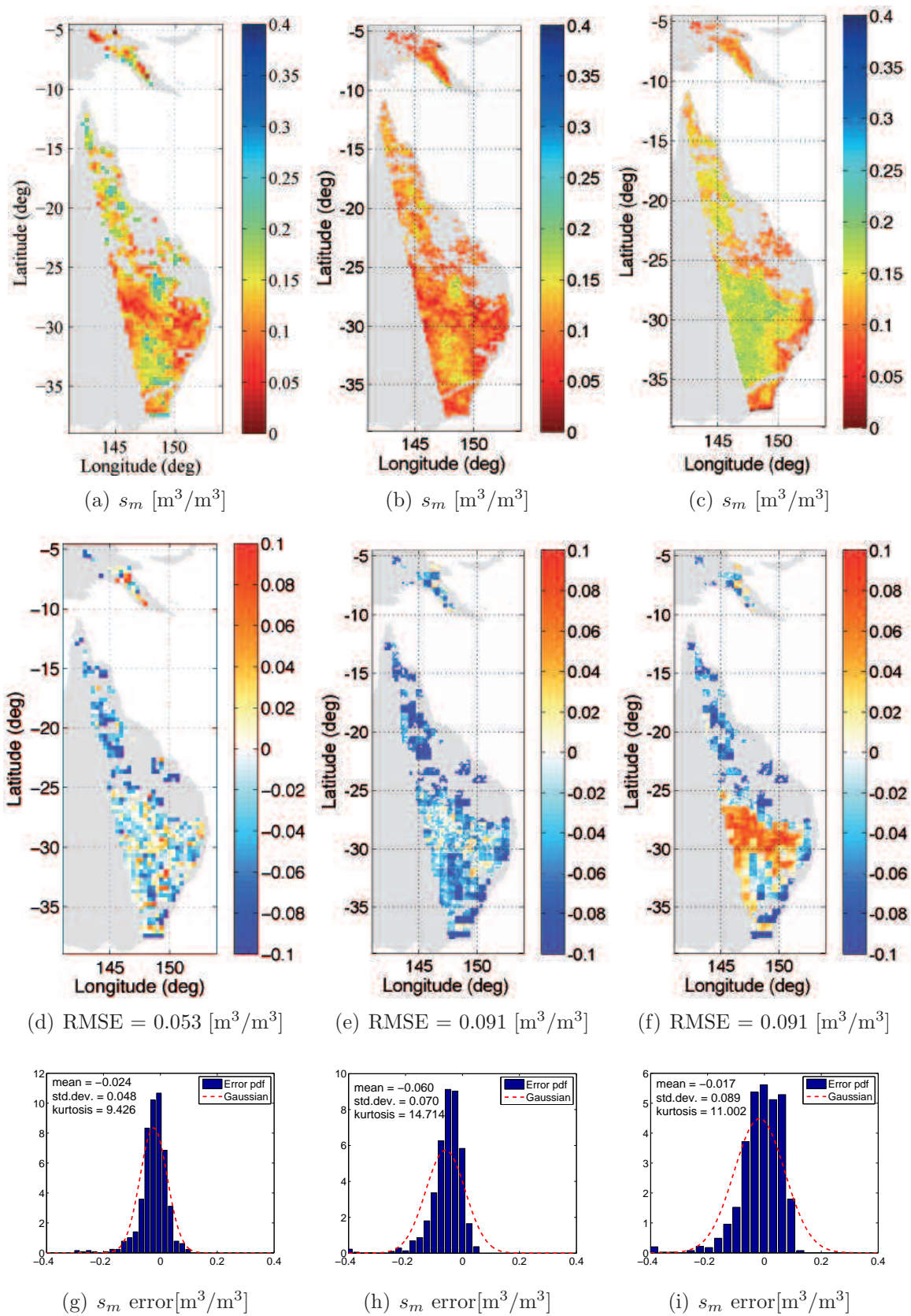
Figure A.1 As for Fig 6.16, but using an SMOS image over eastern Australia from February 17, 2010 (6 am).
