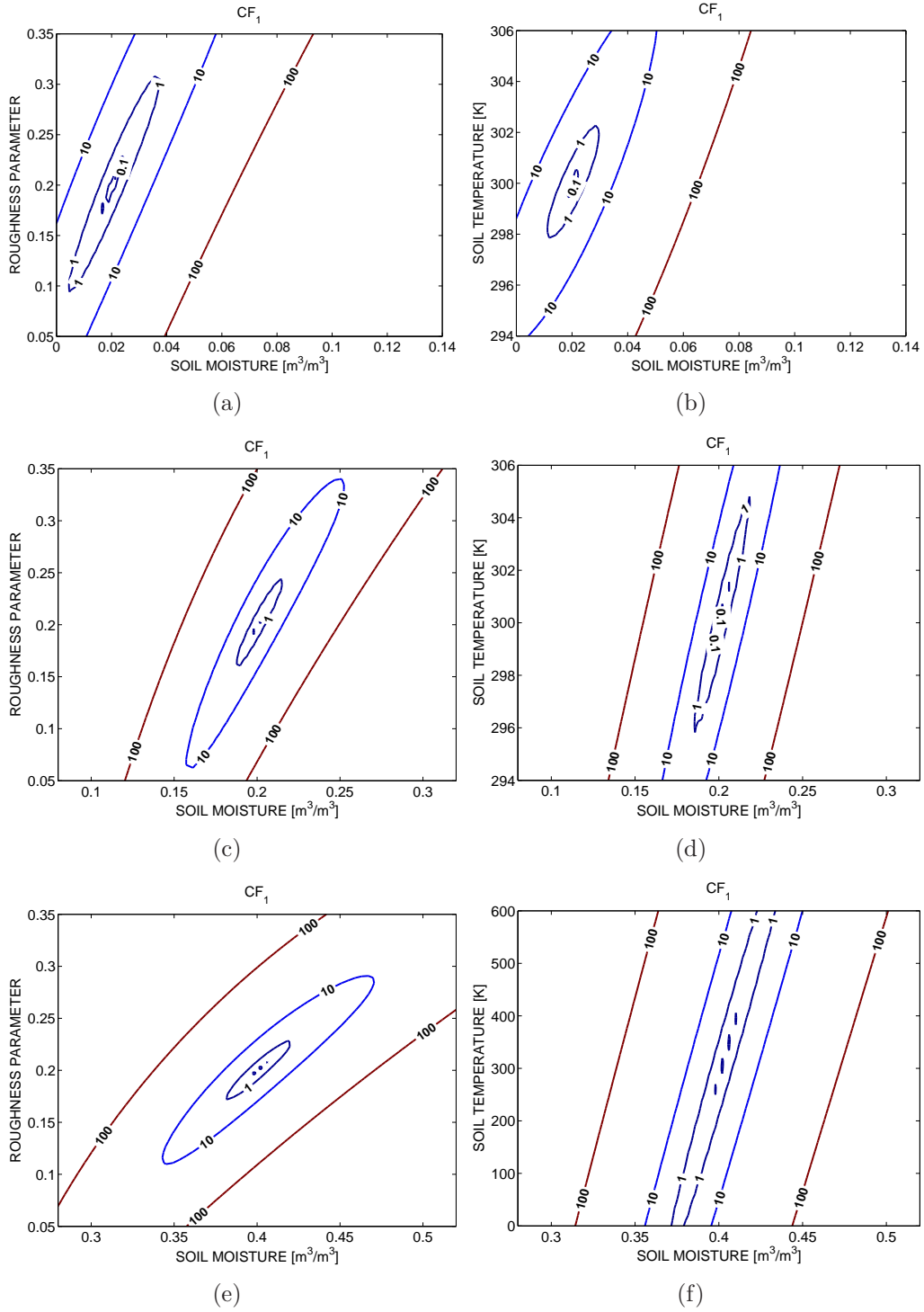
Figure 4.3 Cost functions formulated using T_{vv} - T_{hh} with no constraints. Contours of h_s vs. s_m (a) and T_s vs. s_m (b) over a bare dry soil scenario. Contours of h_s vs. s_m (c) and T_s vs. s_m (d) over a bare moist soil scenario. Contours of h_s vs. s_m (e) and T_s vs. s_m (f) over a bare wet soil scenario.
