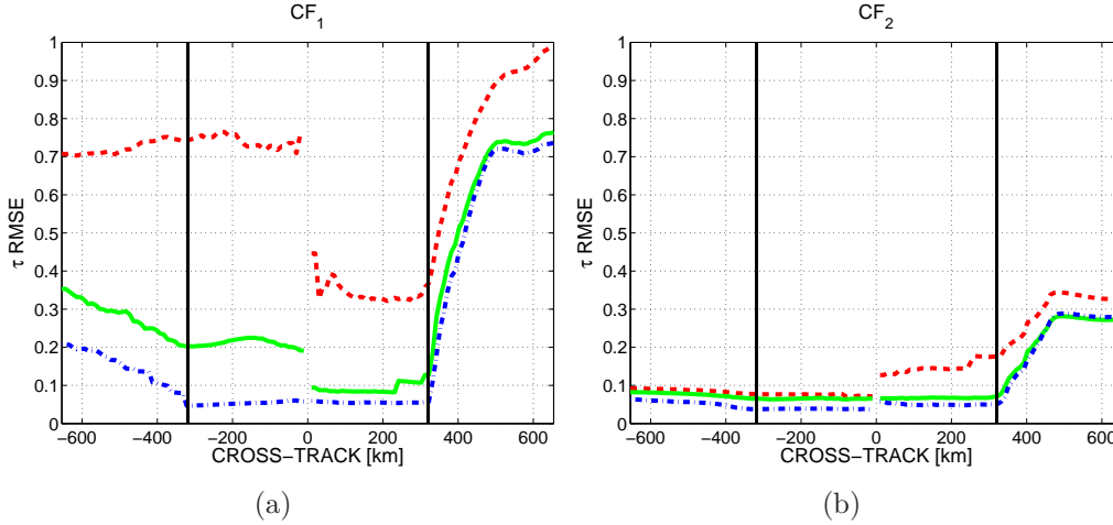
Figure 4.6 Retrieved vegetation optical depth RMSE of simulated SMOS observations versus pixel position in the swath; Simulations over the vegetation-covered dry (red, dashed lines), moist (green, solid lines), and wet (blue, dashed-dotted lines) scenarios of Table 4.1, (a) with no constraints on the cost-function ( CF_1 ), and (b) adding constraints on all parameters, except s_m ( CF_2 ). In each plot: first Stokes parameter (left side) and Earth's reference frame (right side). Vertical lines denote the Narrow Swath.
