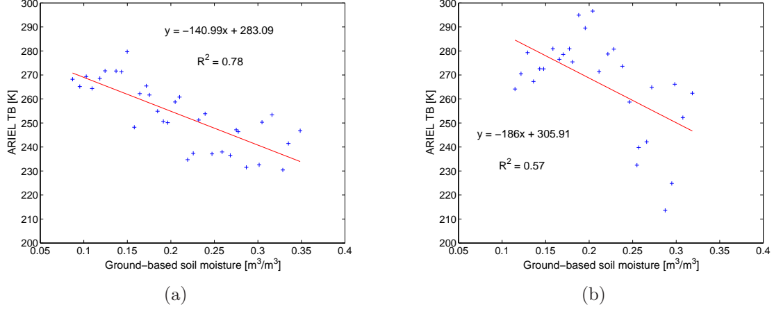
Figure 6.3 Linear regression between ARIEL T_B and coincident ground measurements of 0-5 cm soil moisture acquired during (a) Flight 1, and (b) Flight 2.
