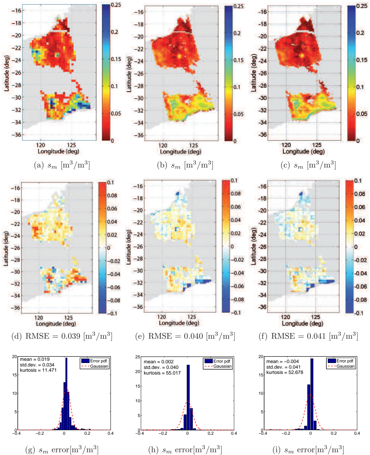
Figure 6.16 SMOS-derived soil moisture maps and error statistics at 32, 16, and 8 km spatial resolution over western Australia, from December 8, 2009 (6 am), using the linking model in (6.9). SMOS-derived soil moisture maps [ \text{m}^3/\text{m}^3 ] at (a) 32 km, (b) 16 km, and (c) 8 km spatial resolutions. Spatial distribution of the soil moisture error [ \text{m}^3/\text{m}^3 ] between soil moisture retrievals at (d) 32 km, (e) 16 km, and (f) 8 km, and soil moisture retrievals at 64 km. Empty areas in the images correspond to clouds masking MODIS T_s measurements. Normalized pdf and statistics of the difference between soil moisture retrievals at (g) 32 km, (h) 16 km, and (i) 8 km, and soil moisture retrievals at 64 km. The red dashed line is the normal distribution pdf with the same mean value and standard deviation.
