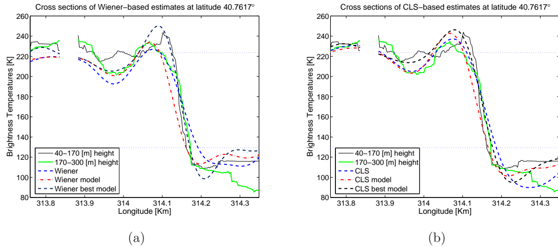
Figure 5.10 Cross-sections of the image obtained from ARIEL observations at heights 40-170 m, 170-300 m, and of the images resulting from (a) the application of Wiener-derived filters to the 170-300 m height image, and (b) the application of CLS-derived filters to the 170-300 m height image.
