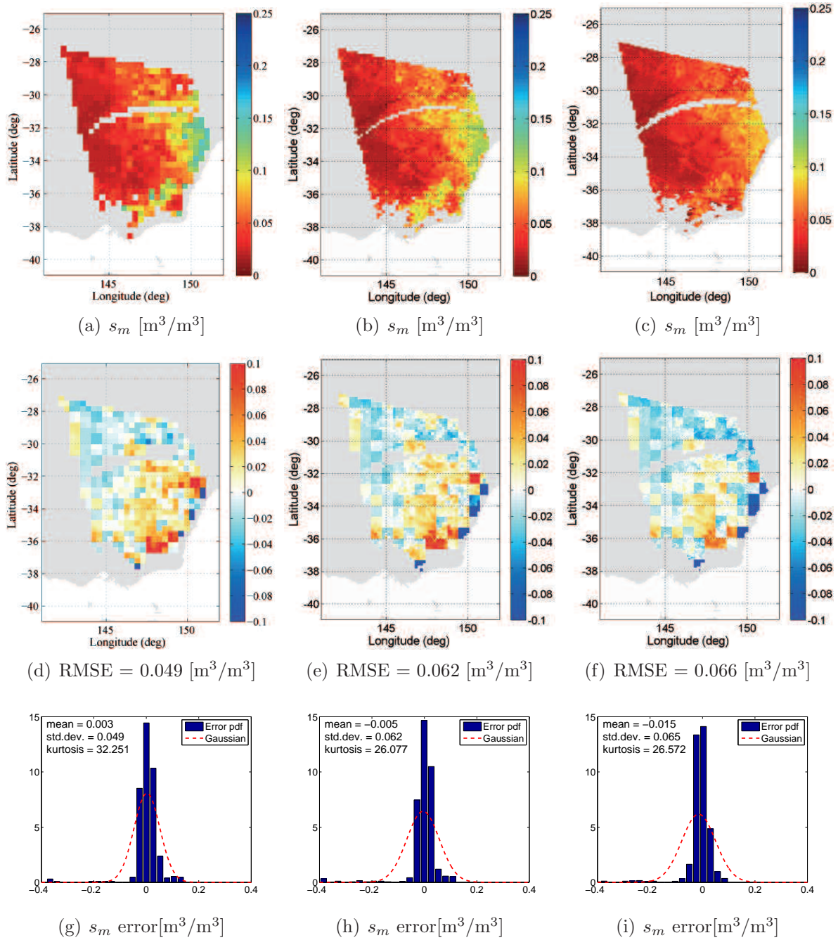
Figure A.4 As for Fig. 6.16, but using the linking model in (6.3), and an SMOS image over eastern Australia from January 22, 2010 (6 am).
