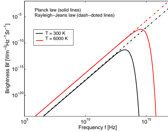
Figure 2.2 Comparison of Planck radiation law with its low-frequency approximation (Rayleigh-Jeans law) for T=300 K and T=6000 K.
