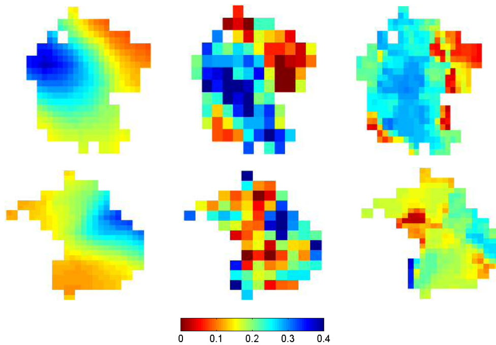
Figure 6.4 Sample results for the visual comparison of soil moisture fields [ \text{m}^3/\text{m}^3 ]. From left to right: interpolated ground-based soil moisture, soil moisture retrieved from ARIEL T_B , and downscaled soil moisture obtained with the algorithm presented. Upper row: Flight 1; Lower row: Flight 2.
