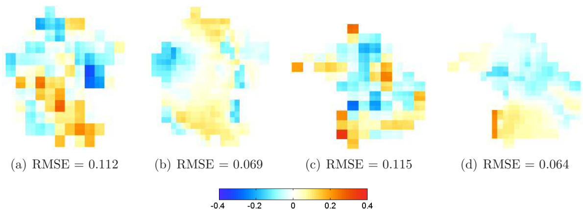
Figure 6.5 Spatial distribution of the soil moisture error [ \text{m}^3/\text{m}^3 ] between the interpolated ground-based soil moisture map and the retrieved one, using ARIEL T_B on (a) Flight 1 and (c) Flight 2, and obtained with the downscaling algorithm on (b) Flight 1 and (d) Flight 2 observations
