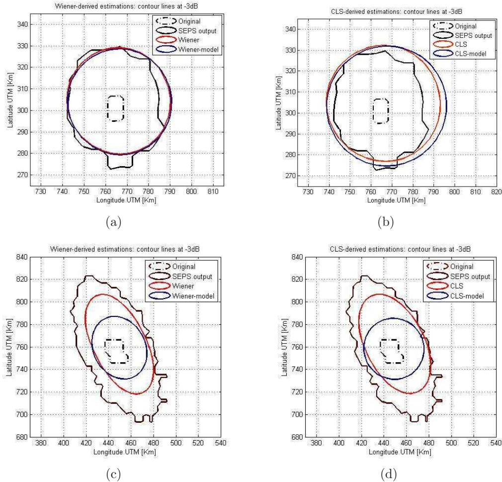
Figure 5.2 Best case pixel's contour at -3 dB after applying (a) Wiener-derived methods and (b) CLS-derived methods to Fig. 5.1(b). Worst case pixel's contour at -3 dB after applying (c) Wiener-derived methods and (d) CLS-derived methods to Fig. 5.1(b).
