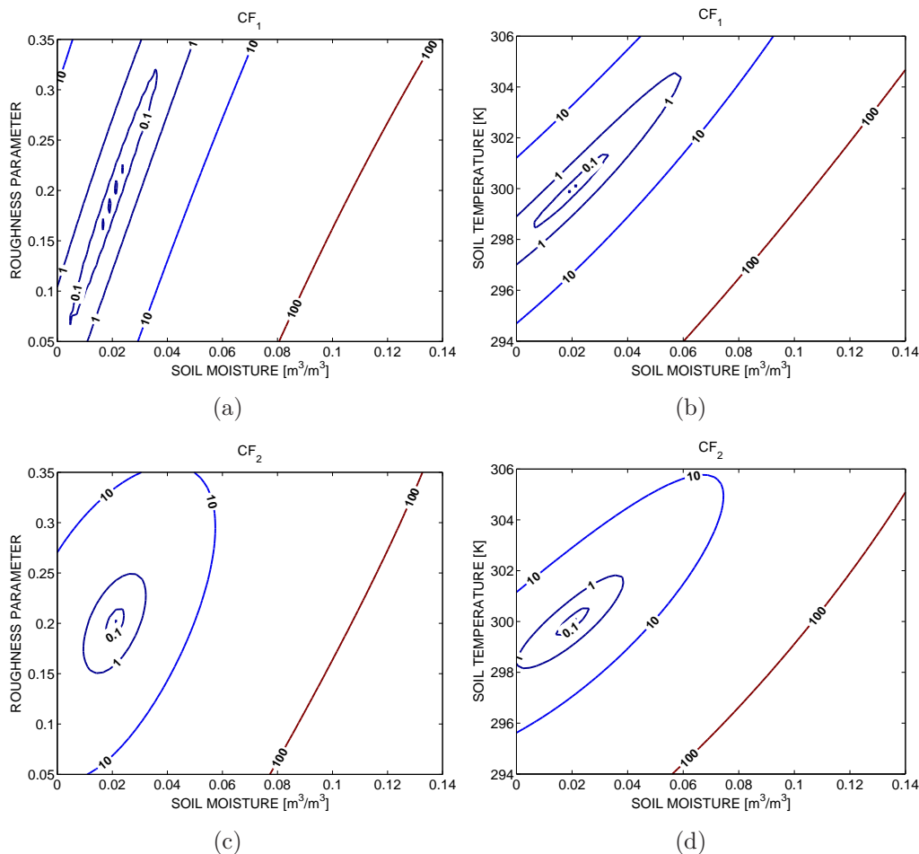
Figure 4.2 Cost functions formulated using T_I over a vegetation-covered dry soil scenario. Contours of h_s vs. s_m (a) and T_s vs. s_m (b), with no constraints on the cost function ( CF_1 ). Contours of h_s vs. s_m (c) and T_s vs. s_m (d), adding constraints on all parameters, except for s_m ( CF_2 ).
