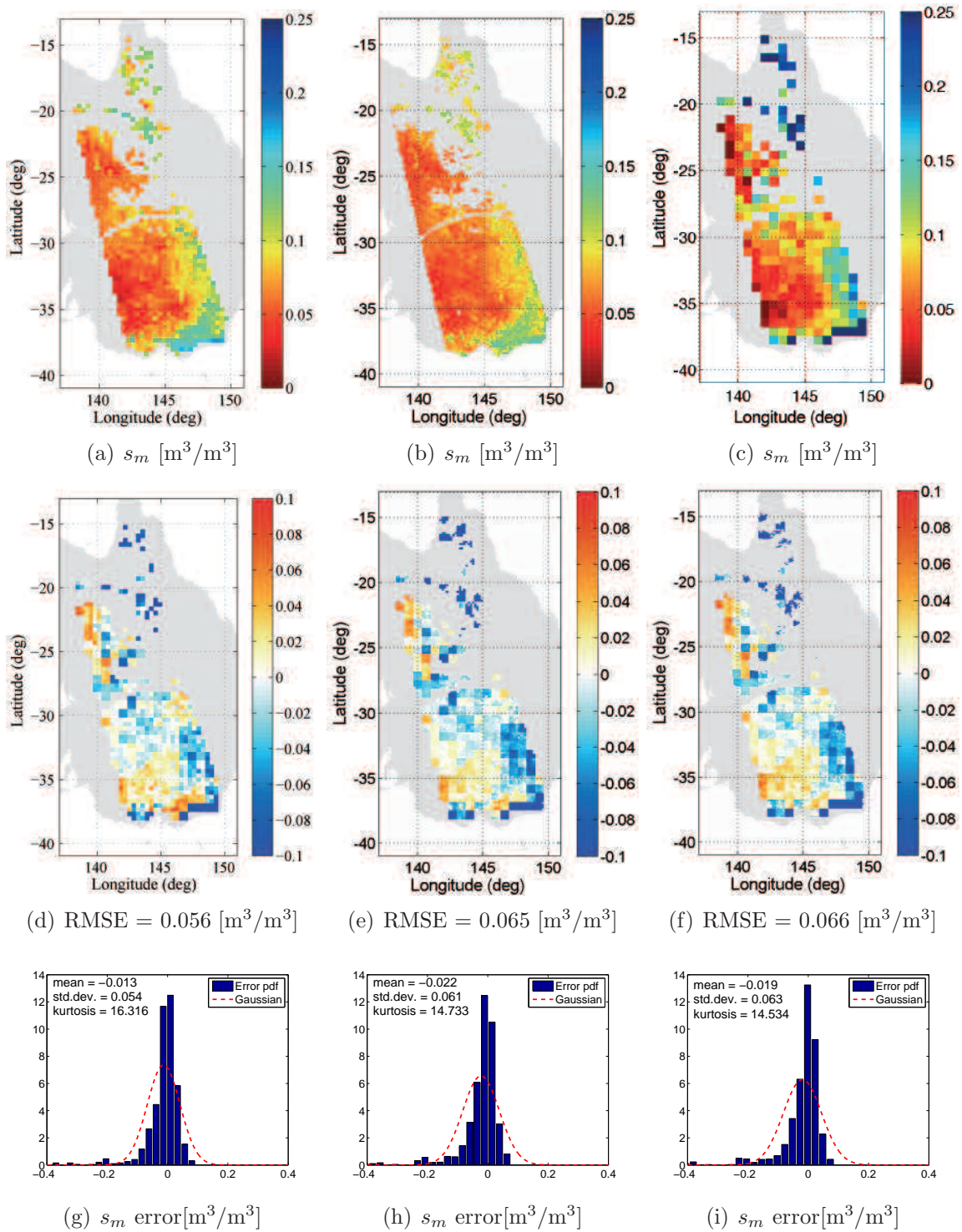
Figure A.6 As for Fig. 6.16, but using the linking model in (6.3), and an SMOS image over eastern Australia, from February 19, 2010 (6 am).
