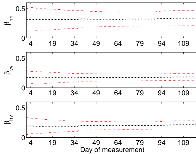
Figure 7.8 Plots of the mean slope (in black) and mean slope \pm the daily slope standard deviation (in red) for vv , hh and hv polarizations, for each day of the 4-month OSSE dataset.
