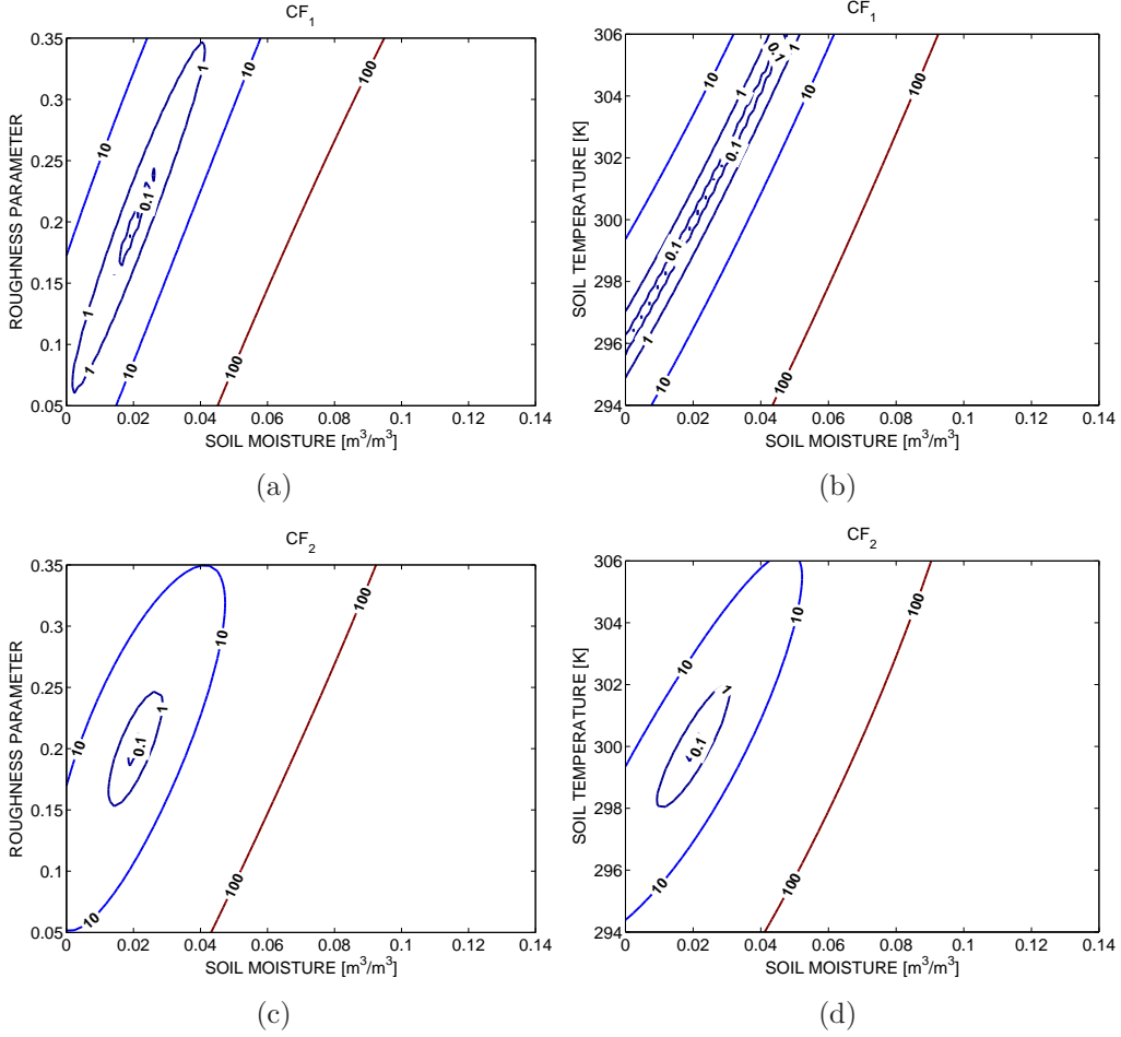
Figure 4.1 Cost functions formulated using T_I over a bare dry soil scenario. Contours of h_s vs. s_m (a) and T_s vs. s_m (b), with no constraints on the cost function ( CF_1 ). Contours of h_s vs. s_m (c) and T_s vs. s_m (d), adding constraints on all parameters, except for s_m ( CF_2 ).
