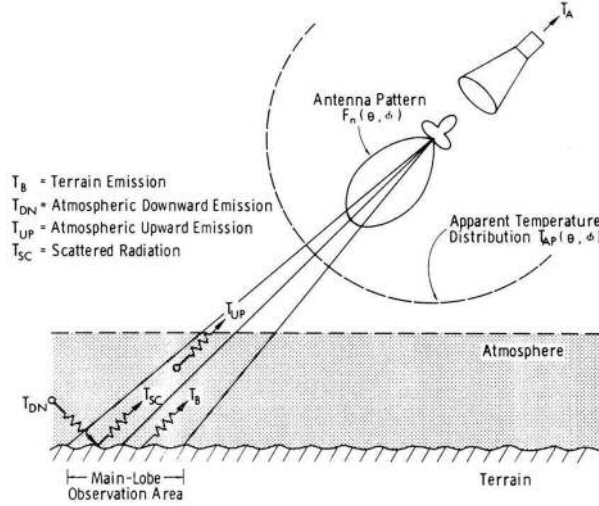
Figure 2.3 Radiation incident upon an Earth-looking radiometer. Relationships between the antenna temperature T_A , apparent temperature T_{AP} , and brightness temperature T_B , from Ulaby et al. [1981]
