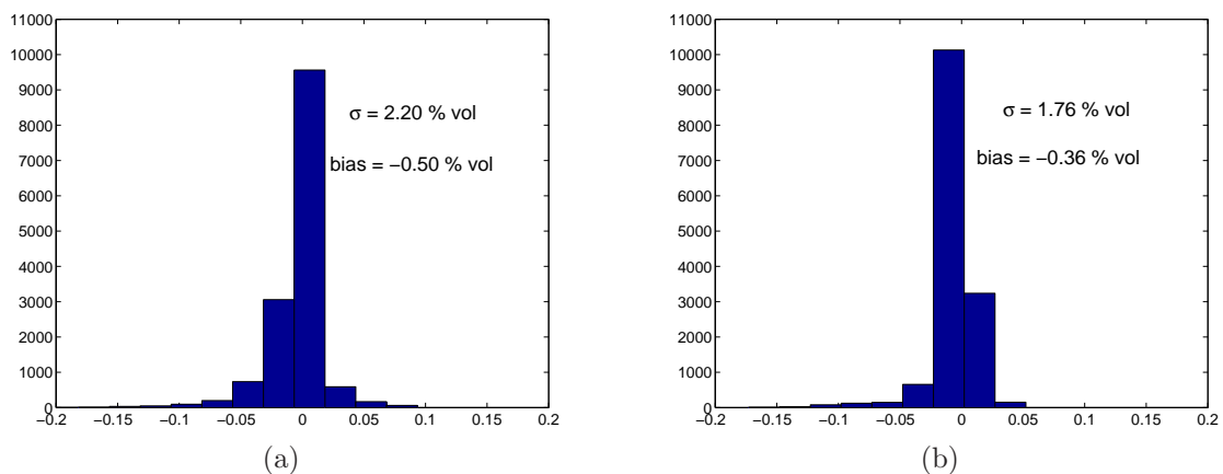
Figure 7.3 Histogram of the difference between soil moisture retrieved using static map of \beta of 400 m and using static map of \beta at 1600 m for (a) hh and (b) vv polarizations.
