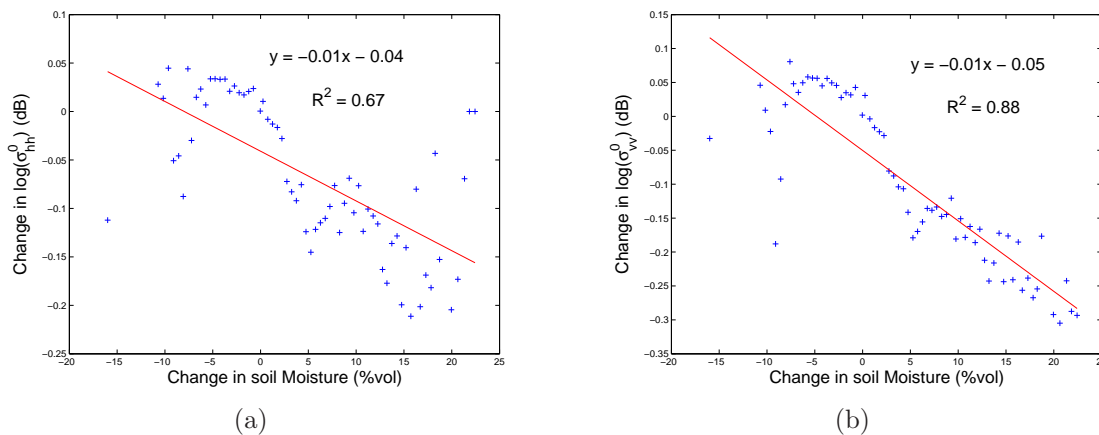
Figure 7.1 Change in log of PALS observed L-band radar backscatter at (a) hh and (b) vv polarizations plotted versus change in in situ volumetric soil moisture in the 0 to 6 cm soil layer for the period June 25 to June 27 and July 5 to July 7. The change in radar backscatter has been stratified by 0.05% change in volumetric soil moisture.
