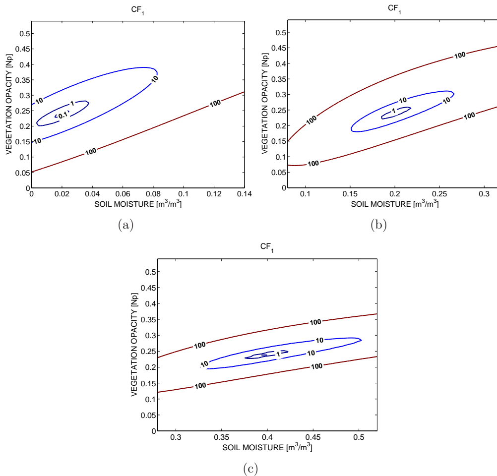
Figure 4.4 Cost functions formulated using T_{vv} - T_{hh} with no constraints. Contours of \tau vs. s_m (a) over a vegetation-covered dry scenario. Contours of \tau vs. s_m (b) over a vegetation-covered moist scenario. Contours of \tau vs. s_m (c) over a vegetation-covered wet scenario.
