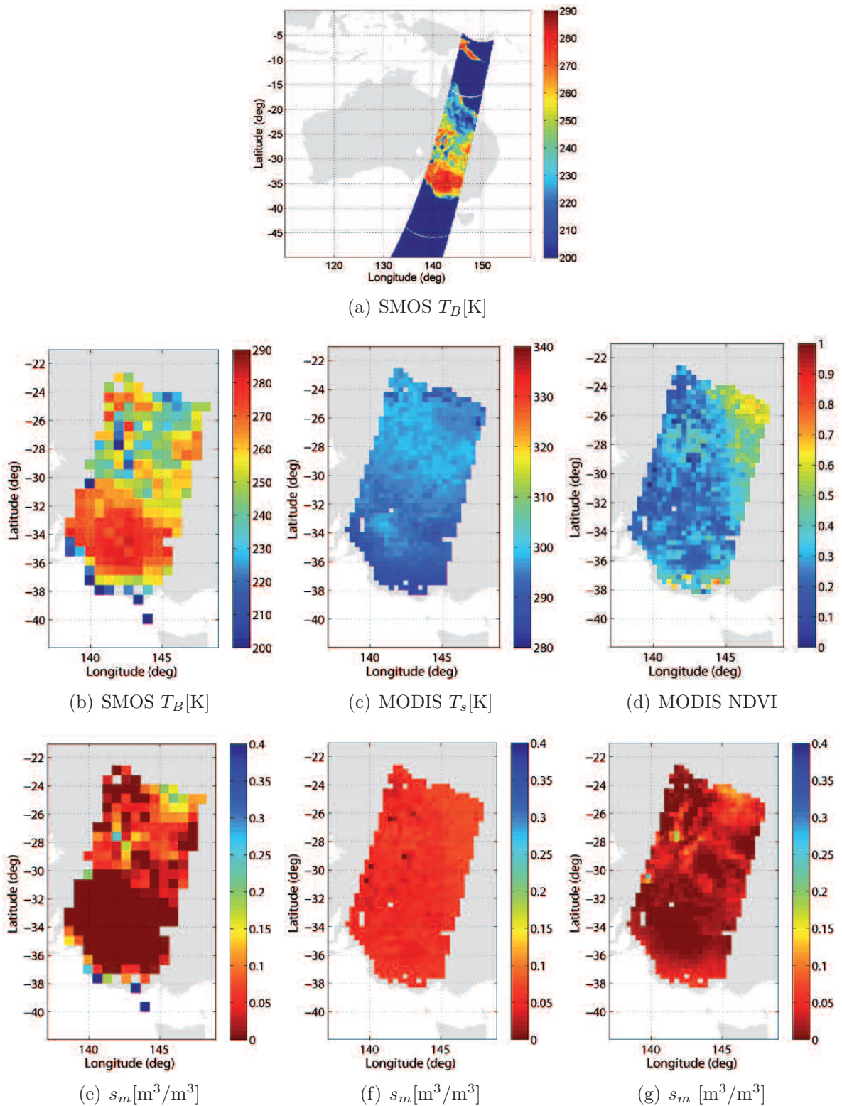
Figure 6.11 As for Fig. 6.6, but using an SMOS image over south-eastern Australia, from February 17, 2010 (6 pm).
