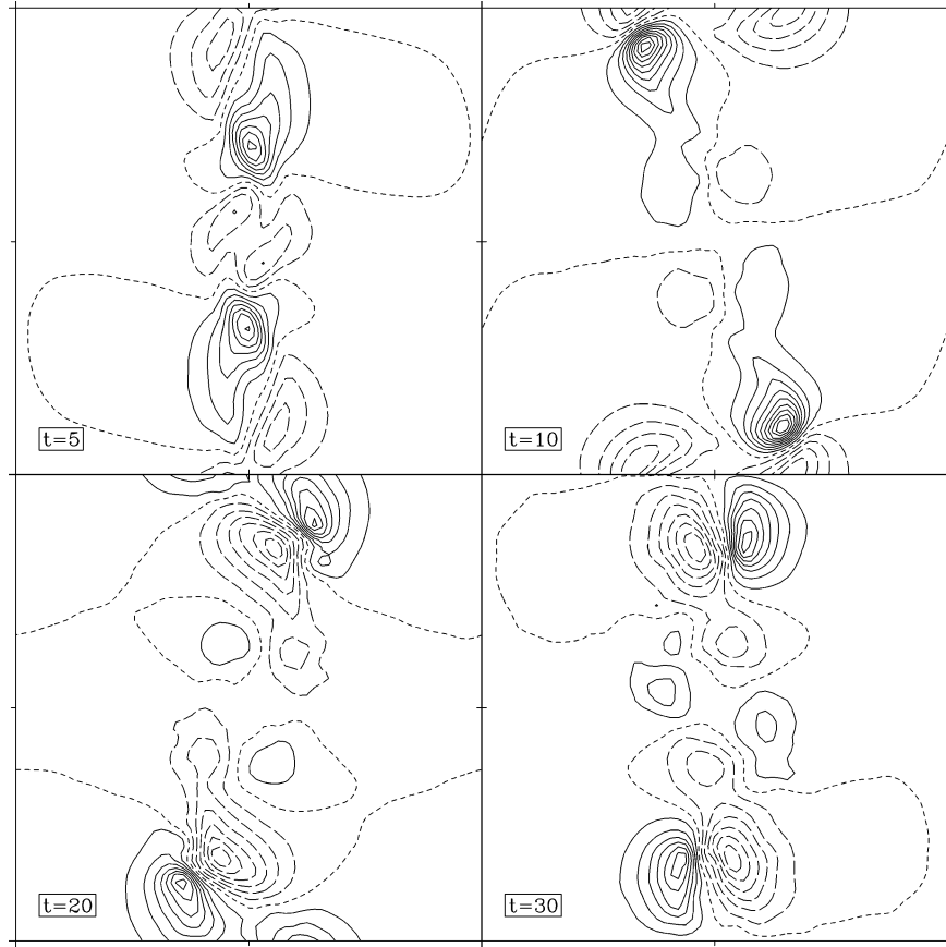
FIG. 3. As in Fig. 2 but for the QG vertical velocity w^q .
