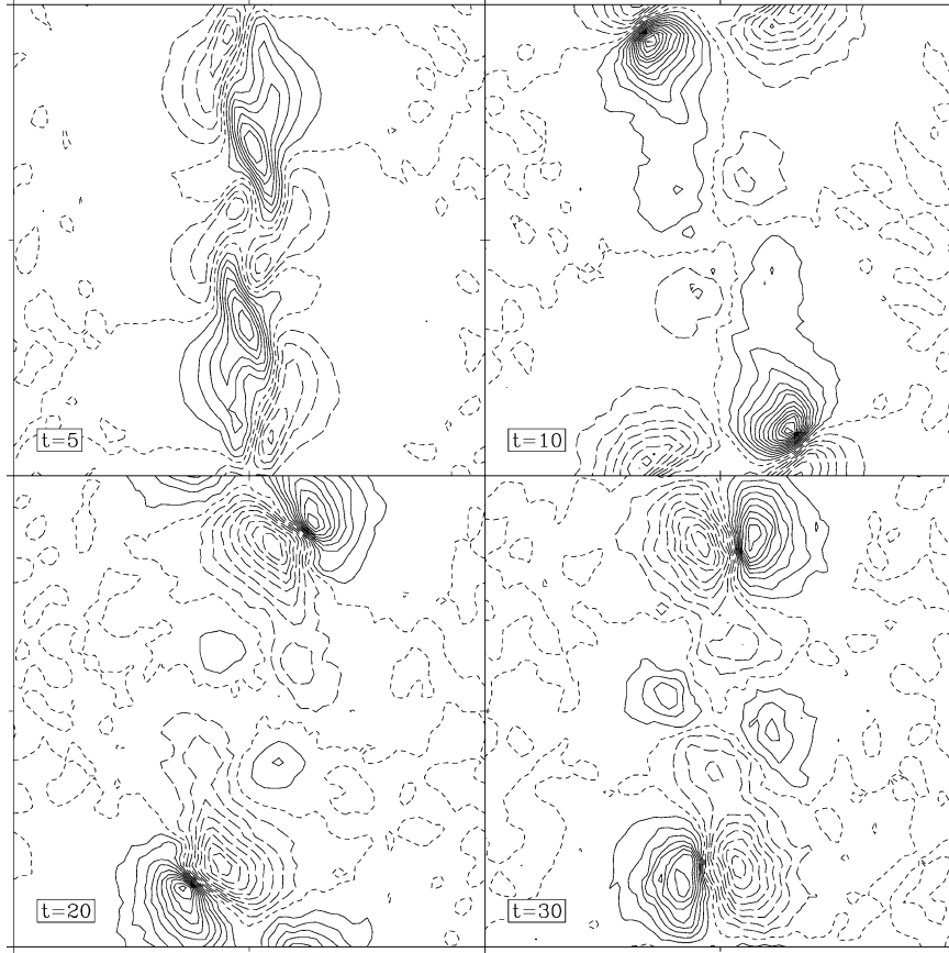
FIG. 2. Time evolution of the vertical velocity w in the horizontal layer l_z = 28 for the case \varpi_0 = -0.75 and e_f = 10 . Times are indicated in inertial periods. Contour interval \Delta is 2.5 \times 10^{-5} .
