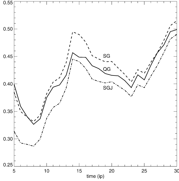
FIG. 23. Time series, for the jet current case with \varpi_0 = \pm 0.75 and e_f = 10 , of the relative spatial averages \langle |w - w^q| \rangle / \langle |w| \rangle (symbol QG), \langle |w - w^s| \rangle / \langle |w| \rangle (symbol SG), and \langle |w - w^{sJ}| \rangle / \langle |w| \rangle (SGJ, where w^{sJ} is obtained by solving the SG \omega equation including the term -J'_z ).
