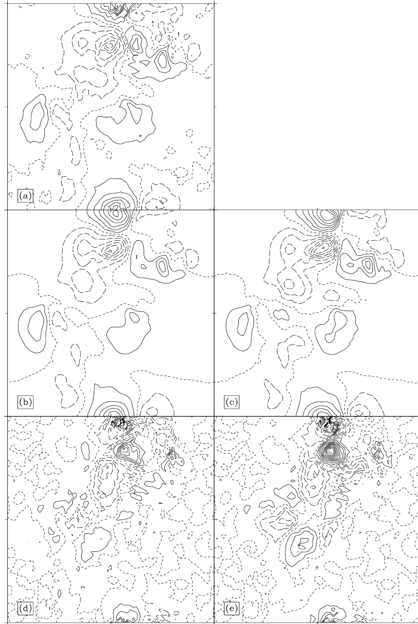
FIG. 21. Horizontal distributions of (a) w ( \Delta = 5 \times 10^{-5} ), (b) w^q ( \Delta = 5 \times 10^{-5} ), (c) w^s ( \Delta = 5 \times 10^{-5} ), (d) w - w^q ( \Delta = 2.5 \times 10^{-5} ), and (e) w - w^s ( \Delta = 2.5 \times 10^{-5} ), for the jet current at t = 20 t_{ip} and horizontal layer l_z = 28 .
