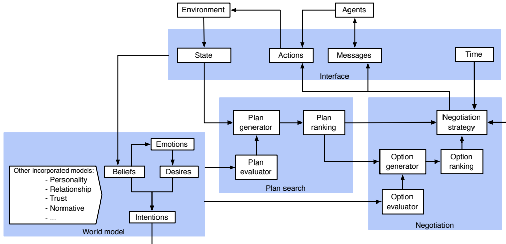
Figure 3: Graphical representation of HANA. Arrows represent data flows. Coloured boxes represent the modules that form part of the agent, and white boxes are components of those modules.
