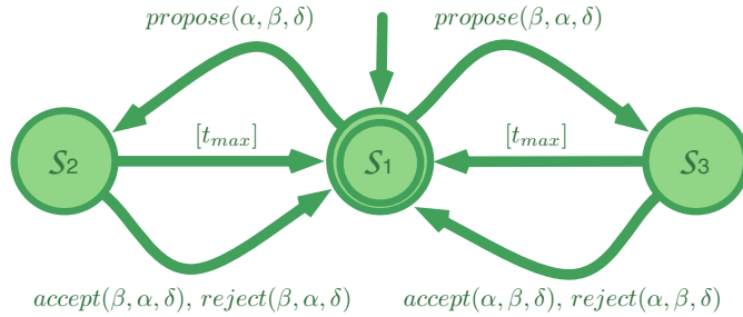
Figure 1: Negotiation protocol. Proposals are replied by accepts and rejects. It is not possible to send a proposal when a previous one is not yet replied. [t_{max}] represents the end of the negotiation round.
