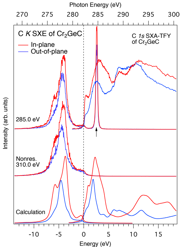
FIG. 3: (Color online) Top-right: C 1s XAS-TFY spectra of Cr 2 GeC. Left top-to-bottom: resonant spectra excited at 285.0 (indicated by the upward arrow) and nonresonant C K XES spectra at 310.0 eV. All spectra are plotted on a photon energy scale (top) and a relative energy scale (bottom) with respect to the top of the valence band.
