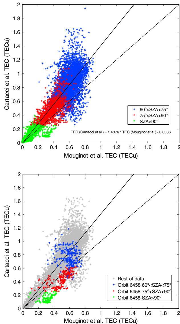
Figure 4. (top) TEC (Cartacci et al.) versus TEC (Mouginito et al.). Data have been split into three different solar zenith angle intervals: dayside in blue ( 60^\circ < \chi < 75^\circ ), dayside/terminator in red ( 75^\circ < \chi < 90^\circ ), and nightside in green ( \chi > 90^\circ ). The dashed black line shows the 1:1 dependence, while the solid black line represents a ratio of 1.4076 between the two data sets. (bottom) Same figure than before but only with the orbit 6458 shown in colors, while the rest of data (data from 18 orbits) is plotted in grey in the background. TEC is always represented in TECu.
