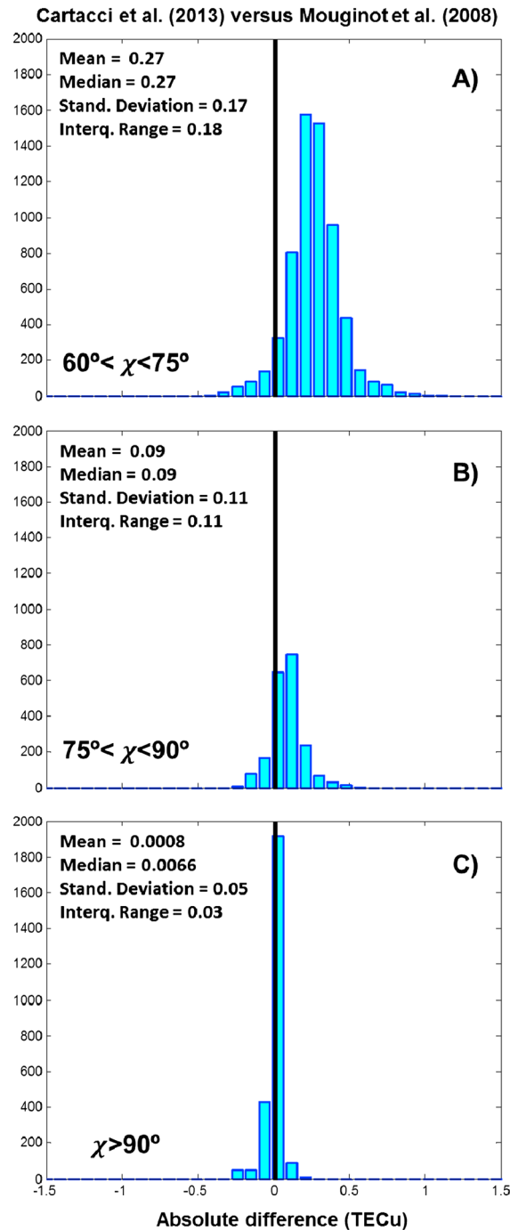
Figure 3. Absolute differences of the 19 selected orbits between Cartacci et al. and Mougnot et al.'s data for three different solar zenith angle intervals: (a) dayside ( 60^\circ < \chi < 75^\circ ) (top, amount of data 6232), (b) dayside/terminator ( 75^\circ < \chi < 90^\circ ) (medium, amount of data 2003), and (c) nightside ( \chi > 90^\circ ) (bottom, amount of data 2538). The vertical black line marks the zero difference, and the units are in TECu. During nightside and close to the terminator when the disturbing effect of ionosphere is not substantial, both methods agree well. The discrepancy rises on the dayside, where the ionospheric distortion in the electromagnetic signals is evident.
