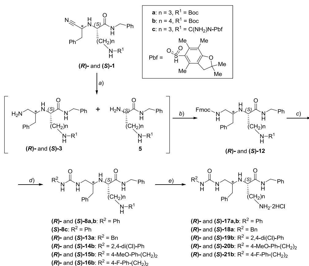
Scheme 2. Reagents and conditions: (a) NH 2 NH 2 ·H 2 O, Raney Ni, MeOH, 65 °C. (b) Fmoc-Cl, propylene oxide, CH 3 CN, 0°C. (c) Et 2 NH, CH 2 Cl 2 , rt. (d) R 2 NCO, CH 2 Cl 2 , 0°C. (e) 3M HCl, EtOAc, rt.
