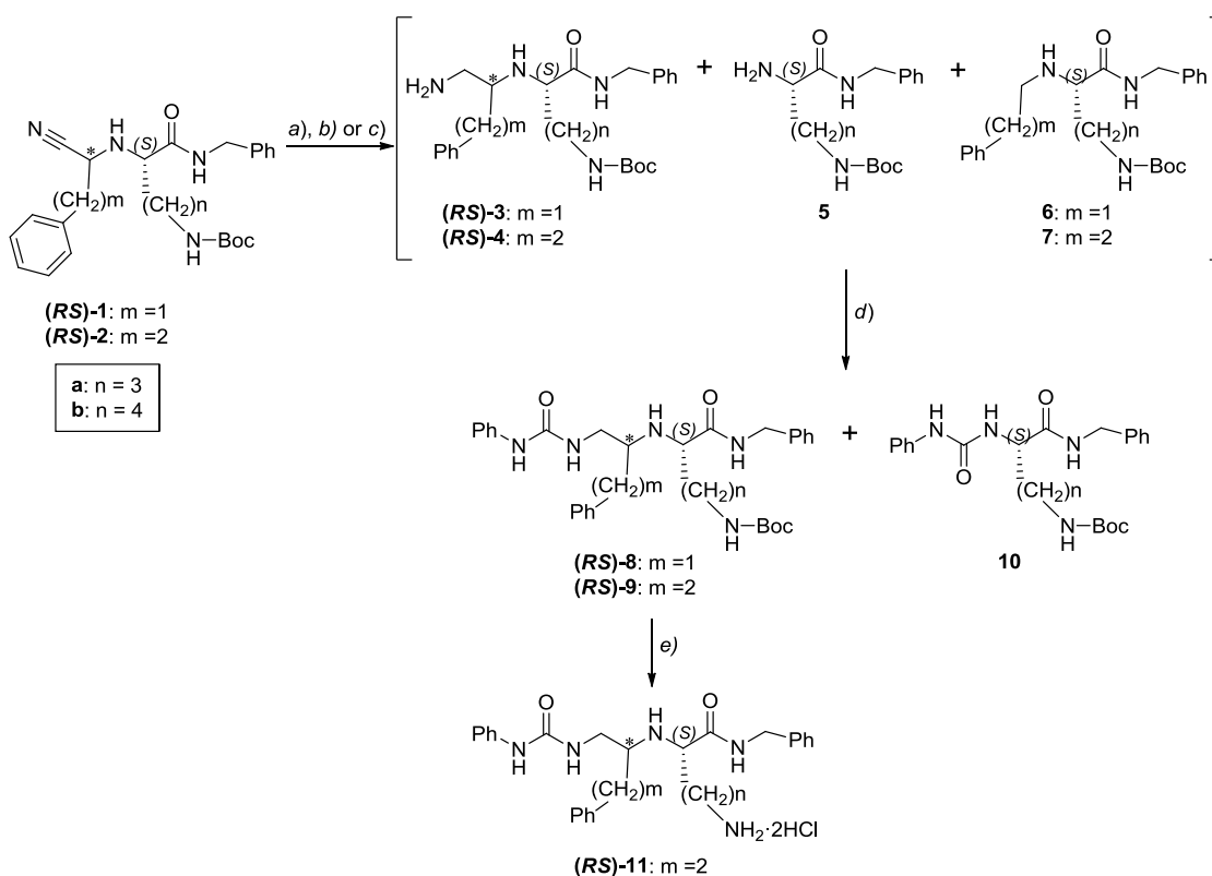
Scheme 1. Reagents and conditions: (a) \text{H}_2 , Pd(C), MeOH, rt. (b) \text{H}_2 , Raney Ni, MeOH, rt. (c) \text{NH}_2\text{NH}_2 \cdot \text{H}_2\text{O} , Raney Ni, MeOH or EtOH, T and time as indicated in Table 1. (d) PhNCO, \text{CH}_2\text{Cl}_2 , 0^\circ\text{C} . (e) 3M HCl, EtOAc, rt.
