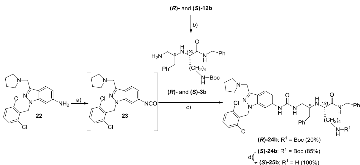
Scheme 3. Reagents and conditions: (a) (\text{CCl}_3\text{O})_2\text{CO} , propylene oxide, THF, 0 °C . (b) \text{Et}_2\text{NH} , \text{CH}_2\text{Cl}_2 , rt. (c) THF, 0 °C. (d) 3M HCl, EtOAc, rt.
