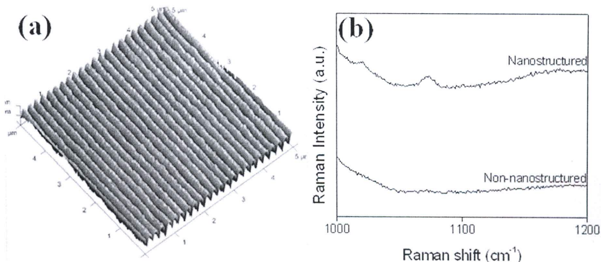
Figure 1: (a) Gold coated polymer grating. (b) Raman spectrum of a drop of BT diluted to a concentration of 10^{-3} M and dried in air on a gold coated polymer film and on a gold coated polymer grating nanofabricated by NIL.
