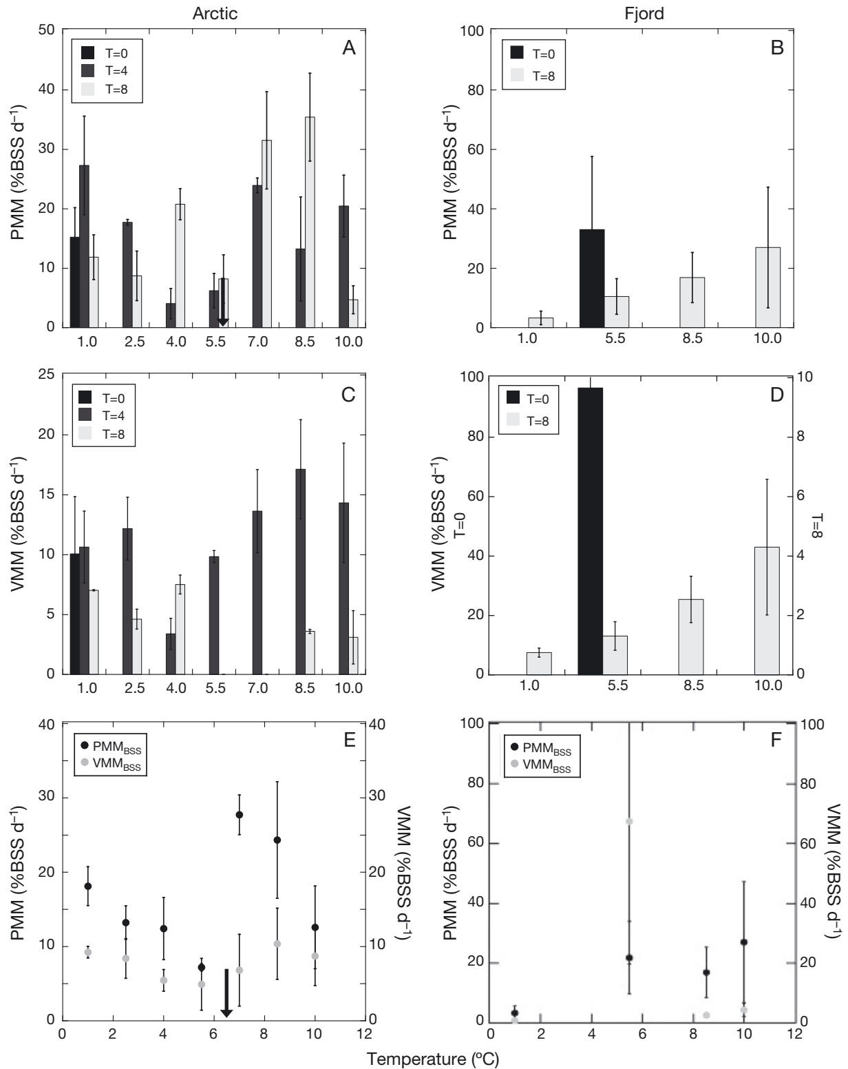
Fig. 6. Average of duplicates of virus-mediated mortality in bacteria as a percentage of the bacterial standing stock (BSS) for each temperature treatment: (A) protist-mediated mortality (PMM BSS ) in Arctic microcosms at Days 0, 4 and 8; (B) PMM BSS in Fjord microcosms at Days 0 and 8; (C) virus-mediated mortality (VMM BSS ) in Arctic microcosms; (D) VMM BSS in Fjord microcosms. Average values (±SE) of PMM BSS and VMM BSS in (E) Arctic and (F) Fjord microcosms for each temperature treatment. Arrows indicate the temperatures at which shifts in bacterial mortality occurred
