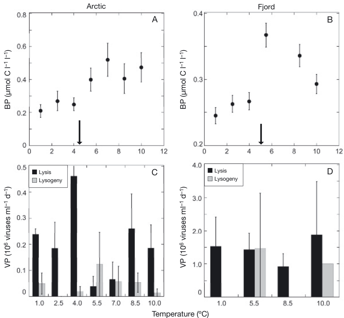
Fig. 5. Average values ( \pm SE) over the experimental period of (A,B) bacterial production (BP) for each temperature treatment in Arctic and Fjord microcosms, and average of duplicate subsamples of lytic and lysogenic viral production (VP) for each temperature treatment in (C) Arctic microcosms (measured at Days 0, 4 and 8), and (D) Fjord microcosms (measured at Days 0 and 8). Arrows indicate the temperature at which the shifts in BP occurred
