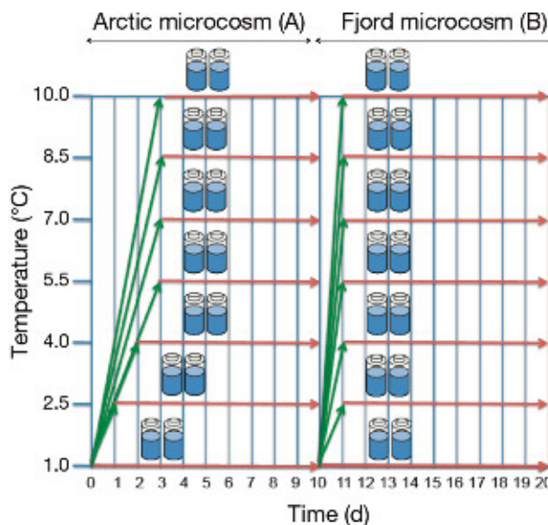
Fig. 2. Schematic representation of 2 experimental microcosms used to study the effects of Arctic warming on microbial communities. Duplicate carboys were incubated at 7 experimental temperatures, ranging from 1.0° to 10.0°C increasing in 1.5°C steps. (A) Arctic microcosms: the temperature was increased gradually over the first 3 d of the experiment from 1.0°C to each final treatment temperature. (B) Fjord microcosms: the temperature was immediately set to each final treatment temperature
