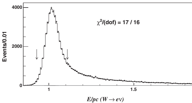
FIG. 2. The distribution of E/pc for the W \rightarrow e\nu data (points) and the best-fit simulation (histogram) including the small jet background (shaded). The arrows indicate the fitting range used for the electron energy calibration. The jet background, which is barely visible on this scale, contributes a negligible uncertainty in the calibrations of the electron energy scale and the amount of radiative material.
