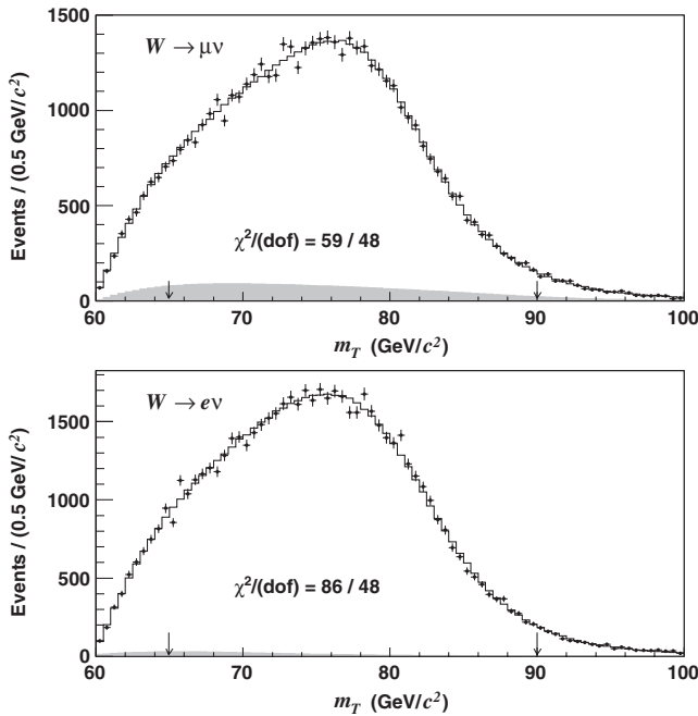
FIG. 4. The m_T distribution of the data (points) and the best-fit simulation template (histogram) including backgrounds (shaded), for muons (top panel) and electrons (bottom panel). The arrows indicate the fitting range. The \chi^2/(\text{dof}) for the electron channel distribution receives large contributions from a few bins near 65 \text{ GeV}/c^2 , which do not bias the mass fit.
