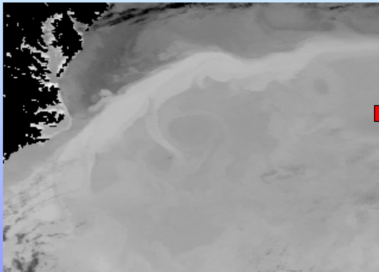
Pathfinder SST Image (Hatteras Cape, May 8, 2000)
