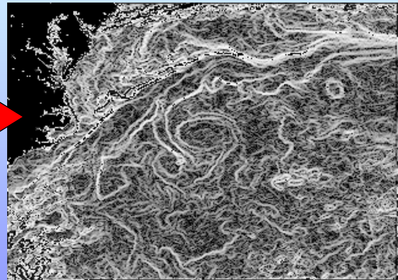
Associated singularity exponents
