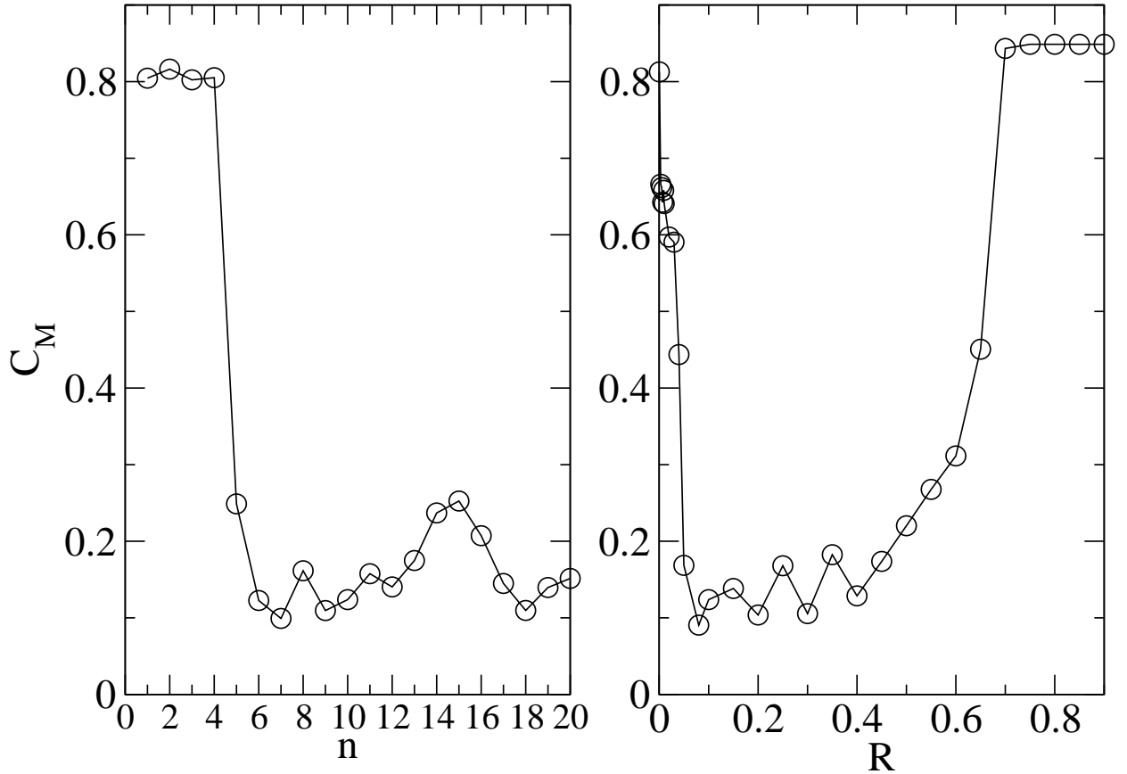
FIG. 1: Left: C_M vs n with R = 0.1 . Right: C_M vs R for n = 10 . In both plots, U_0 = 10 , \sqrt{1 + 2\frac{U_0^2}{V_0^2}} = 2\pi , and the time average is performed over the last 2000 steps in a numerical simulation running for 5000 steps with dt = 0.01 .
