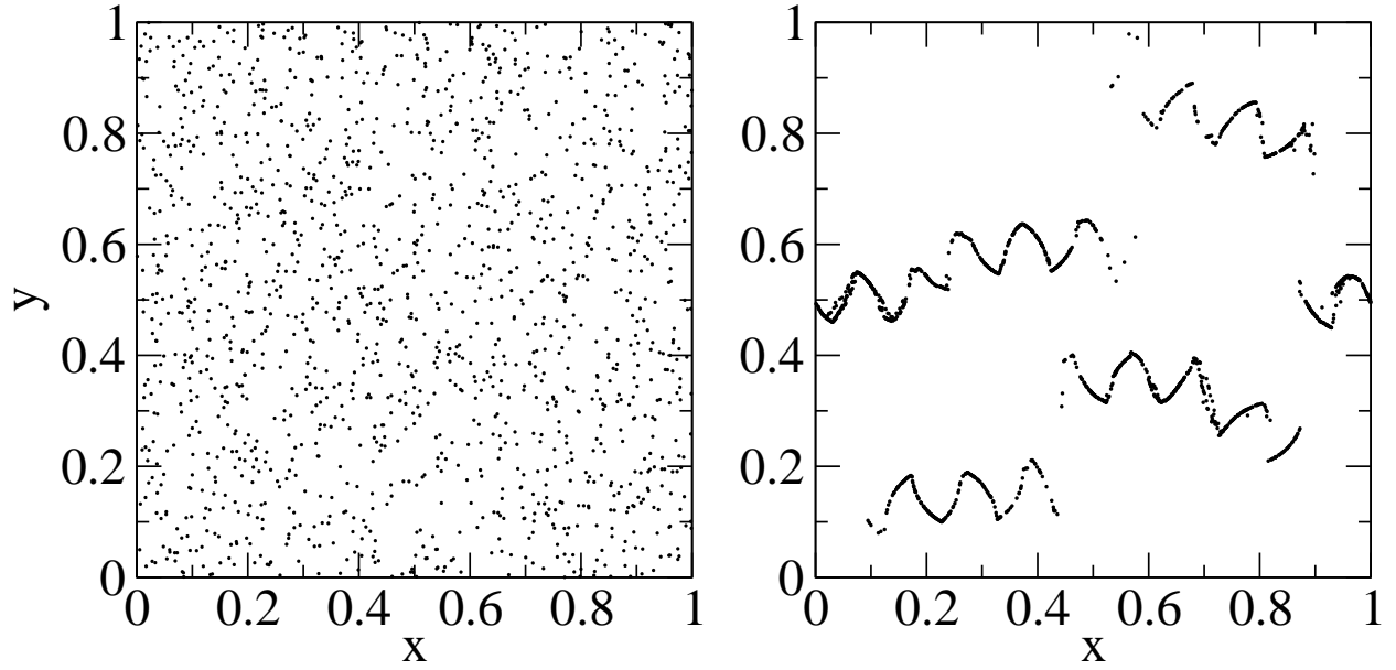
FIG. 2: Spatial distribution (statistically stationary) of particles at time t = 0 (left), and t = 16 (right panel). Here R = 0.1 , n = 10 , U_0 = 1 ( \sqrt{1 + 2\frac{u_0^2}{V_0^2}} = 2\pi , and the initial number of particles N_0 = 1500 ).
