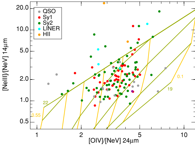
Figure 13. Predicted [\text{Ne III}]15.56 \mu\text{m}/[\text{Ne V}]14.32 \mu\text{m} ratio vs. [\text{O IV}]25.89 \mu\text{m}/[\text{Ne V}]24.32 \mu\text{m} . The green lines trace constant hydrogen column density and the orange lines trace constant ionization parameter. The input parameters for the model are \log n_{\text{H}} (\text{cm}^{-2}) = 19.0, 20.0, 20.3, 20.6, 21.0, 22.0 and I_0 = 0.1, 0.15, 0.20, 0.25, 0.32, 0.4, 0.55 for constant pressure ( \log P/k = 8 ). The galaxy symbols are as in Figure 2.
