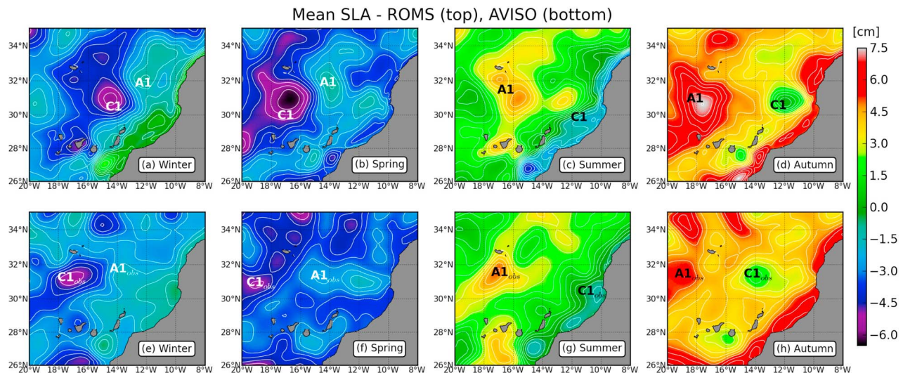
Figure 10. Seasonal mean sea level anomalies. (a–d) The SLAs from L0 and (e–h) the AVISO SLAs (for the same time period as the SCOW wind stress, i.e., 1999–2007) are shown. Contours are plotted in white every 0.5 cm.
