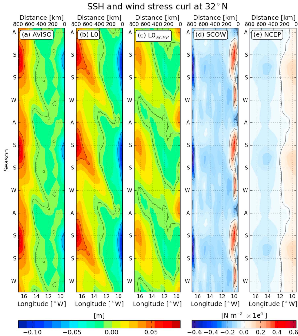
Figure 11. Longitude/time plots showing three repeated yearly cycles of monthly mean SSH and wind stress curl at 32°N (meridionally averaged between 31.5° and 32.5°N). SSH is taken from (a) AVISO altimetry, (b) L0, and (c) L0 NCEP . Contours are shown in black at -0.055, -0.005, and 0.045 m. Years 6–18 (1995–2007) are used from L0/L0 NCEP (AVISO). Wind stress curl is taken from (d) SCOW and (e) NCEP. Contours are shown in black every 0.2 N m -3 × 1e 6 . Intense negative curl in SCOW at the western boundary is associated with Madeira. The seasons are labeled W, S, S, and A for winter, spring, summer, and autumn, respectively.
