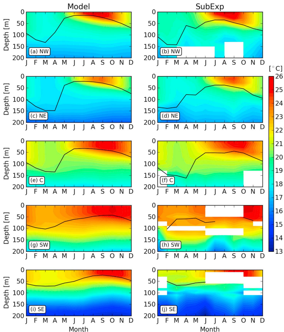
Figure 4. Comparison of monthly mean temperature within the top 200 m from (b, d, f, h, j) the five Subduction Experiment moorings (refer to Figure 1 for the mooring locations) and (a, c, e, g, i) L0. The mixed layer depth is plotted in black. Periods/depths with missing Subduction Experiment data are masked.
