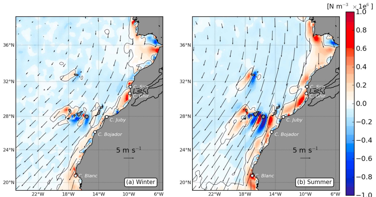
Figure 2. Normalized wind stress curl from the QuikSCAT-derived SCOW wind stress climatology of Risien and Chelton [2008] over the northeast Atlantic in (a) winter and (b) summer. Vectors show the wind speed and direction. The zero wind stress curl is contoured in black. Contours over land (1000 and 2000 m) show the Atlas Mountains.
