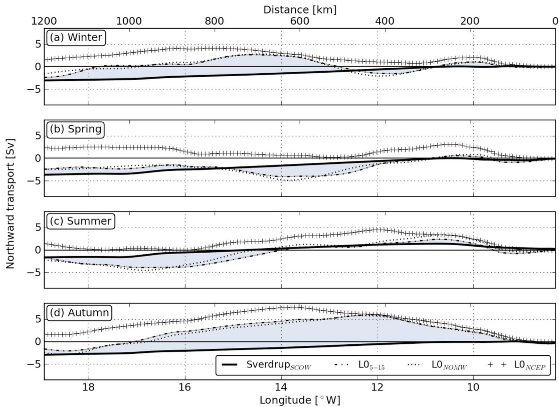
Figure 9. Comparison of seasonal mean accumulated (starting from the eastern boundary) meridional barotropic transports from the model ( L0_{5-15} , L0_{NOMW} , and L0_{NCEP} ), with the Sverdrup transport derived from the curl of the SCOW wind stress. Grey shading highlights difference between L0_{5-15} and Sverdrup_{SCOW} . The transports are meridionally averaged over the latitudes 30.5^{\circ} – 33.5^{\circ} N.
