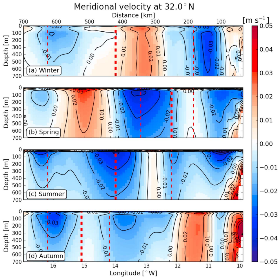
Figure 8. L0 seasonal mean zonal sections of meridional velocity at 32°N. The CanC is visible, particularly in summer where it is centered at \sim 14^\circ\text{W} and reaches 0.05 \text{ m s}^{-1} . Velocity contours are plotted every 0.01 \text{ m s}^{-1} , solid (dashed) contours show northward positive (southward negative) velocity. The thick (thin) red dashed lines show the core (outer limits of the) seasonal positions of the CanC as observed by Machin et al. [2006].
