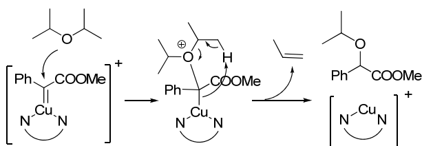
Scheme 4 Reaction between methyl phenyldiazoacetate and diisopropylether
