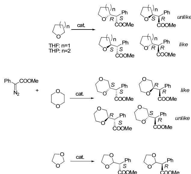
Scheme 1 Insertion reactions of methyl phenyldiazoacetate with different cyclic ethers
