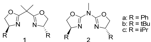
Chart 1 Oxazoline-containing ligands used along this work
