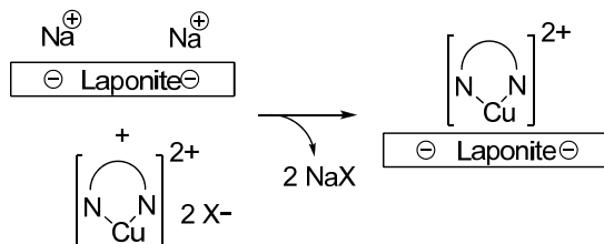
Scheme 2 Cationic exchange on laponite
