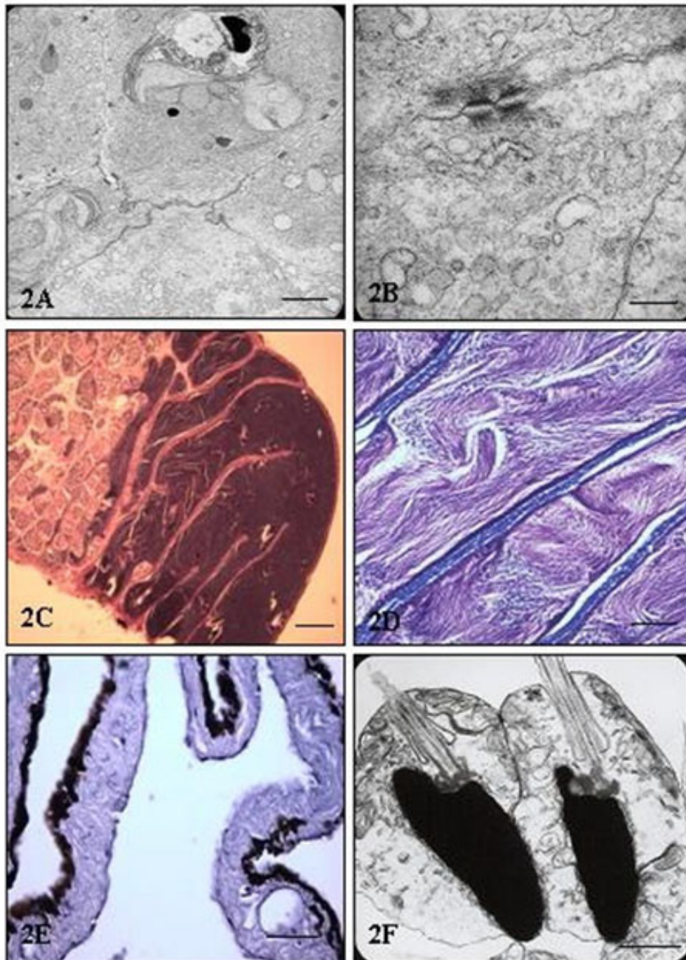
Figure 2. Spermatogenesis in Heliocolerus dactylopterus . A. and B. Tight junctions between Sertoli cells isolate spermatozoa (HRP tracer analysis). Scale bar: 1 \mu\text{m} . C. Mature, spermiated spermatozoa released towards the lobular lumen and accumulate at sperm duct. Scale bar: 20 \mu\text{m} . D. Spermatozoa bundles in efferent ducts during the spawning period. Scale bar: 20 \mu\text{m} . E. Intense brown staining of walls of the sperm duct using the lectin Triticum vulgaris . Scale bar: 15 \mu\text{m} . F. Spermatozoa in the sperm duct with cytoplasmic bag around heads. Scale bar: 2 \mu\text{m} .
