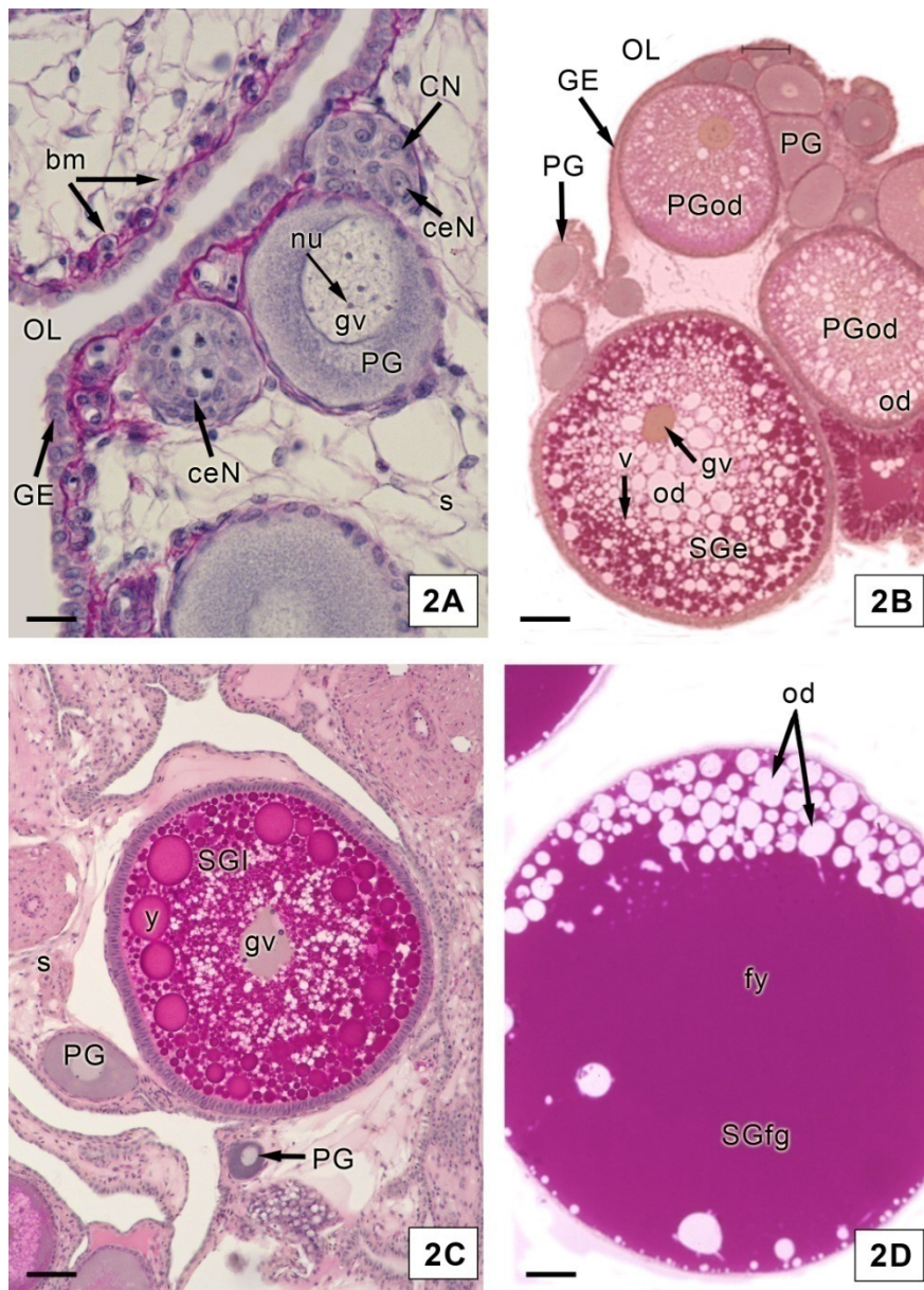
Figure 2. Oocytes in different stages of oogenesis. A. Ovary of the goodeid Ilyodon whitei . The germinal epithelium (GE) lines the ovarian lumen (OL). A periodic acid Schiff-positive basement membrane (bm) is subjacent the germinal epithelia of two lamellae. Cell nests (ceN) contain oocytes in the chromatin nucleolus (CN) stage. The oocyte in the primary growth (PG) stage has multiple nucleoli (nu) in the germinal vesicle (gv) and the ooplasm is basophilic. Bar = 10µm. B. Ovary of the poeciliid Poecilia latipinna . Early in primary growth (PG), oocytes have basophilic ooplasm. Later, oocytes in primary growth (PGod) are larger and contain numerous oil droplets (od). The initial deposition of periodic acid Schiff-positive yolk (v) is seen in oocytes during early secondary growth (SGe). Bar = 20µm. C. Ovary of the goodeid Xenotoca eisenni . Small yolk globules coalesce and increase in size, forming larger yolk gobules (y) during late secondary growth (SGI). Primary growth oocytes (PG) are also seen for growth comparisons. Bar = 30µm. D. Ovary of the poeciliid Poecilia latipinna . In a full-grown oocyte (SGfg) the fluid yolk (fy) has become a single mass and yolk globules are no longer present. Oil droplets (od) are primarily at the periphery of the oocyte. (gv) germinal vesicle; (s) stroma. Bar = 50µm.
