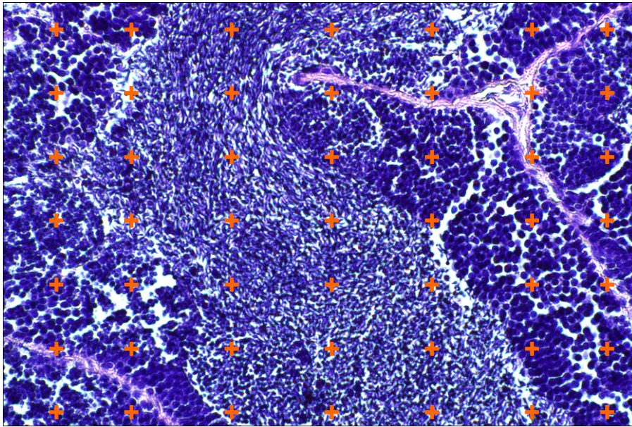
Figure 1. Image of a histological section of a developing testis of European eel with all tissue types present. The image is overlaid by a point grid in order to determine the area of fraction per tissue type.
