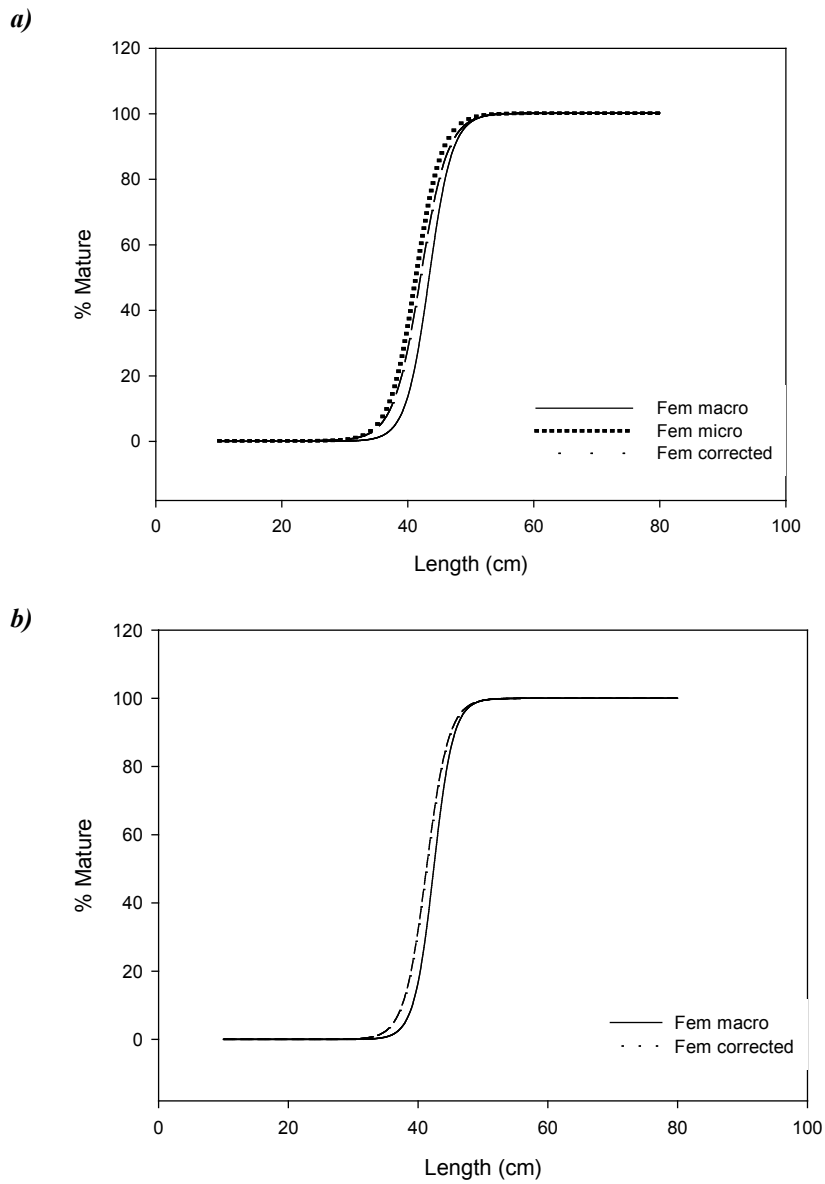
Figure 2. Maturity ogives estimated with different maturity data in a) Vigo and b) Gulf of Cadiz.
