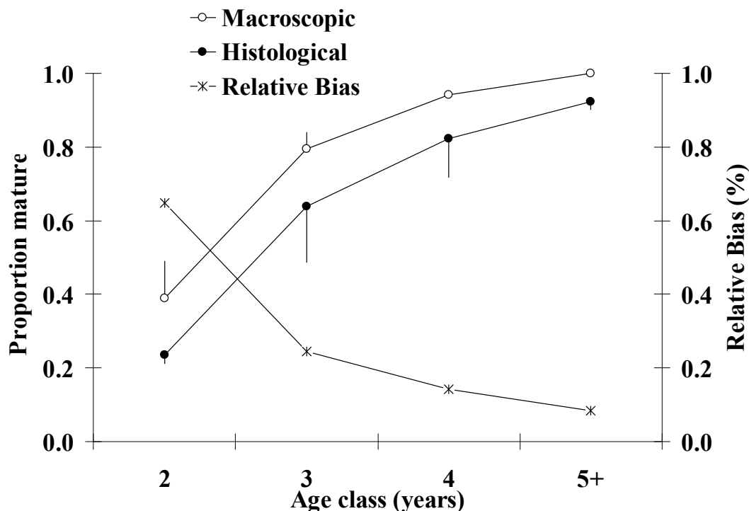
Figure 1. Comparison between histological and macroscopic staging of the gonads. The Relative Bias (%) is calculated per age class. Bars represent standard errors.
