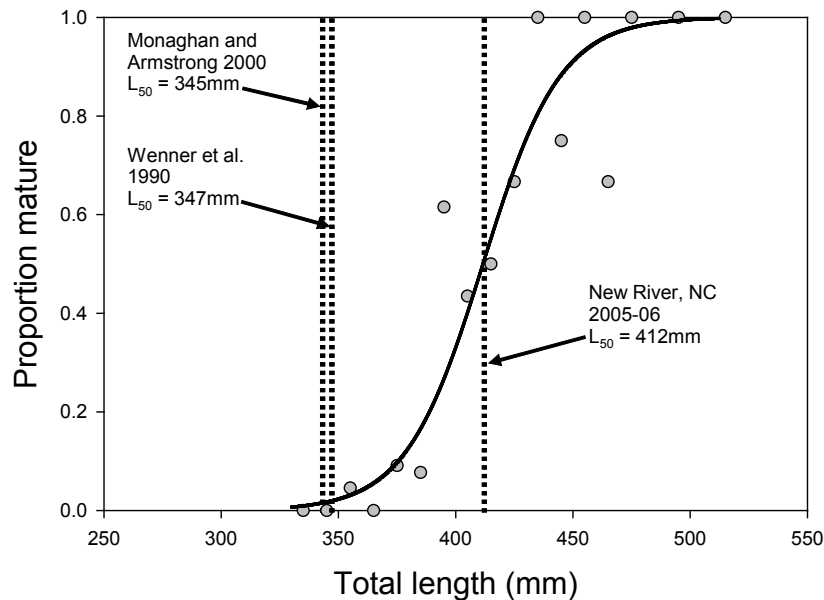
Figure 1. Proportion mature by total length for southern flounder collected during 2005-06 tag-return study (Smith and Scharf in review). Estimated L50 are presented for this data and also for previous studies in North Carolina (Monaghan and Armstrong 2000) and South Carolina (Wenner et al. 1990) waters.
