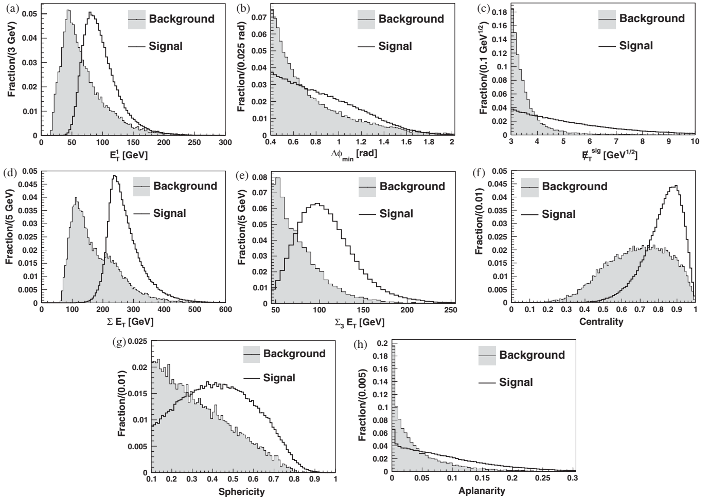
FIG. 3. Distribution of neural network input variables for multijet data (background) and t\bar{t} MC (signal) samples: (a) the transverse energy of the leading jet E_T^1 , (b) \Delta\phi_{\min}(\cancel{E}_T, \text{jet}) , (c) \cancel{E}_T^{\text{sig}} , (d) \sum E_T , (e) \sum_3 E_T , (f) the centrality C , and the topology-related variables (g) sphericity S and (h) aplanarity A .
