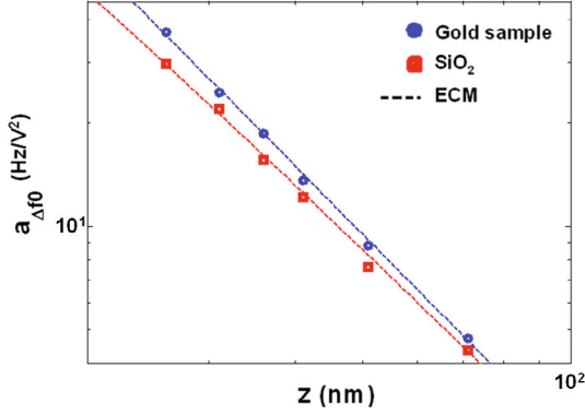
Fig. 9. (Color online) a_{\Delta f_0}(z) curves measured on a conductive gold sample ( \bullet ) and a \text{SiO}_2 /gold sample ( \blacksquare ) with h_{\text{SiO}_2} = 12 nm. The tip radius R = 105 \pm 4 nm is obtained from experiments on gold using ECM. Then, by fitting the \text{SiO}_2 experiments, we calculated the permittivity of the \text{SiO}_2 insulating layer: \epsilon_r = 4.5 \pm 1.1 .
