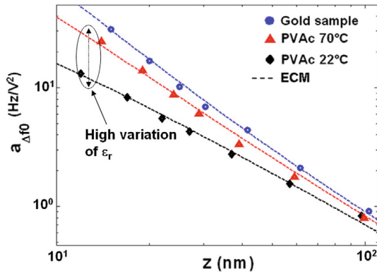
Fig. 11. (Color online) a_{\Delta f_0}(z) curves obtained on a 50 \pm 3 nm PVAc thin film at 22^\circ\text{C} ( \blacklozenge ) and 70^\circ\text{C} ( \blacktriangle ) in comparison with the curve obtained on a gold sample ( \bullet ). The tip radius R = 32 \pm 2 nm is obtained from experiments on gold using ECM. Fitting PVAc parabolic coefficients using ECM, we obtained \epsilon_r = 2.9 \pm 0.3 at 22^\circ\text{C} and \epsilon_r = 8.2 \pm 1.0 at 70^\circ\text{C} .
