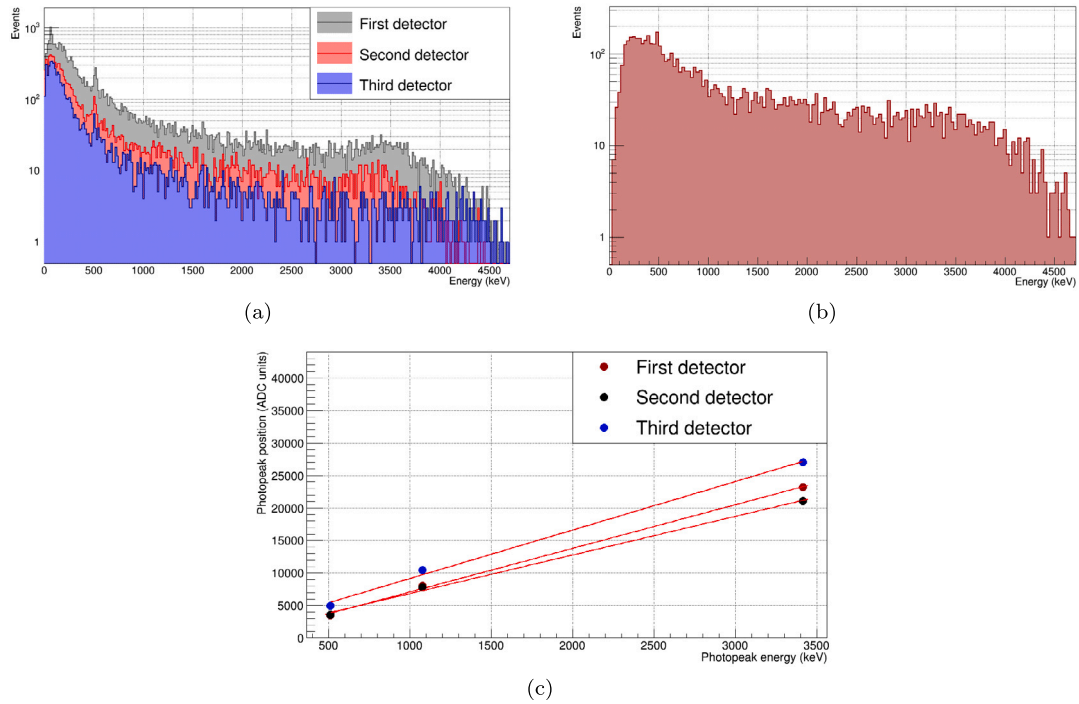
Fig. 4. Detector characterization measurements, the 241 Am- 9 Be data were calibrated using a linear fit for the photopeaks of 511 keV, 3.4 MeV and 1077 keV from the 68 Ge. (a) Calibrated 241 Am- 9 Be spectra measured with the three system detectors in singles mode. (b) Coincidences (sum of energies measured in the first and the second detector). (c) Photopeaks position in ADC units versus photopeaks energy in keV for the data combined of 241 Am- 9 Be and 68 Ge.
