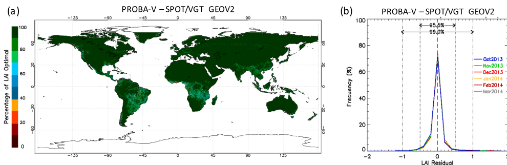
Fig. 5. Consistency between SPOT/VGT and PROBA-V GEOV2 LAI products during the overlapping period from October 2013 to March 2014: (a) Percentage of cases within CGLS optimal uncertainty levels: max(0.5, 20%) LAI; (b) Histogram of residuals per month.
