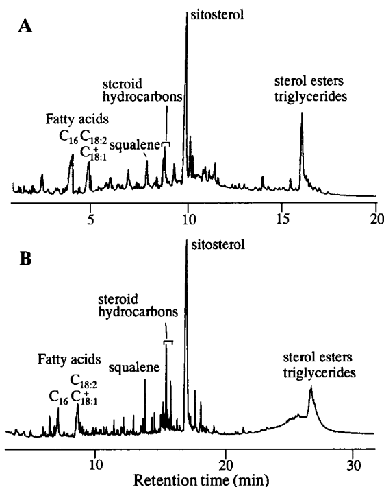
Fig. 4. Chromatograms of the lipid extract of eucalypt wood obtained in (A) GC-FID (DB5-HT, 5 m), temperature-programmed from 100°C (1 min) to 350°C (3 min) at 15°C/min, and (B) GC-MS (DB5-HT, 15 m), temperature-programmed from 120°C (1 min) to 380°C (5 min) at 10°C/min. The identity of major compounds is shown in the chromatograms.
