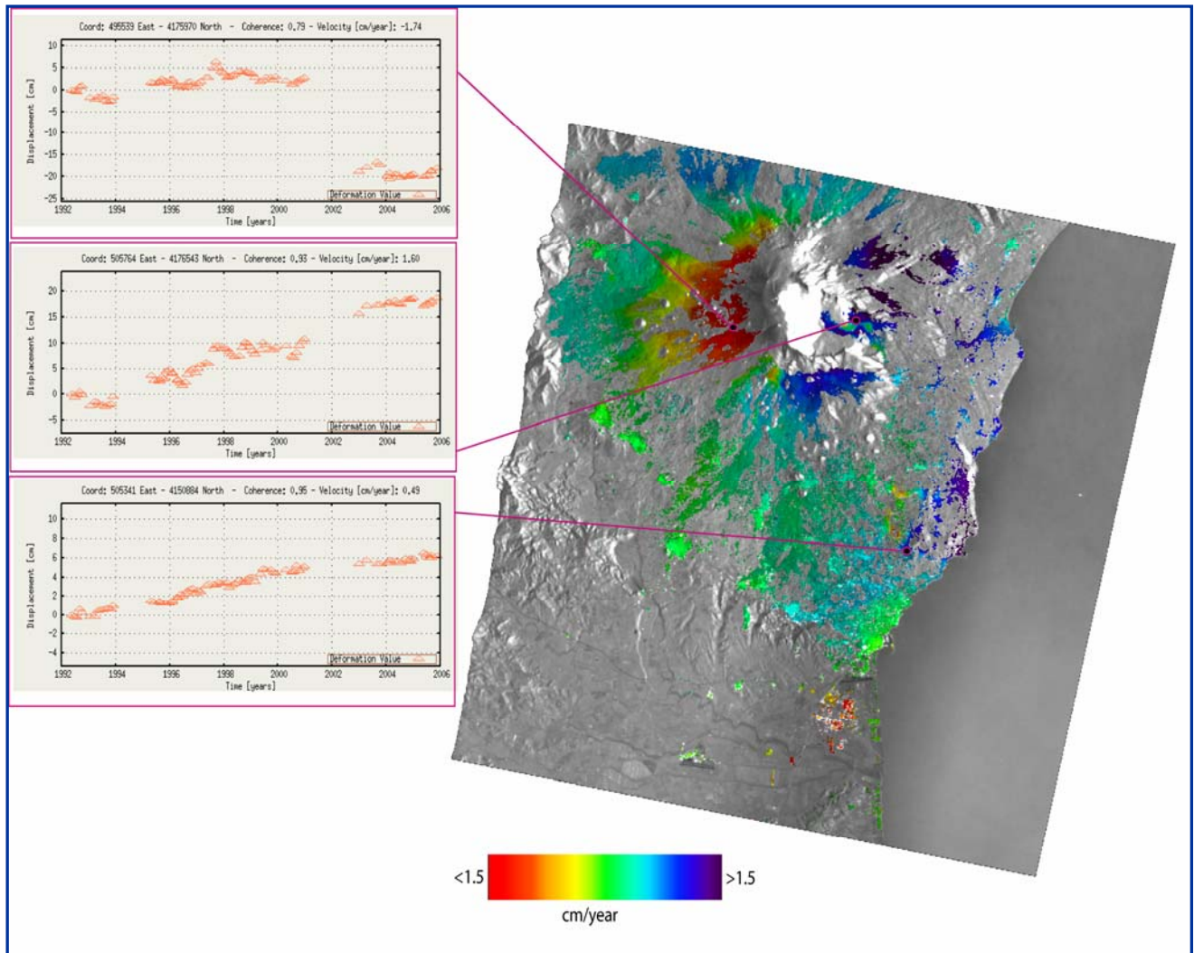
Figure 2. Mean deformations velocity map in LOS of Mt. Etna (1992-2006) computed using ERS/ENVISAT data (descending orbit) superimposed to multilook image of the area. On the left part of the figure are reported the displacement time series, from up to down: the first plot referred to western flank, the second referred to the recent lava flow (1986-1987, 1989) and the third plot referred to Timpe Fault system.
