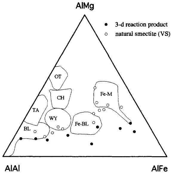
Figure 3. Projection of the octahedral composition of both 3-d reaction product and VS natural-soil smectites in the ternary system AlMg-AlAl-AlFe as proposed by Güven (1988). OT = Otatilla montmorillonite, CH = Chambers montmorillonite, TA = Tatatilla montmorillonite, WY = Wyoming montmorillonite, BL = Beidellite, Fe-BL = Fe-rich beidellite, Fe-M = Fe-rich montmorillonite. AEM analyses are those of Table 2.
