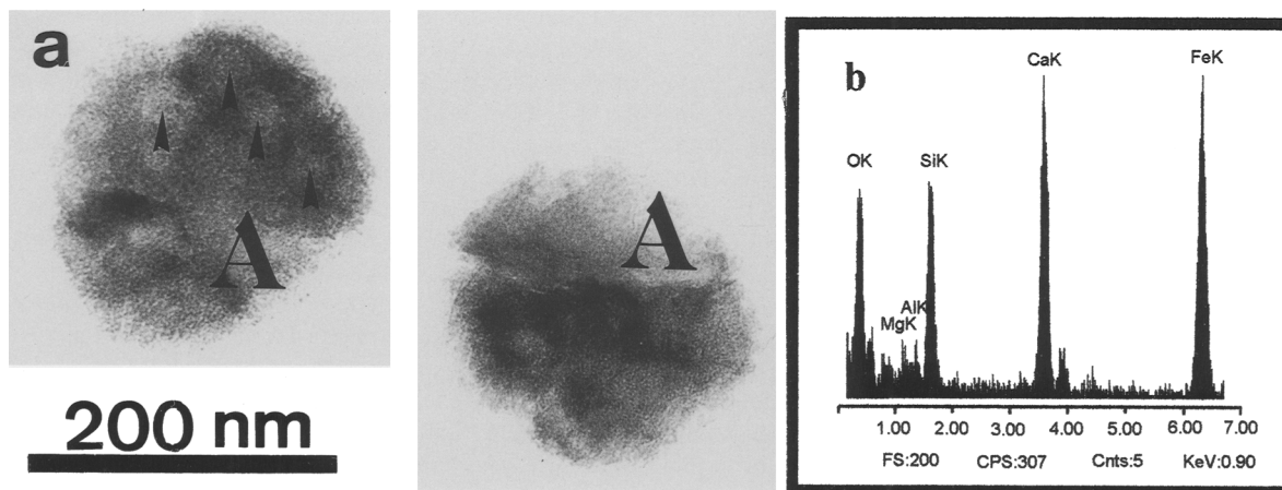
Figure 11. a) Si-Ca-Fe amorphous material formed at 40 d of reaction showing a spheroidal-like morphology with minor rounded particles (arrows) within it. b) EDX spectrum of the rounded material.
