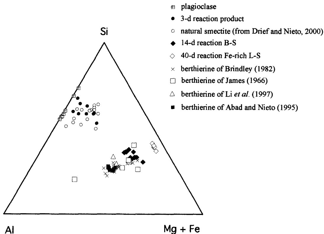
Figure 12. A synthetic plot in the Si-Al-(Fe + Mg) ternary system of the chemical composition of the starting plagioclase, clays formed in the present study along with VS smectite, and berthierine reported in the literature.
