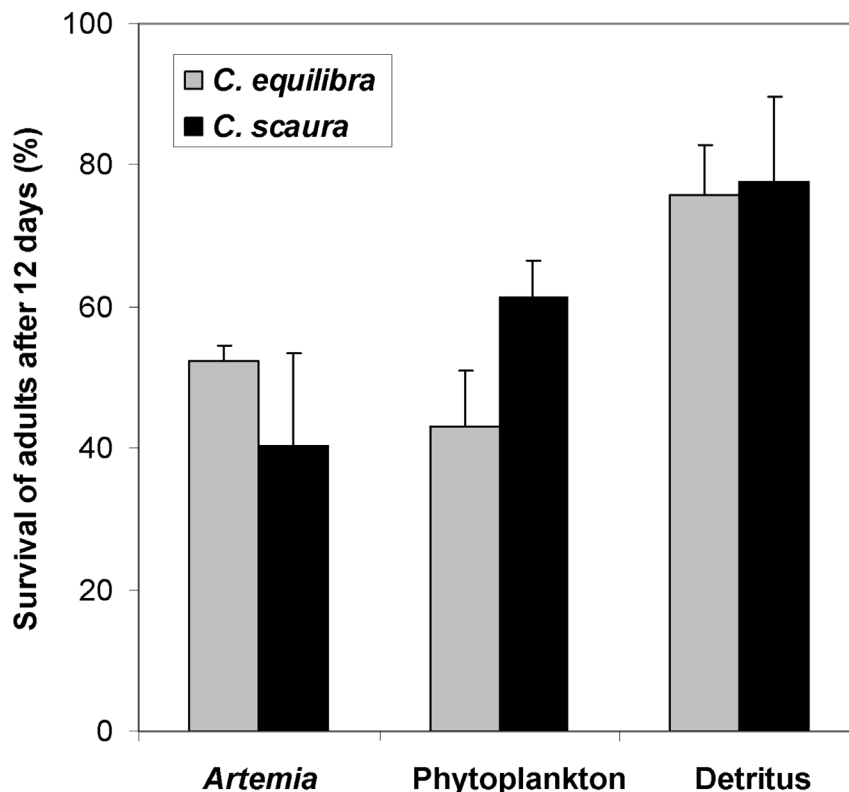
Fig 5. Survival rate (%) of adult specimens of Caprella equilibra and C. scaura after 12 days. Specimens were fed with Artemia, phytoplankton or detritus.
