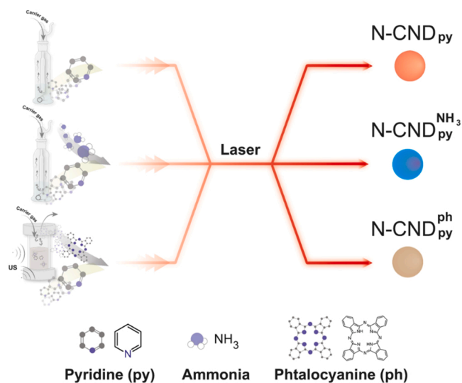
Fig. 1. Simplified scheme of the synthesis of different N-doped CNDs using laser pyrolysis (cw CO 2 infrared laser) and feeding different N-containing precursors.
