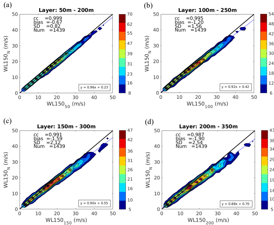
Figure 10. Two dimensional histograms of the dropsonde WL150 at different 150-m layer altitudes versus their corresponding WL150_N (see colourbar). The 150-m layer is placed at 50-200m (a), 100-250m (b), 150-300m (c) 200-350m (d). The same statistical parameters as in Figure 9 can be found in the legend. The corresponding linear fit is also shown at the bottom right side of each plot.
