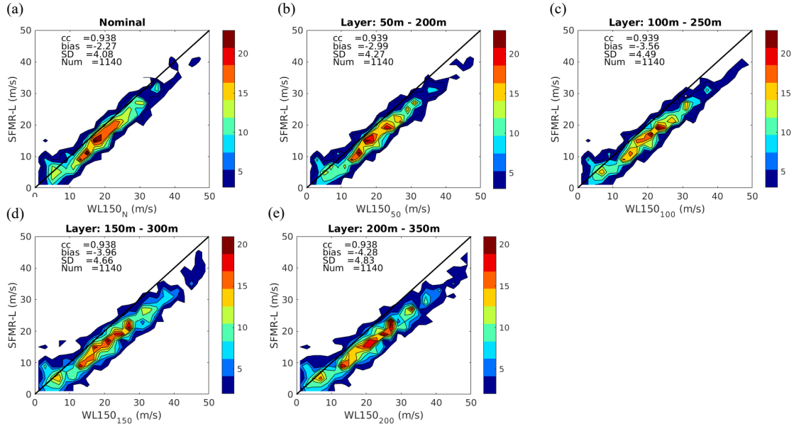
Figure 11. Two-dimensional histograms of the SFMR surface winds at the dropsonde launch time (SFMR-L) versus the collocated dropsonde WL150 winds (see colourbar). The WL150 wind speed is computed using dropsonde with lowest reading altitude ranging between 10-20 m. The 150 m layer is placed at the nominal altitudes (10-160m) (a), 50-200m (b), 100-250m (c), 150-300m (d) 200-350m (e). The same statistical parameters as in Figure 9 can be found in the legend.
