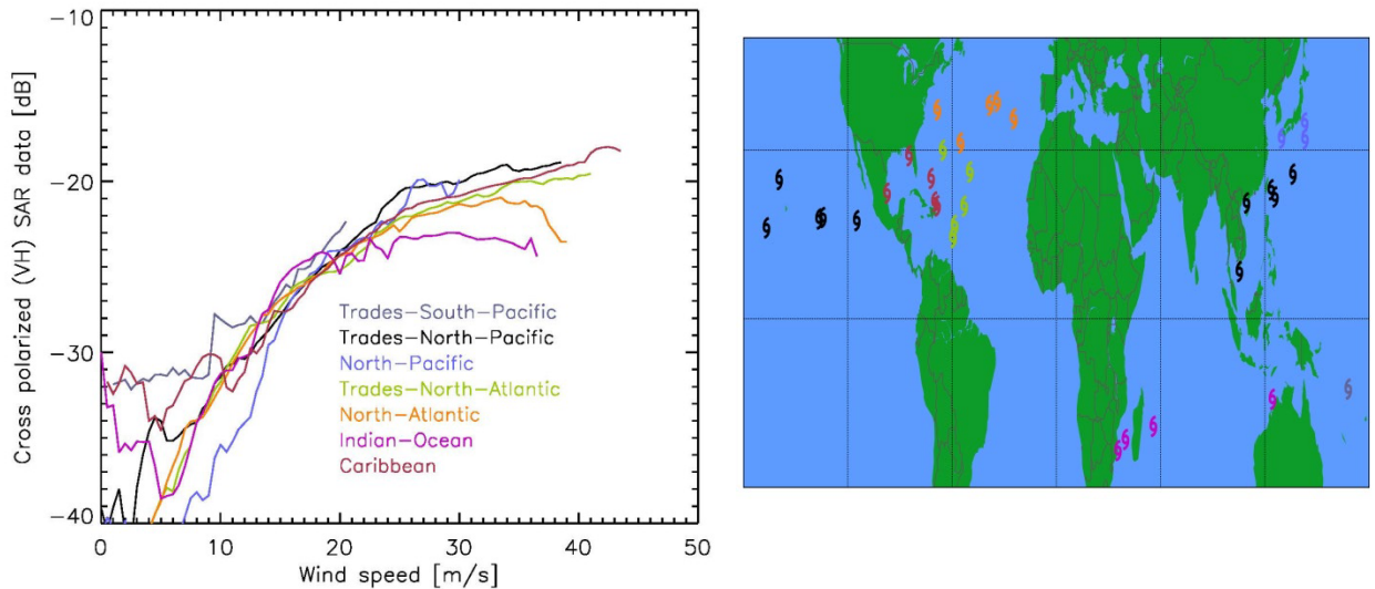
Figure 40. Left panel: Distributions of all the forecasted ECMWF stress equivalent wind speeds ( U_{10s} ) versus collocated VH measurement points from the hurricanes within individual ocean basins. The lines show the median backscatter within 2 m s -1 velocity bins for the distribution, color-coded according to the basin. In the right panel the position of the 32 tropical cyclones considered in this study is shown at the time of the Sentinel=1 overpass.
