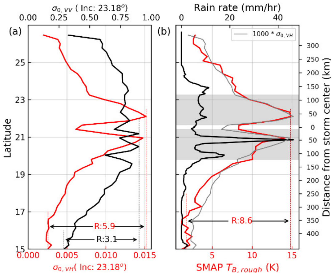
Figure 42: Analysis along transects across a TC eye. (a) Sentinel-1 \sigma^{0,VH} and \sigma^{0,VV} on a grid of 25 km at different latitudes, where the red and black line represent \sigma^{0,VH} and \sigma^{0,VV} , respectively. (b) SMAP T_{B,rough} and IMERG rain rate at different latitudes, where the red and black line represent T_{B,rough} and rain rate, respectively. R gives the ratio of the values indicated by arrows.
