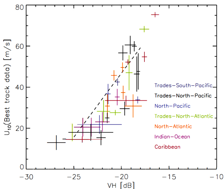
Figure 39. Comparison of the maximum 1-min sustained surface wind speed best-track estimates versus the averaged sum of the VH-GMF retrieved velocities of the 0.995 and 0.9995 percentiles for each hurricane. The error estimates in the x direction show the two percentile values and represent the variability close to the eye within the image, the y direction error bar shows the standard deviation within a 24 h window around the VH measurement, indicative of the variability of the Hurricane as a whole. The color indicates the region in which each hurricane was observed. The dashed line shows the linear relationship from the van Zadelhoff et al. (2014) paper, based on RadarSat-2 observations.
