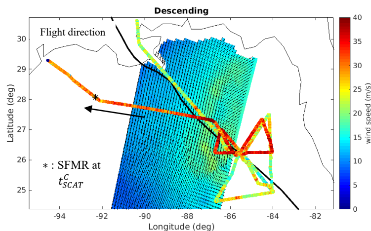
Figure 26. SFMR winds (see colorbar) during the AFRC flight US012 on August 27 th , 2012 for hurricane Isaac. The corresponding ASCAT wind intensities are also shown.
