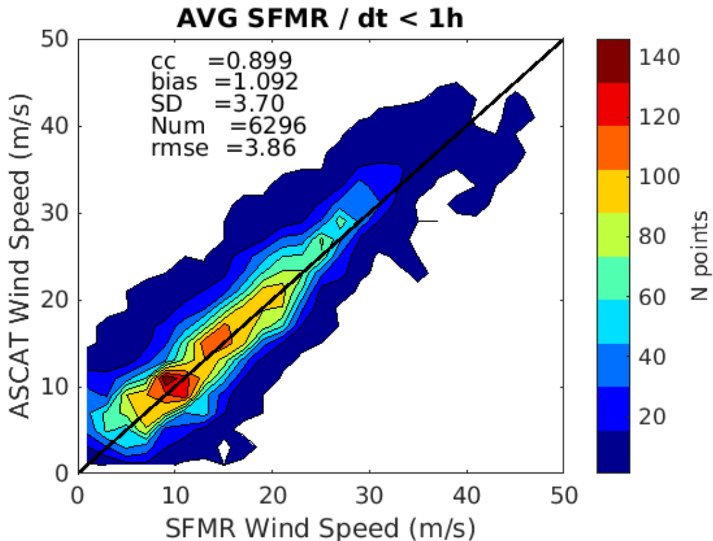
Figure 24. Two-dimensional histograms of ASCAT and collocated SFMR wind speeds, for \Delta t \leq 1h (a) as in the figure above, but now for recalibrated ASCAT winds with respect to SFMR. The same statistical parameters as in Figure 9 can be found in the legend.
