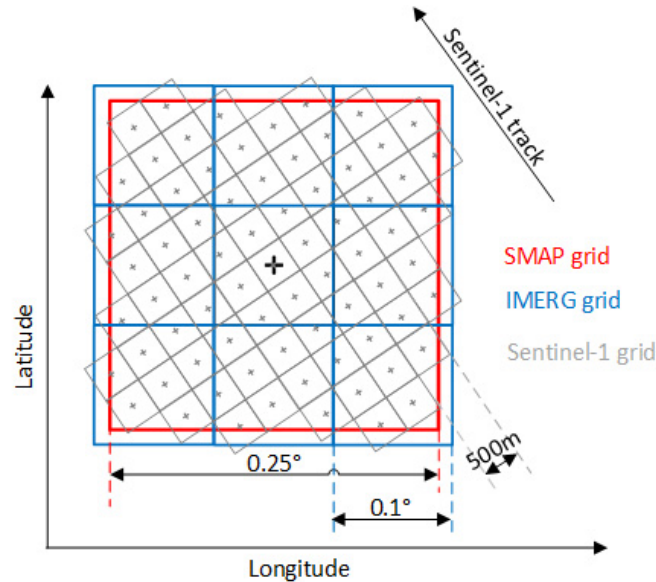
Figure 5: Sketch for illustrating the collocation of Sentinel-1 NRCS, SMAP T_{B,rough} , and IMERG rain rate.
