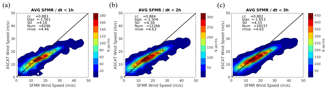
Figure 23. Same as Figure 22, but for collocated SFMR winds averaged over a distance of 12.5 km along track.
