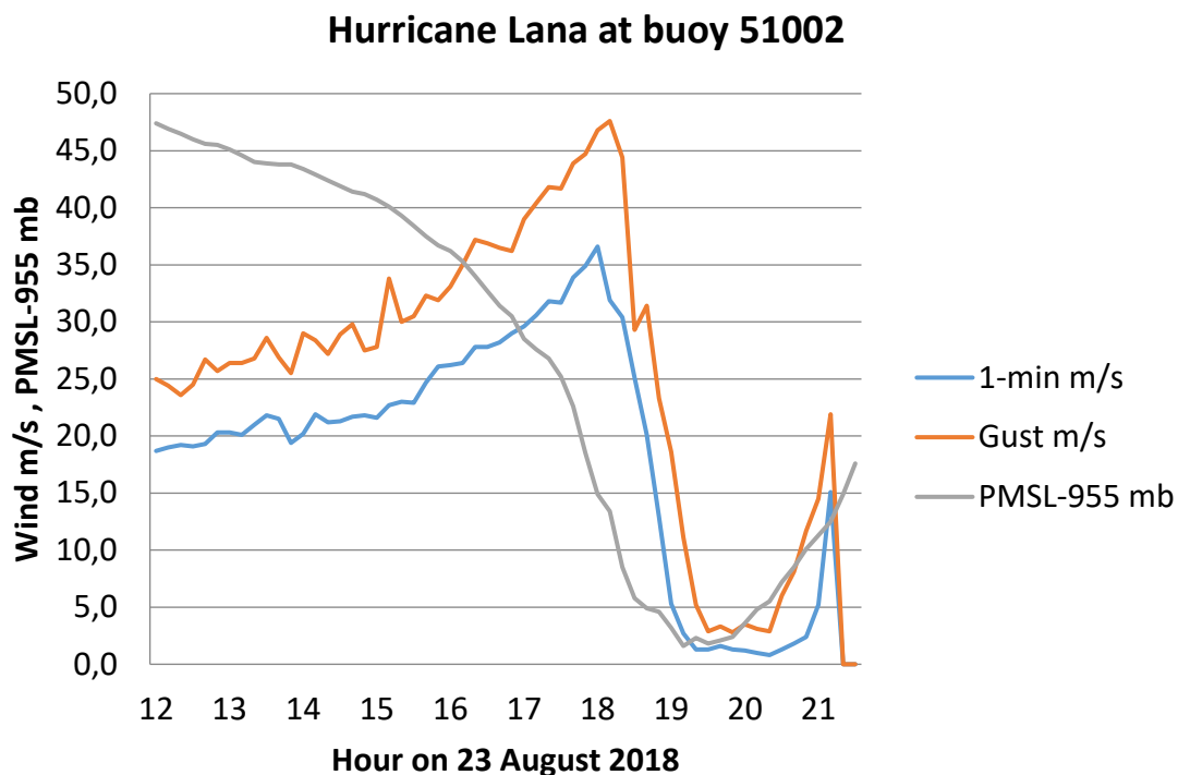
Figure 27. Moored buoy (number 51002) observation in hurricane Lana of mean sea level pressure, PMSL, above its estimated minimum of 955 mb, 1-minute sustained winds and local wind gusts. The wind measurements look credible until the anemometer breaks when the eye wall passes the second time and the PMSL surges.
