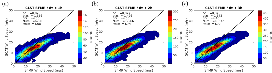
Figure 22. Two-dimensional histograms of ASCAT and collocated SFMR wind speeds, for \Delta t \leq 1h (a), \Delta t \leq 2h (b), \Delta t \leq 3h (c). The same statistical parameters as in Figure 9 can be found in the legend.
