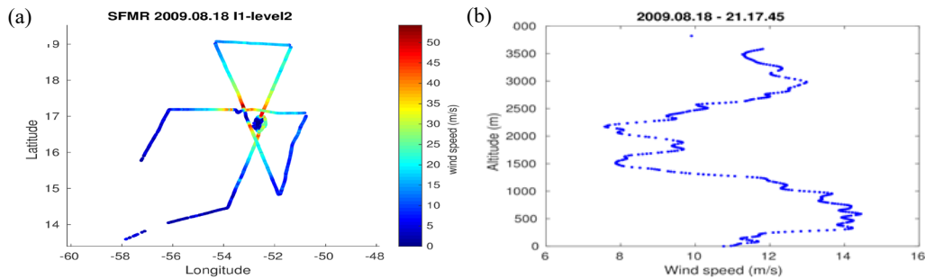
Figure 1. (a) Wind variation during the NOAA hurricane hunters flight experiment on August 18 th , 2009. Wind data are obtained from SFMR measurements. (b) Dropsonde wind profile acquired from NOAA hurricane hunter during that same flight experiment.
