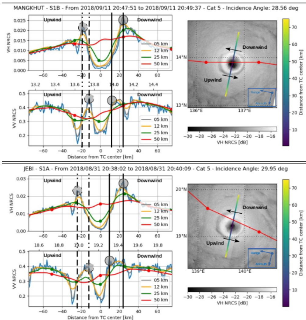
Figure 33. VH and VV NRCS transects across cat-5 TC for incidence angle of 30 degrees. To note, it seems that the saturation observed in VV signal occurs for VH NRCS values at about 0.01 (i.e., -20dB). From previous work, this roughly corresponds to ocean surface wind speeds of 30-35 m s^{-1} .
