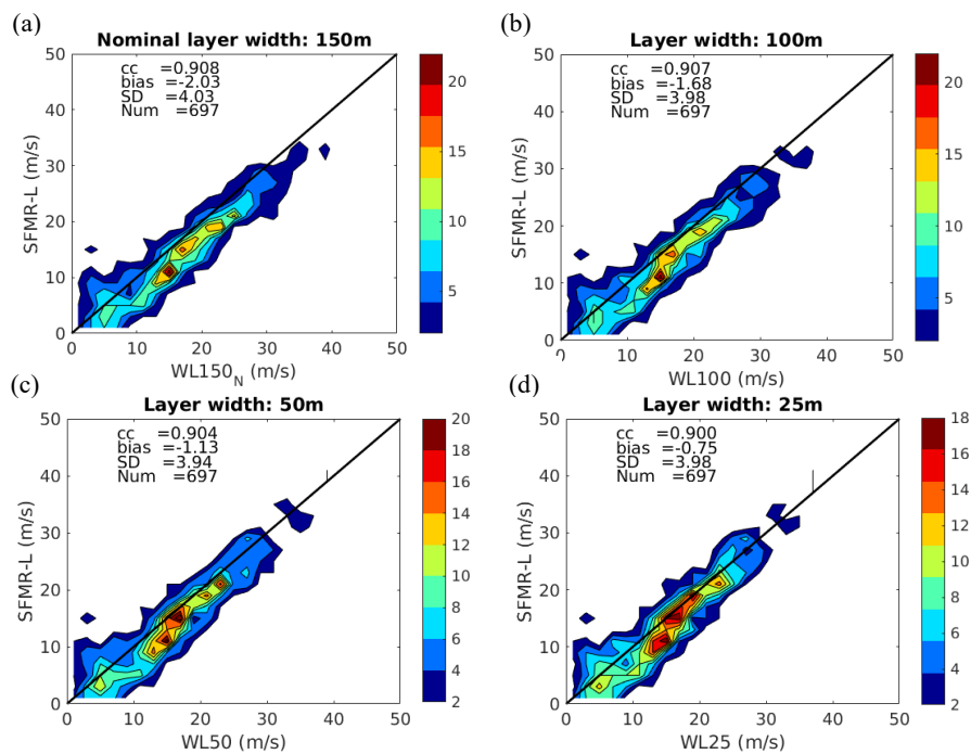
Figure 14. Two-dimensional histograms (see color bar) of the SFMR surface wind speeds at the dropsonde launch time (SFMR-L) and collocated dropsonde averaged winds. The dropsonde averaged wind speed is computed by using different layer widths of 140-150m (a), 90-100m (b), 40-50m (c), and 15-25m (d). The data have been filtered such that dropsondes having the layer lowest reading altitude between 10-20 m and a minimum of 5 readings per layer have been used. The same statistical parameters as in Figure 9 can be found in the legend.
