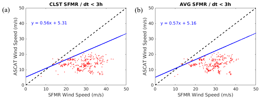
Figure 25. (a) Regression line (solid line) of the ASCAT/SFMR wind comparison as shown in Figure 22c. (b) Same as (a) but using the collocated averaged SFMR wind, as shown in Figure 23c. The equation of the regression line is shown in the legend. The red dots identify the outliers.
