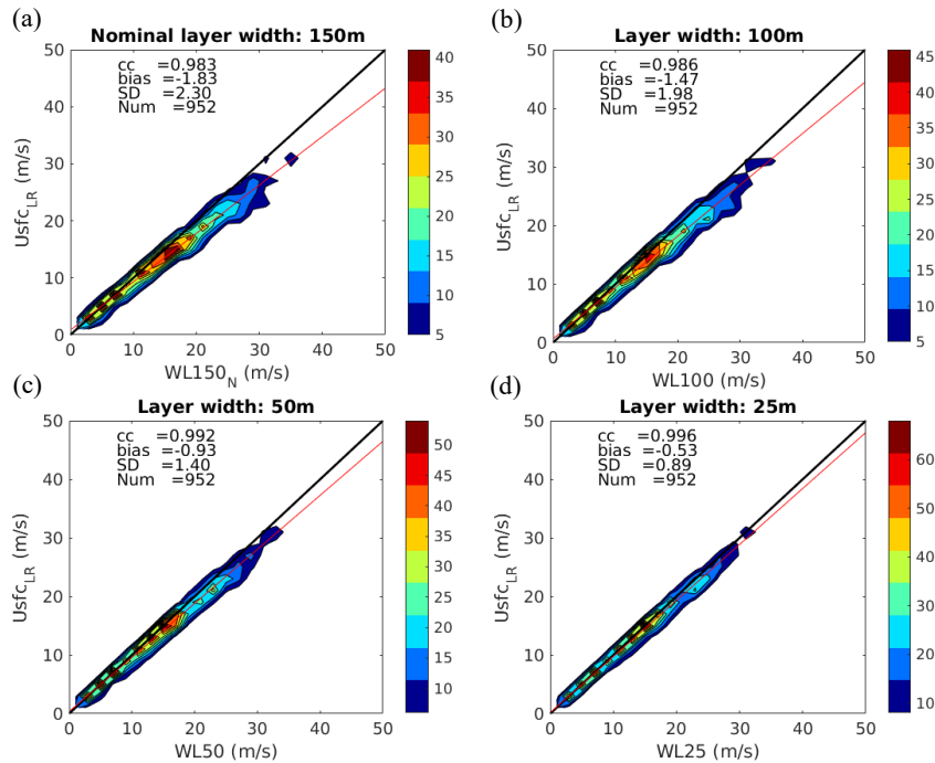
Figure 13. Two-dimensional histograms (see colourbar) of the dropsonde 10 m surface wind measurement and the dropsonde WL averaged winds at different layer widths: (a) 145m-150m ( WL150_N ), (b) 95m-100m ( WL100 ), (c) 45m-50m ( WL50 ) and (d) 20m-25m ( WL25 ). All the layers correspond to the lowest altitude level, i.e., with a lowest reading around 10 m. The same statistical parameters as in Figure 9 can be found in the legend.
