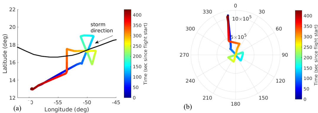
Figure 20. NOAA flight SFMR170903H1 during hurricane Irma on September 3 rd , 2017. (a) Aircraft trajectory in original coordinates with respect to time (see colourbar), along with the BT data (black line); (b) Corresponding flight in storm-motion relative coordinates.
