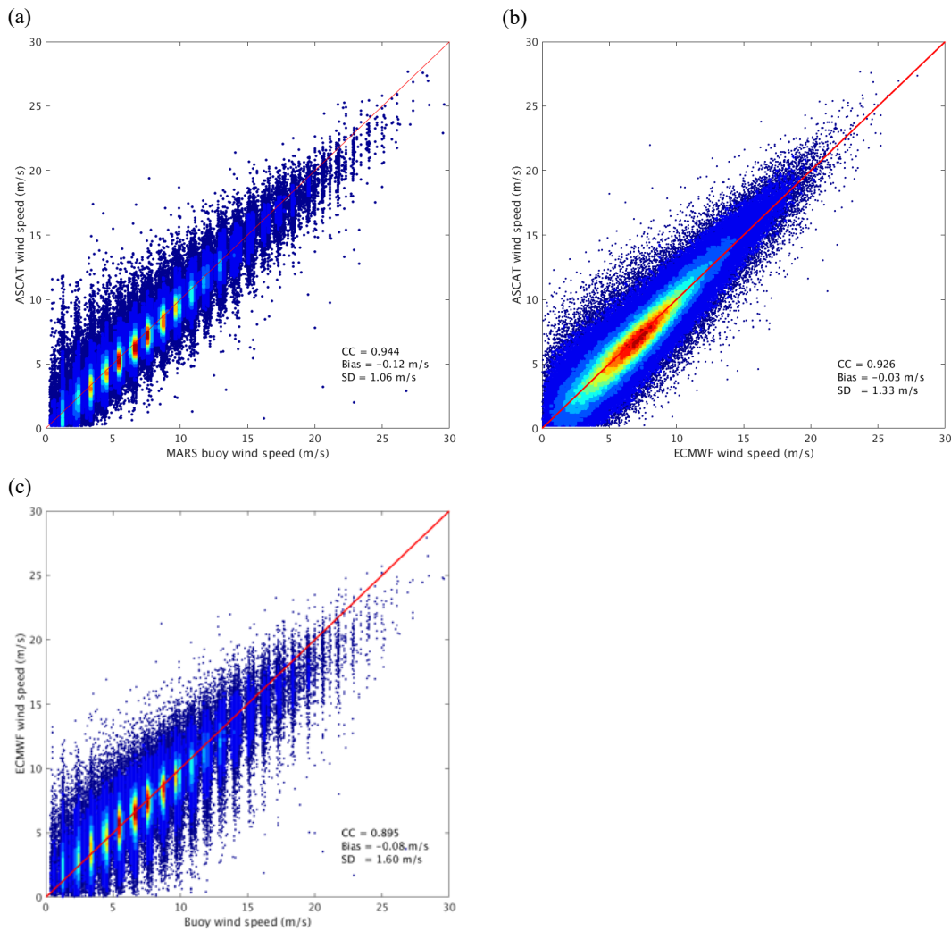
Figure 31. Scatter-density plot of (a) ASCAT U_{10S} wind speed versus MARS buoy U_{10N} wind speed; (b) ASCAT U_{10S} versus ECMWF U_{10N} ; and (c) ECMWF U_{10N} versus buoy U_{10N} . The scores of the correlation coefficient (CC), the bias, and the SD of the speed differences are shown in the legend. The total number of points is about 350,000.
