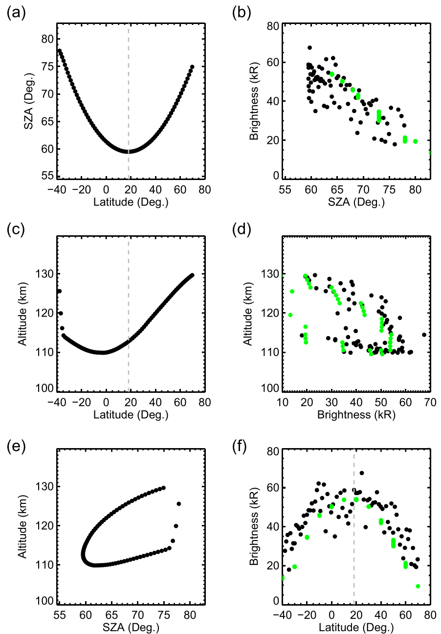
Figure 10. Nadir and Occultation for MArS Discovery/Ultraviolet and Visible Spectrometer limb tracking observation acquired on the 15 February 2021 ( L_s = 4^\circ ) based on 78 spectra (black dots). The left panels represent the geometry of the observation, scanning the Mars atmosphere at almost fixed altitude \sim 120 km (upper peak of the green line) from 40^\circ\text{S} to 70^\circ\text{N} . The vertical dashed lines in panels (a and c) represent the latitude where the SZA is minimum. The right panels show the brightness evolution of the green line as a function of SZA, altitude and latitude. Model simulations are shown with green dots.
