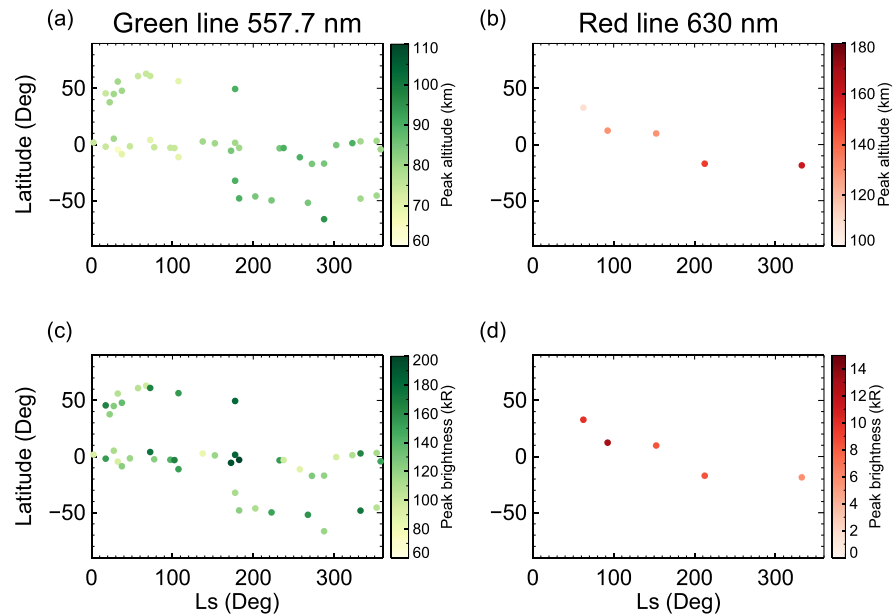
Figure 8. Variation of the peak altitude (top panels) and peak brightness (lower panels) of the oxygen green line (left panels) and red line (right panels) over seasons. Data points are generated using bins of 5^\circ of solar longitude ( L_s ) and latitude for the green line. Bins of 15^\circ of solar longitude are used for the red line.
