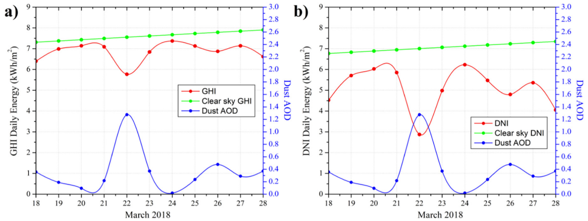
Fig. 9. Daily energy in kWh/m 2 under aerosol-free (green line) and dust aerosol conditions (red lines) for GHI (a) and DNI (b) for the region of Finokalia during the period 18–28 March 2018. The dust AOD is also shown in blue in order to highlight the impact on solar energy, especially during the dust event peak on March 22nd.
