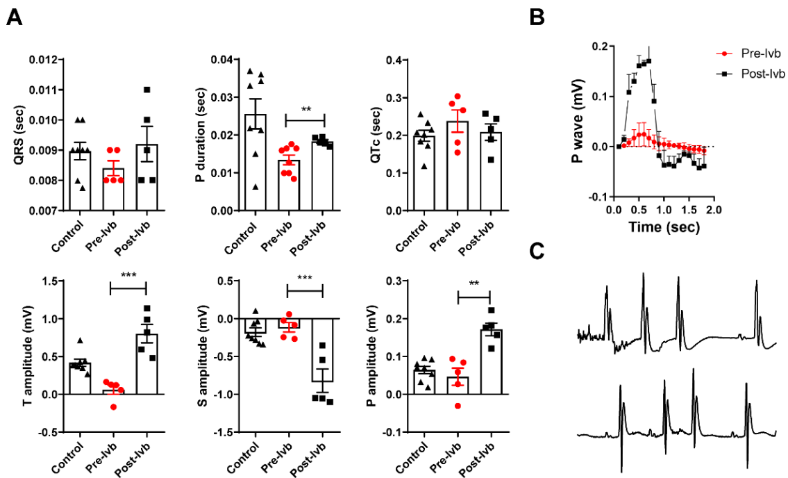
Figure 3. Quantitative/qualitative analysis of ECG parameters after continuous treatment with ivabradine (Ivb) in mice at the EA phase of infection. (A) Differences in wave voltages and amplitudes between treated (Post-Ivb) and untreated (Pre-Ivb) mice. Statistical significance was analyzed by one-way ANOVA (** p < 0.01 and *** p < 0.001 ). (B) Bimodal P-wave morphology, as seen in the mean P-wave trace. (C) Supraventricular ectopic beats were registered after continuous ivabradine treatment in chagasic mice.
