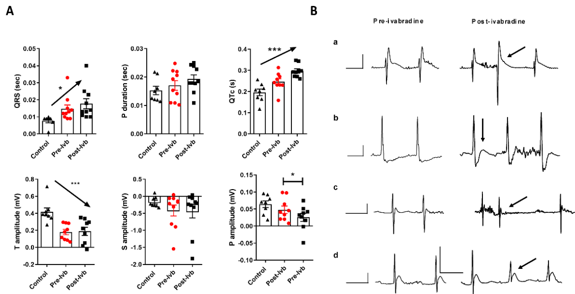
Figure 2. Quantitative/qualitative analysis of ECG parameters after a single-dose treatment with ivabradine (Ivb) in mice at the EA phase of infection. (A). ECG intervals (QRS, P duration, and QTc) and amplitudes (T, S, and P) were determined for control and infected mice before (Pre-Ivb) and after (Post-Ivb) treatment with ivabradine. An unpaired Student’s t -test was performed for statistical comparison (* p < 0.05 ), and a one-way ANOVA post-test for trends indicated in arrows (* p \leq 0.05 and *** p \leq 0.001 ). (B) Representative ECG recordings pre- and post-Ivb treatment. Registers a–d were taken from different infected mice, where a indicates a junctional ectopic beat (arrow), b the QRS enlargement with S blockage, and c–d illustrate atrial ectopic beats.
