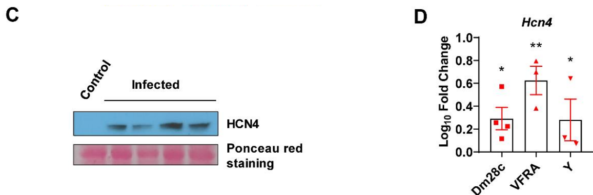
Figure 5. HCN4 expression in heart tissue. (A) Confocal immunofluorescence staining of auricles from control and infected mice at the EA phase using anti-Cx43 and anti-HCN4 antibodies, along with DAPI for nuclear visualization and to delimitate structural relationships in the nodal region of the right auricle. (B) HCN4 mean fluorescence was determined in control and infected samples. (C) Western blot analysis of ventricles was performed to estimate HCN4 expression in control and infected mice at the EA phase. The membrane was stained with Ponceau red before incubating with antibodies as a protein load control. (D) Hcn4 mRNA expression in hearts of control and infected mice at the EA phase. Fold change in each infected group was calculated compared to control (“0” value in log 10 scale). Statistical analysis was undertaken using an unpaired Student’s t-test of the infected and the control groups in B and D (* p < 0.05 ; ** p < 0.01 ).
