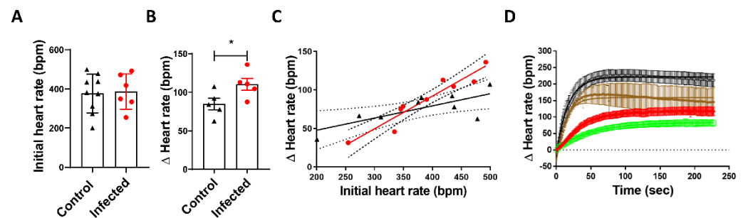
Figure 1. Heart rate kinetics in mice. (A) Initial heart rate in beats per min (bpm) in control (black symbols) and infected (red symbols) mice. (B) The \Delta heart rate, defined as the differential of the heart rate at point 0 and 5 min post-ivabradine single-dose treatment, in control (black symbols) and infected (red symbols) groups. * The p -value was estimated at 0.0425 by Student's t -test. (C) Linear regression between initial heart rate and the \Delta heart rate in control (black symbols) and infected (red symbols) groups. Slopes were considered significantly different with a p -value of 0.0036. (D) Control mice were treated (brown symbols) or not treated (black symbols) with a single bolus of 5 mg/kg of ivabradine five minutes before stimulation with 1.1 mg/kg isoproterenol; infected mice were treated (green symbols) or not treated (red symbols) with ivabradine, like the control mice.
