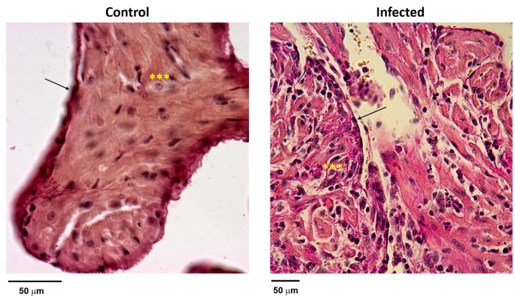
Figure 4. Histological sections of auricles stained with Van Gieson’s stain. The left panel shows the normal morphology of cells compatible with pyramidal P cells (***) and peripheral fusiform fibroblast-like cells (arrow) located externally to the nodal area. Structural relationships are well-defined and conserved. The right panel shows the right auricle of the infected tissue with loss of structure and depopulation of pyramidal cells. A moderate mononuclear infiltrate can be appreciated. Fusiform fibroblast-like cells preserve morphology and location (arrow).
