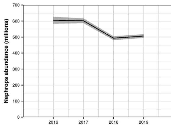
Fig 3. FU1 Iceland: Stock abundance (Underwater TV, millions; SSB proxy, 95% confidence intervals).
