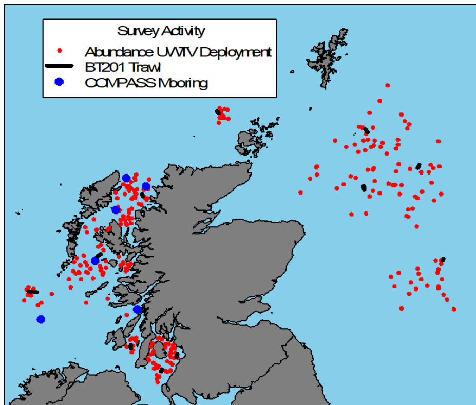
Figure 5.1.3.3. Map illustrating the location of the various UWTV activities, ACDP deployments and COMPASS mooring recoveries that were conducted within the seven survey areas during the MRV Scotia cruise in June 2019.
