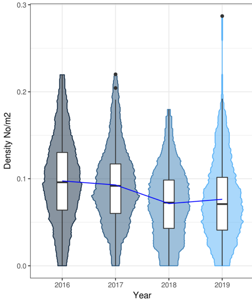
Fig 2. FU1 Iceland: Violin and box plot of adjusted burrow density distributions by year from 2016 - 2019. The blue line indicates the mean density over time. The horizontal black line represents the median, white box is the inter quartile range, the black vertical line is the range and the black dots are outliers.
