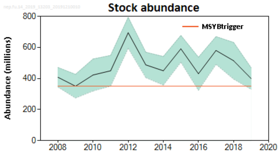
Figure 5 – Nephrops abundance for 2009 – 2019.
