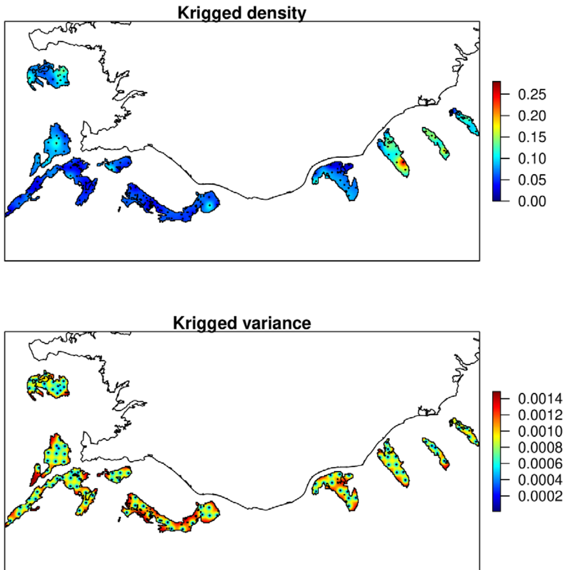
Fig 1. FU1 grounds: Contour plots of the krigged burrow density (per 100m 2 ) estimates (above) and krigged variance (below), from the 2019 survey. Black crosses represent the stations.
