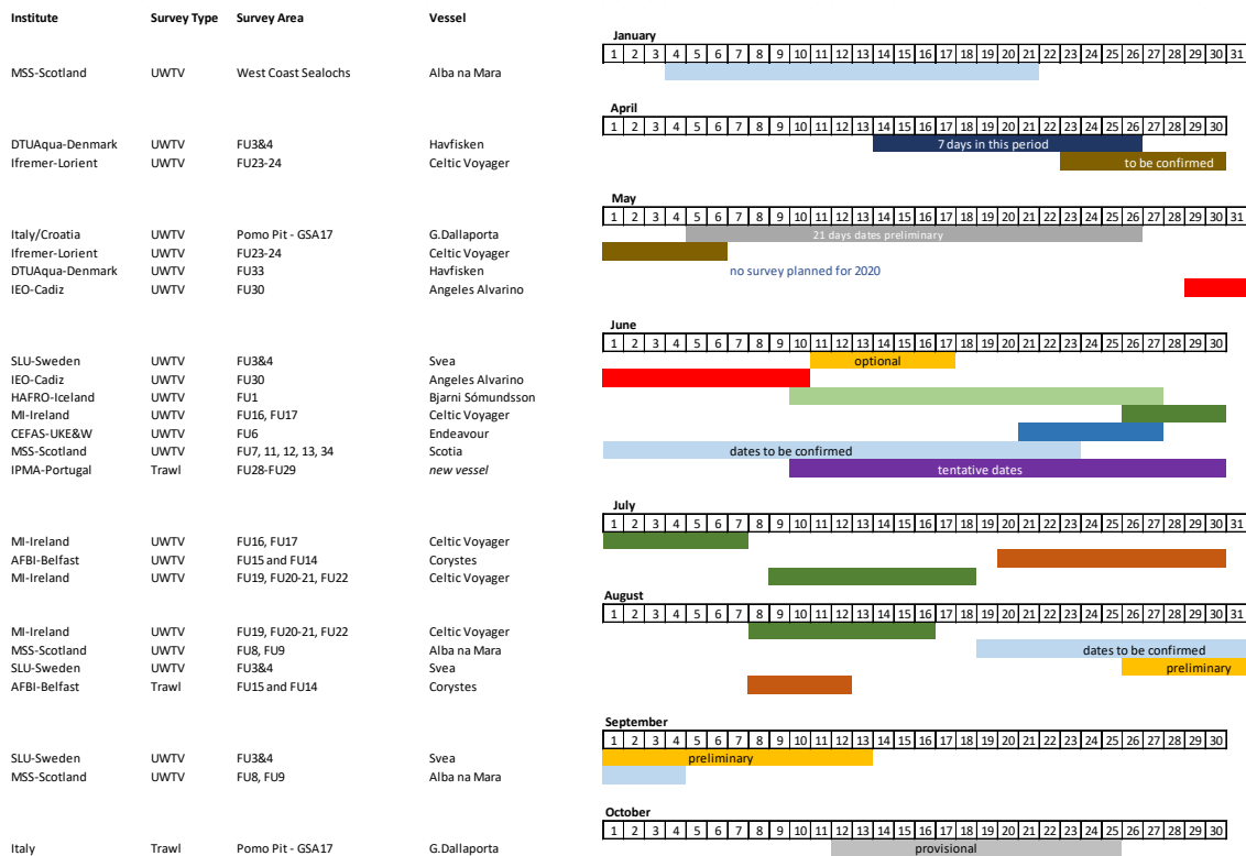
Figure 1.2 Nephrops surveys conducted in 2019 and survey schedule for 2020.
