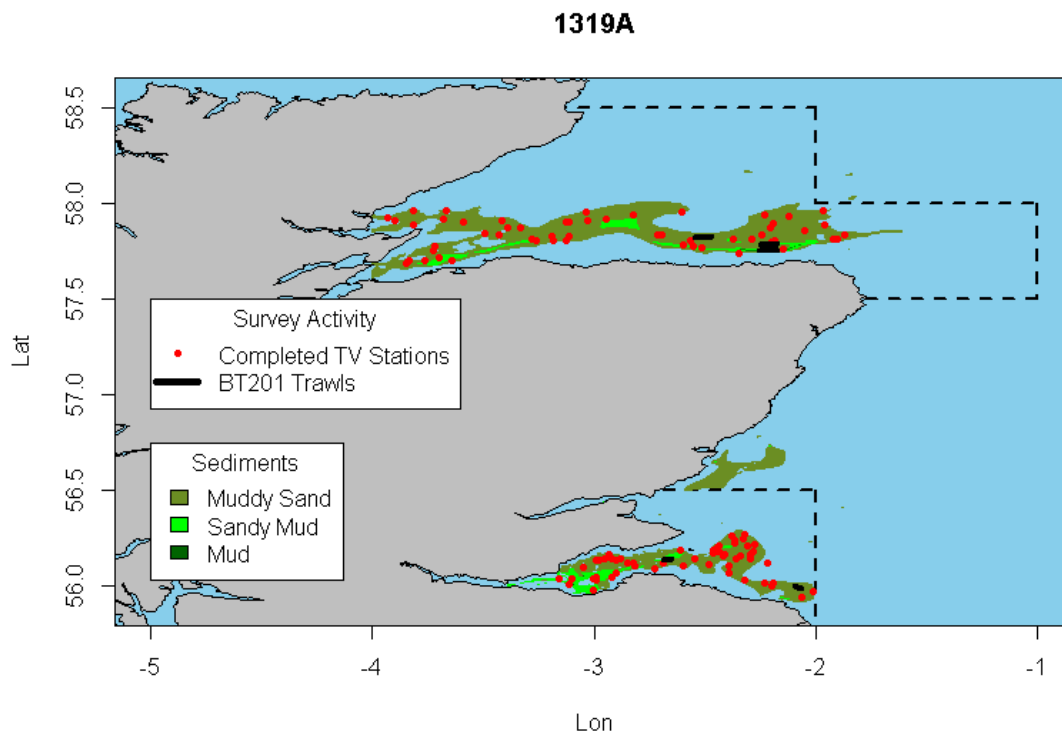
Figure 5.1.3.4. Map illustrating the location of the various UWTV activities carried out during the MRV Alba-na-Mara cruise during August 2019 within the Firth of Forth (FU 8) and the Moray Firth (FU 9).
