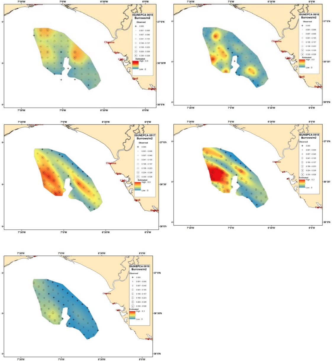
Figure 1: Gulf of Cadiz (FU 30). Bubble plot of the burrow density observations overlaid on a head map krigged burrow density surface for UWTV survey series (2015-2019). Station positions with zero density are indicated using a +.
