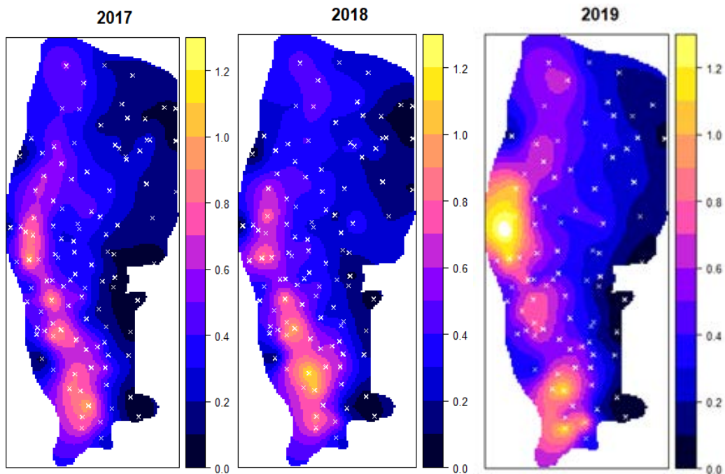
Figure 3 – Geostatistical outputs 2017 – 2019, maps of Nephrops density distribution (m 2 ).
