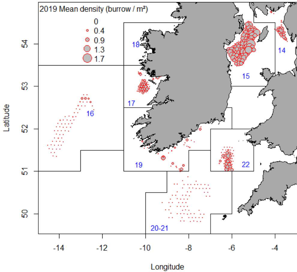
Figure 3. 2019 Mean adjusted density estimates (burrow/m 2 ) by station for Nephrops grounds in ICES Subarea 7.
