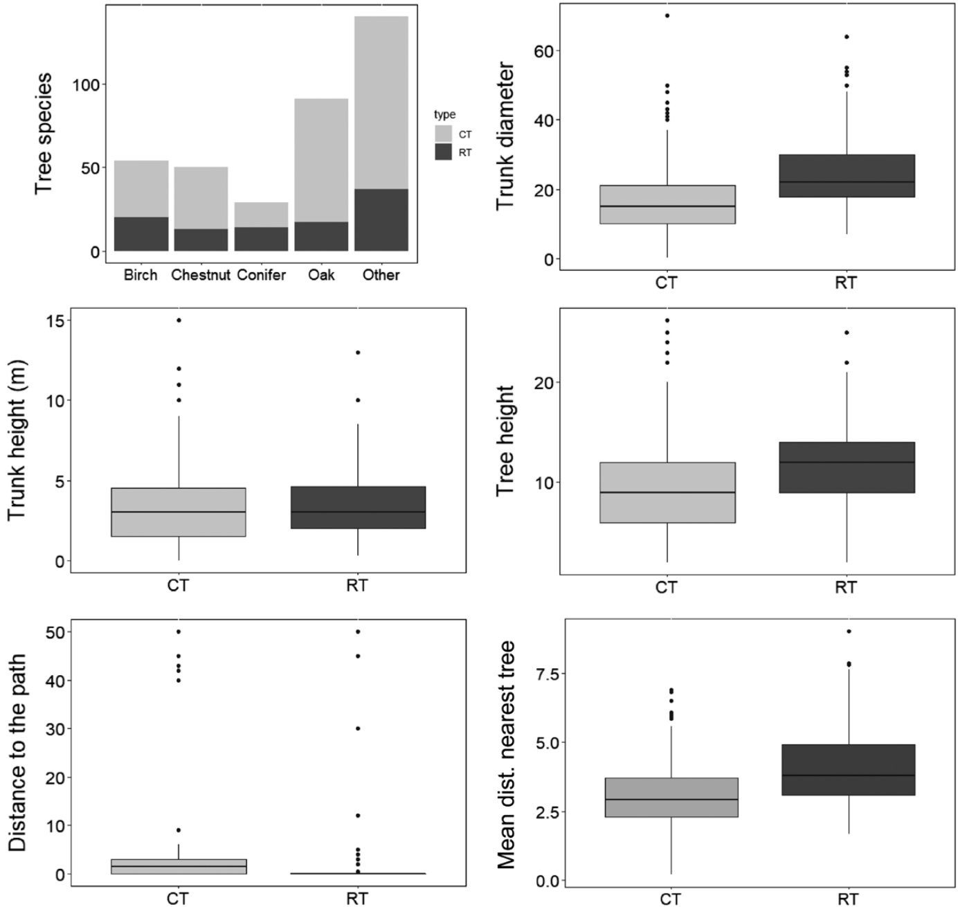
Fig. 2.—Characteristics of parameters used to describe rub trees (RTs) used by brown bears ( n = 101 RTs; dark gray) and control trees (CTs; n = 363 ; light gray) in the Cantabrian Mountains of NW Spain.
