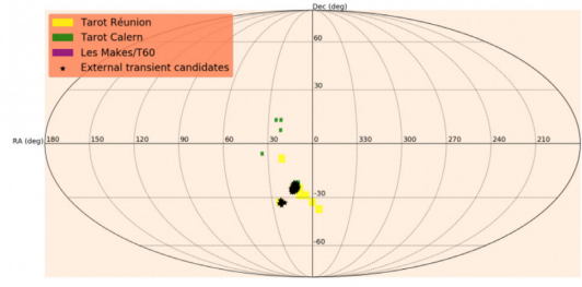
(b) S190814bv
