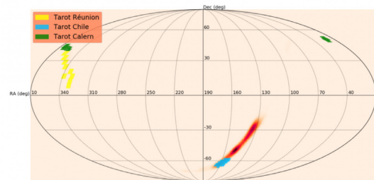
(h) S190828l
