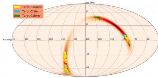
(c) S190923y
