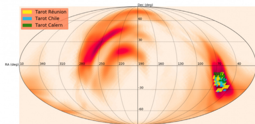
(g) S190901ap
