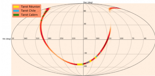
(g) S190707q
