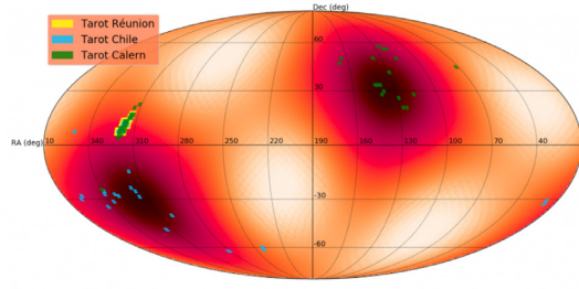
(a) S190930t
