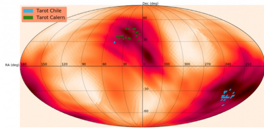
(e) S190910h
