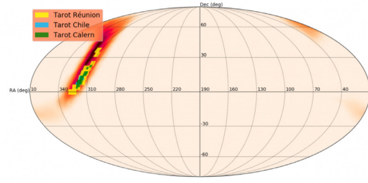
(b) S190930s
