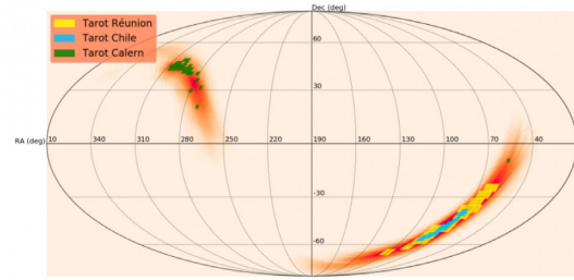
(f) S190910d
