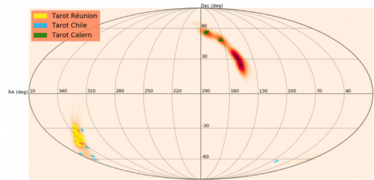
(h) S190706ai
