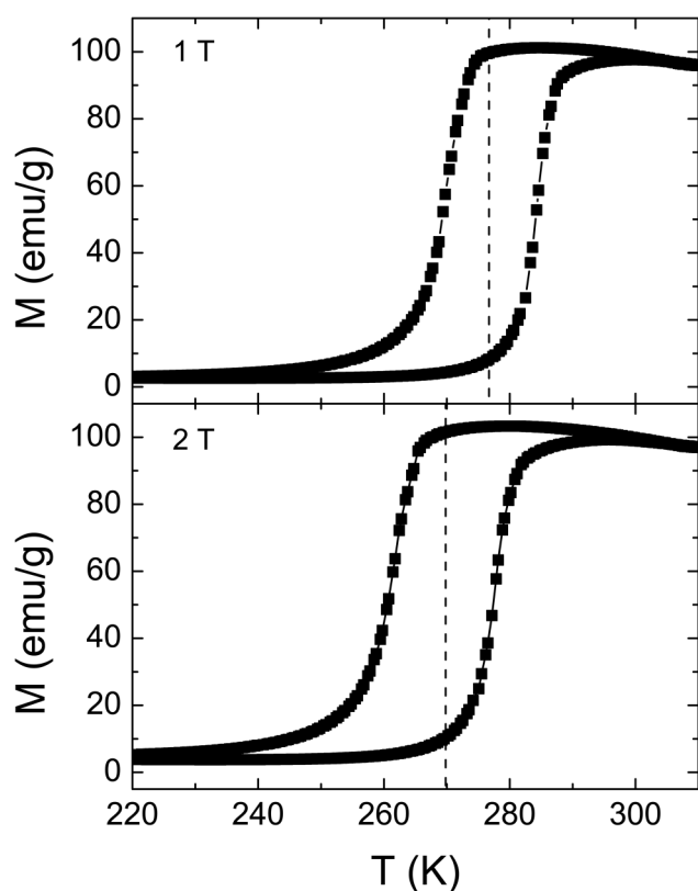
FIG. 2. Thermal hysteresis of \text{Ni}_{45.7}\text{Mn}_{36.6}\text{In}_{13.5}\text{Co}_{4.2} for applied fields of 1T and 2T. The center of the saturation loop, shifting to lower temperatures with increasing field, is marked as vertical dashed lines.
