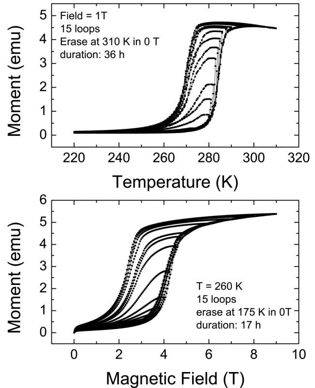
FIG. 1. Temperature and field-dependent magnetization loops, showing that the austenitic transition can be driven both by temperature and magnetic field. In between loops, the sample was taken to a completely saturated state (see Experimental for details of the procedure).
