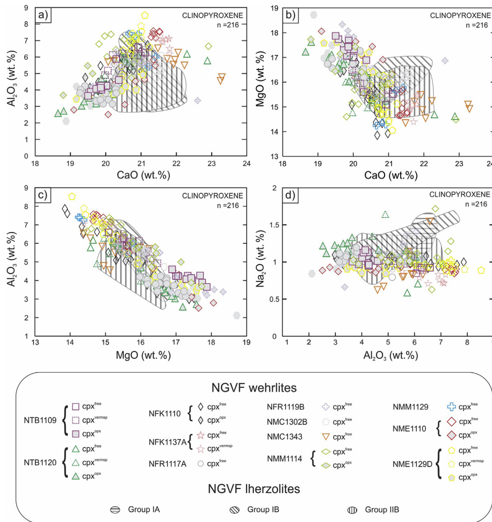
Fig. 11. Major element compositions of wehrlitic clinopyroxenes appearing in different textural positions: (a) CaO vs. Al 2 O 3 ; (b) CaO vs. MgO; (c) MgO vs. Al 2 O 3 ; (d) Al 2 O 3 vs. Na 2 O. (cpx free —vermicular spinel and orthopyroxene free clinopyroxenes; cpx vermsp —clinopyroxenes hosting vermicular spinel; cpx opx —clinopyroxenes hosting orthopyroxene) compared to distinct NGVF lherzolites of Liptai et al. (2017).
