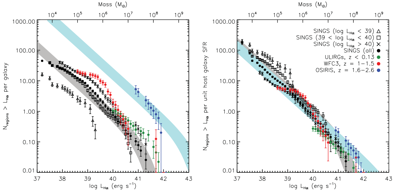
Figure 8. Cumulative LFs of H II regions in the SINGS, z \sim 1-1.5 and z \sim 2 samples, shown as a mean per galaxy (left) and normalized by total galaxy H \alpha luminosity (right). We plot the SINGS sample as a whole and subdivided into three luminosity bins. The shaded regions illustrate model predictions from the GMC mass functions of Hopkins, Quataert & Murray (2012) for Milky Way-like (grey) and high- z (blue) simulations. We find evolution in the H II region LF with redshift, which seems to be driven by the gas fraction of the disc.
