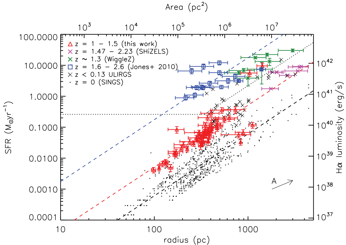
Figure 6. H\alpha SFR for extracted H\text{II} regions as a function of size, compared to the lensed z \sim 2 sample of Jones et al. (2010), high- z unlensed samples from SHiZELS (Swinbank et al. 2012) and WiggleZ (Wisnioski et al. 2012), low- z (U)LIRGs from Rodríguez-Zaurín et al. (2011) and the z = 0 SINGS galaxies (Kennicutt et al. 2003). SFRs are calculated using the Kennicutt (1998a) prescription adjusted for a Chabrier IMF with a dust extinction A_{H\alpha} = 1 in all samples, and the error bars of the high- z lensed sources are dominated by the uncertainty in the lensing magnification. Dashed lines show the median surface brightnesses in the SINGS, z \sim 1-1.5 and z \sim 2 samples. The black dotted line indicates the sensitivity limit of the z \sim 2 OSIRIS observations. The arrow indicates the effect of degrading the image resolution, as discussed in the text. The four lowest surface brightness clumps in the z \sim 1-1.5 sample come from one galaxy (MACS J1133), and the two brightest regions are from Abell 773, the most compact galaxy in the sample. The remaining galaxies have clumps with surface brightnesses in between those of the z = 0 and z \sim 2 samples, similar to local (U)LIRGs.
