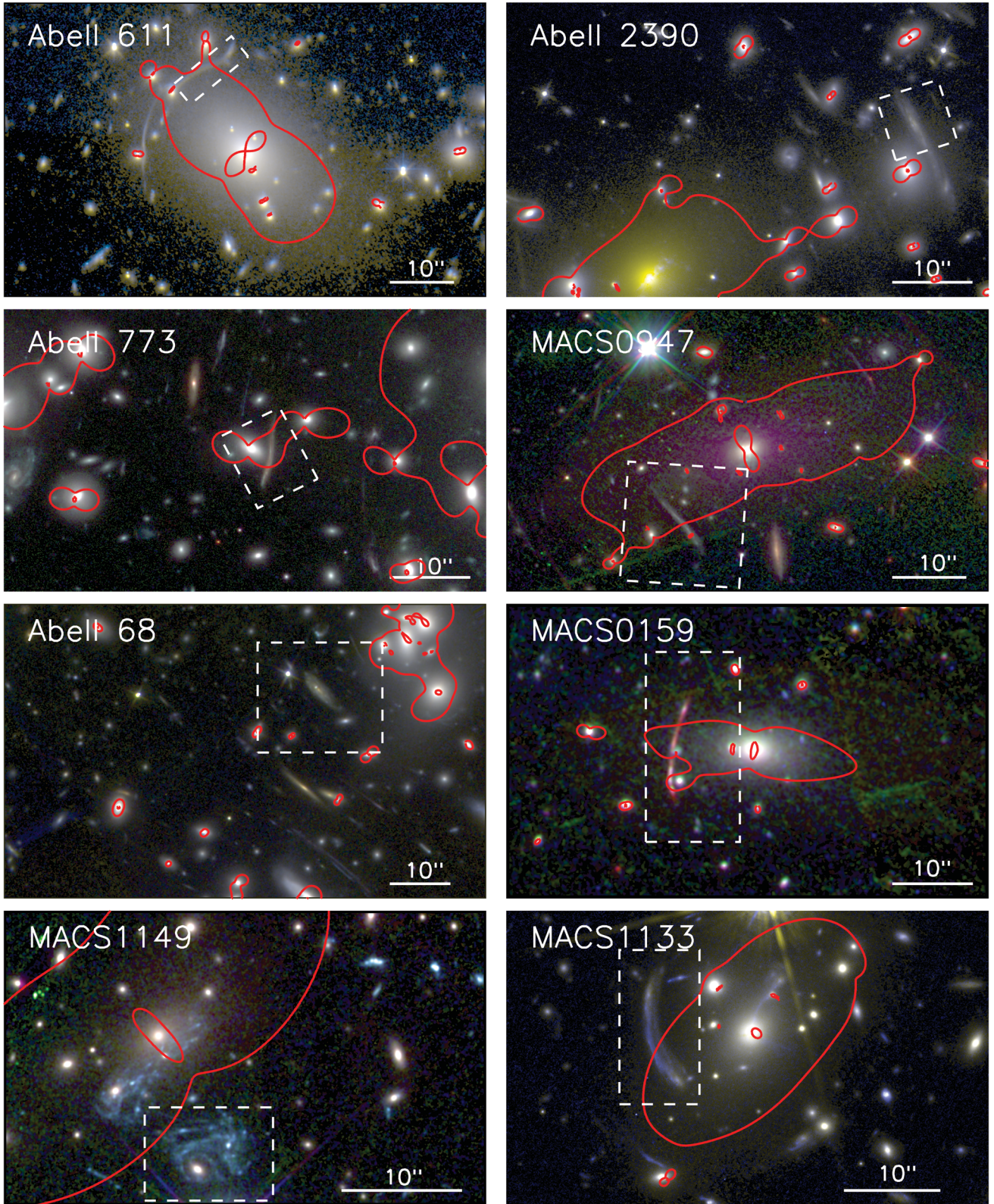
Figure 1. HST /ACS and WFC3 three-colour images of the observed clusters with the critical line at the redshift of the target arc overlaid, showing the positions of the target arcs. The arcs are contained within the white dashed boxes which denote the regions extracted in Fig. 2.
