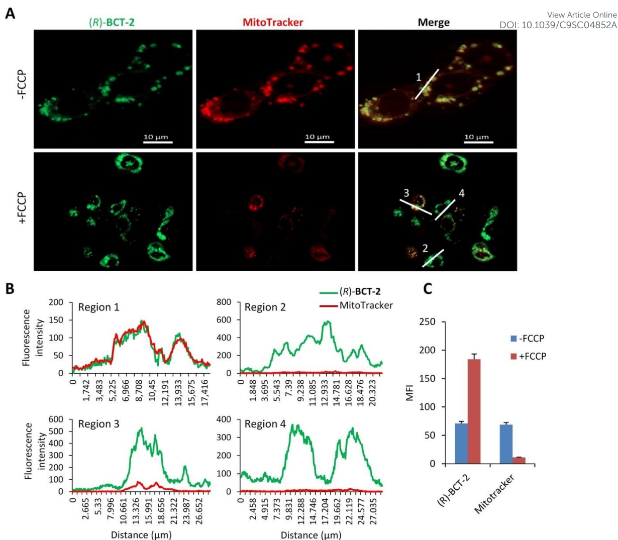
Figure 5. Mitochondrial labelling by ( R )- BCT-2 does not depend on \Delta\Psi_m . (A) Microscopic analysis of SCC38 cells pretreated or not with FCCP before co-labelling with 20 nM ( R )- BCT-2 and 0.5 nM MitoTracker. Scale bars, 10 \mu\text{m} . (B) Graphic shows the fluorescence intensity profiles of the regions of interest indicated with white lines in right panels. (C) Data represent the mean fluorescence intensity (MFI) of labelled cells from flow cytometry analysis of SCC38 cells incubated in the presence (+FCCP) or absence (–FCCP) of 60 \mu\text{M} FCCP for 3 h, before labelling with either 20 nM ( R )- BCT-2 or 0.5 nM Mitotracker.
