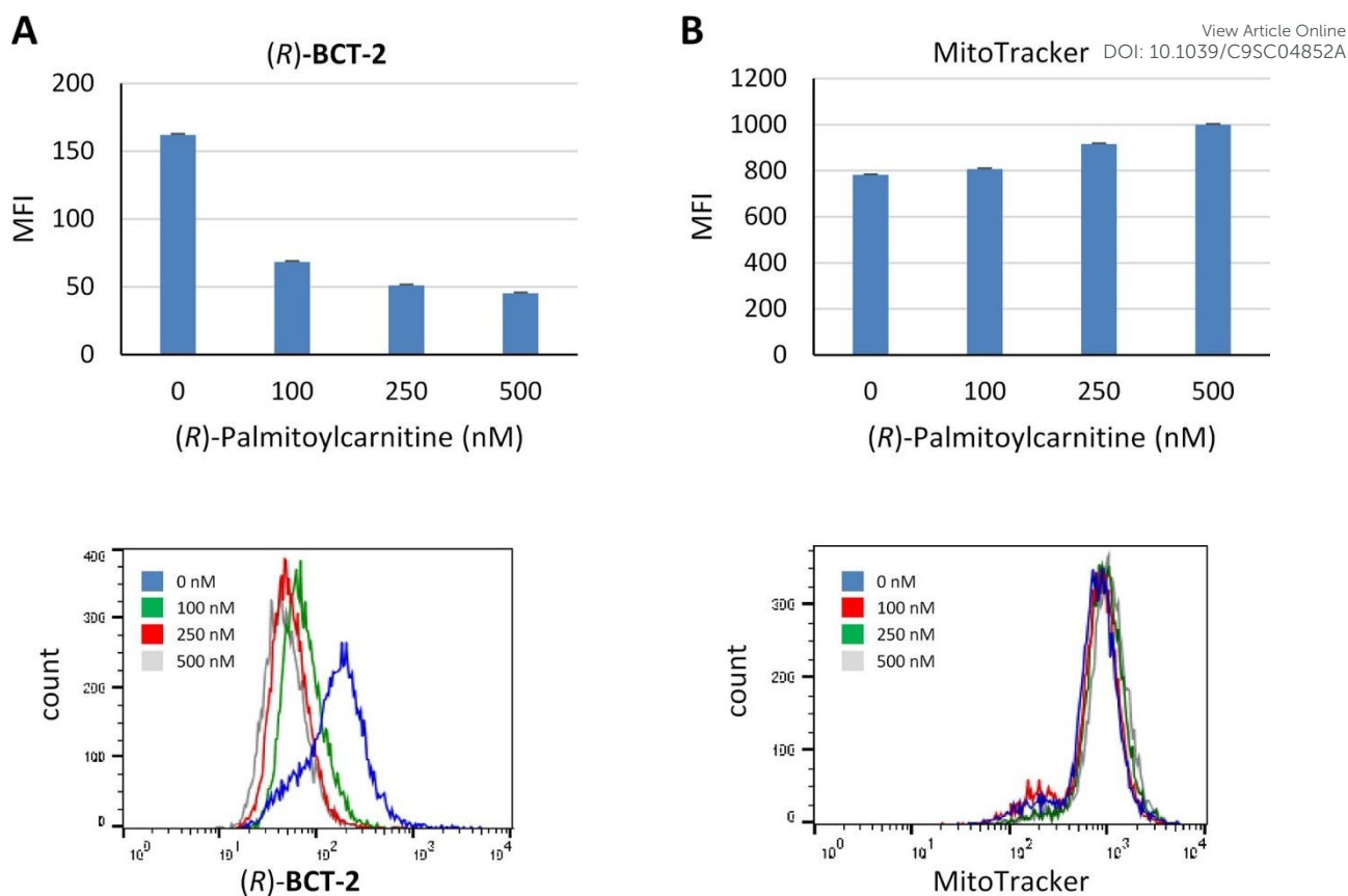
Figure 7. Inhibition of mitochondria staining with (R) -BCT-2 in the presence of increasing concentrations of (R) -palmitoylcarnitine. SCC38 cells were co-incubated with the indicated concentrations of (R) -palmitoylcarnitine and 50 nM (R) -BCT-2 (A) or 50 nM MitoTracker (B) prior to analysis by flow cytometry. Data represent the mean fluorescence intensity (MFI) of labelled cells (upper panels) and representative images of flow cytometry profiles (lower panels).
