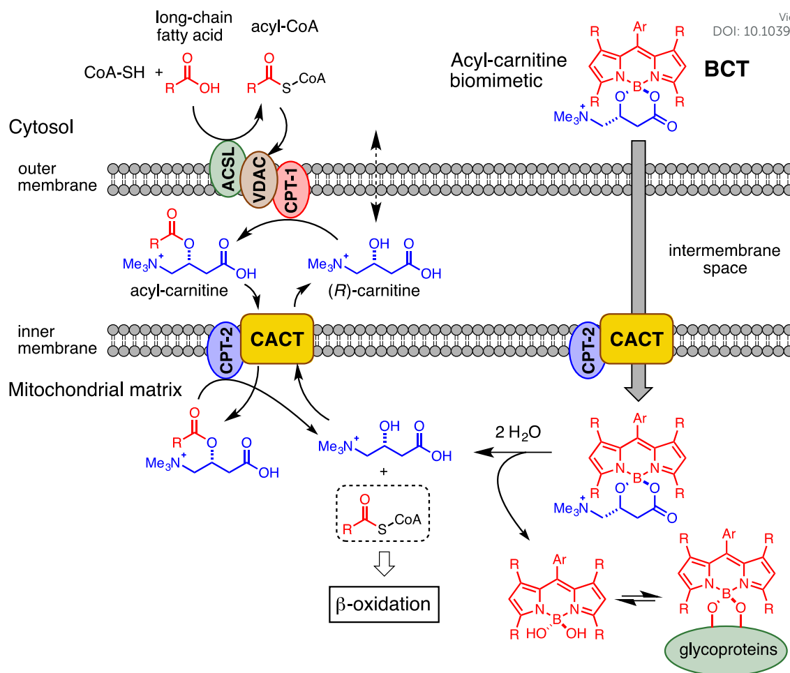
Figure 6. Mechanistic hypothesis for the transport (and fate) of BCT probes into the mitochondrial matrix via the carnitine shuttle system.
