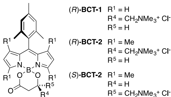
Scheme 1. General molecular design of the BODIPY-carnitine BCT probes and structures of the starting components and final probes synthesized.
