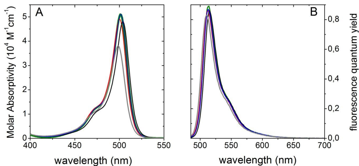
Figure 1. Absorption (height-normalized to molar absorptivity) (A) and fluorescence (height-normalized to quantum yield) (B) spectra of the ( R )- BCT-2 probe in different solvents; chloroform (green), acetone (black), acetonitrile (red), ethanol (blue), and water (grey).
