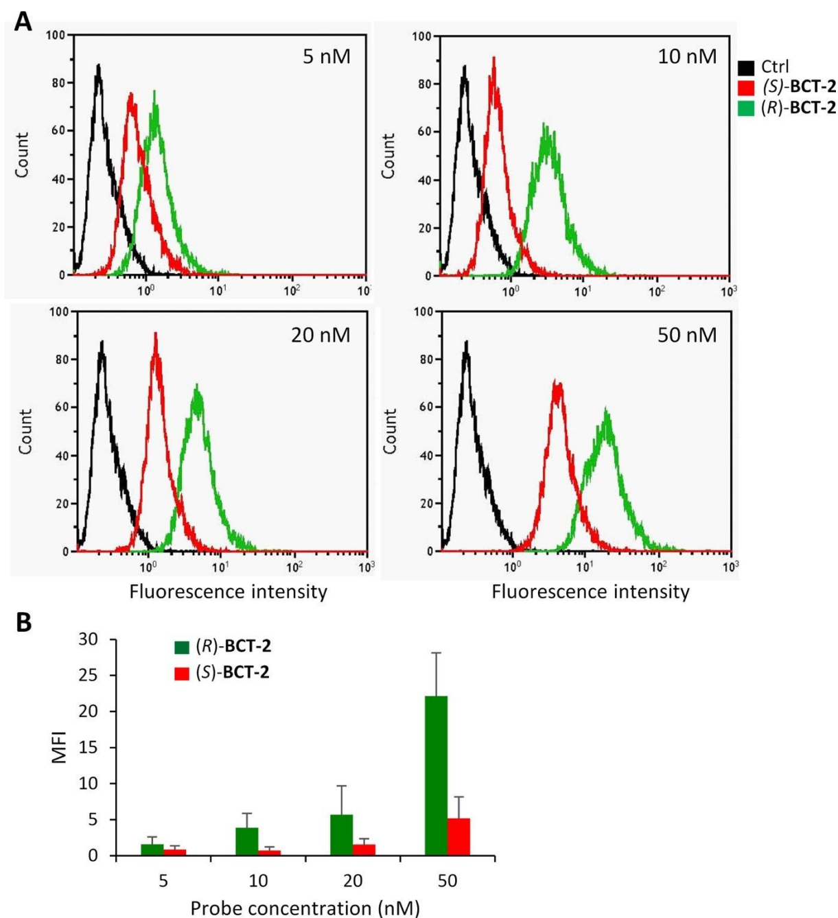
Figure 9. Flow cytometry analysis of SCC38 cells labelled with increasing concentrations of ( R )-BCT-2 or ( S )-BCT-2. The cells were incubated with the indicated concentrations of the probes for 30 min before flow cytometry analysis. (A) Representative images of flow cytometry profiles. (B) Data represent the mean fluorescence intensity of labelled cells.
