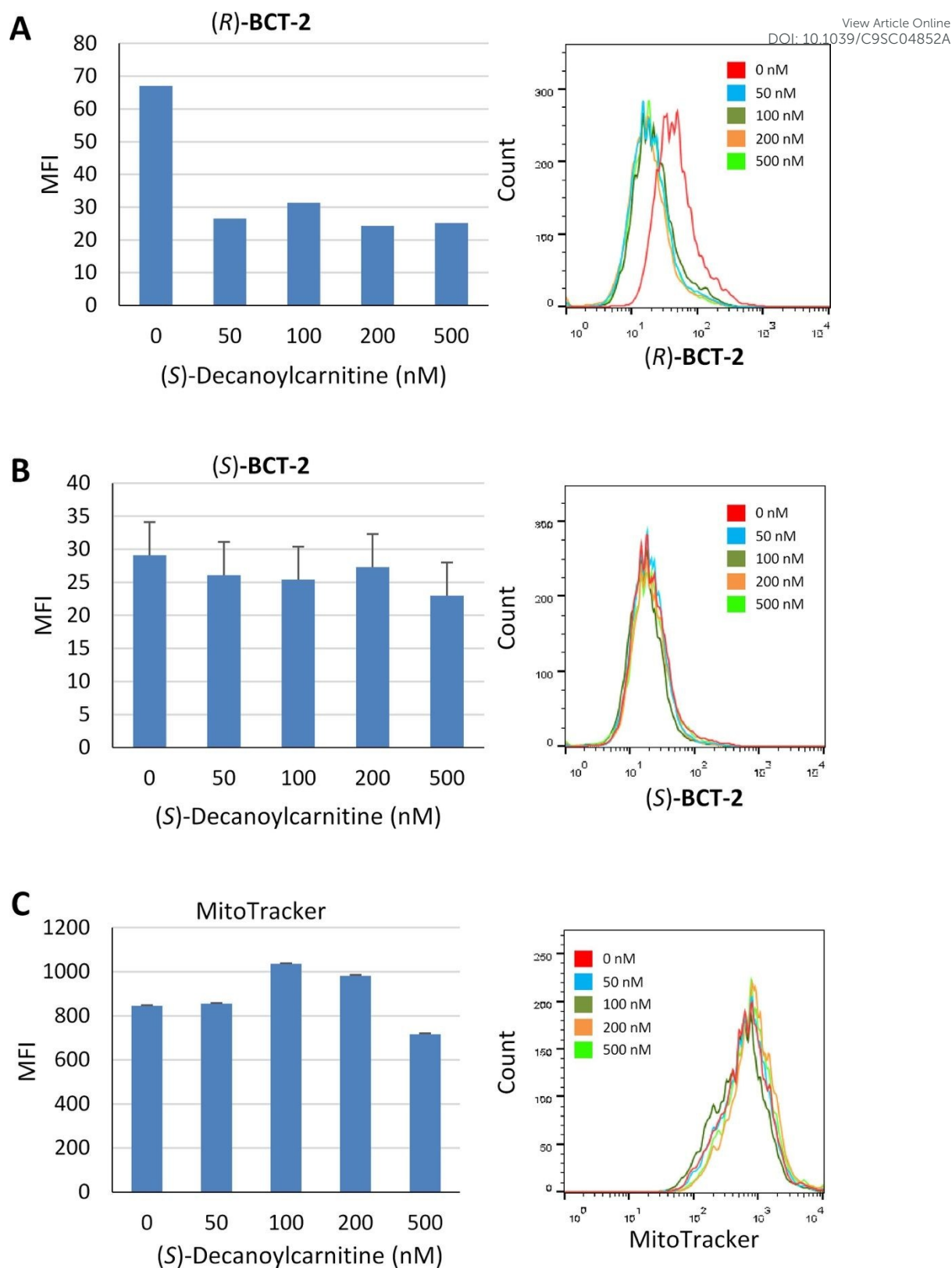
Figure 8. Inhibition of mitochondria staining in the presence of increasing concentrations of ( S )-decanoylcarnitine. SCC38 cells were co-incubated with the indicated concentrations of ( S )-decanoylcarnitine and 50 nM solutions of ( R )-BCT-2 (A), ( S )-BCT-2 (B), or MitoTracker (C), prior to analysis by flow cytometry. Data represent the mean fluorescence intensity (MFI) of labelled cells (left panels) and representative images of flow cytometry profiles (right panels).
