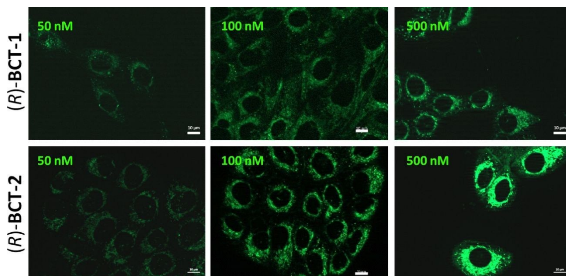
Figure 2. Dose-dependent cellular distribution of ( R )- BCT-1 and ( R )- BCT-2 compounds. Representative fluorescence images of live SCC38 cells incubated with the indicated concentrations of ( R )- BCT-1 and ( R )- BCT-2 compounds for 30 min before washing and microscopic analysis under the same acquisition conditions. Scale bars, 10 \mu m.
