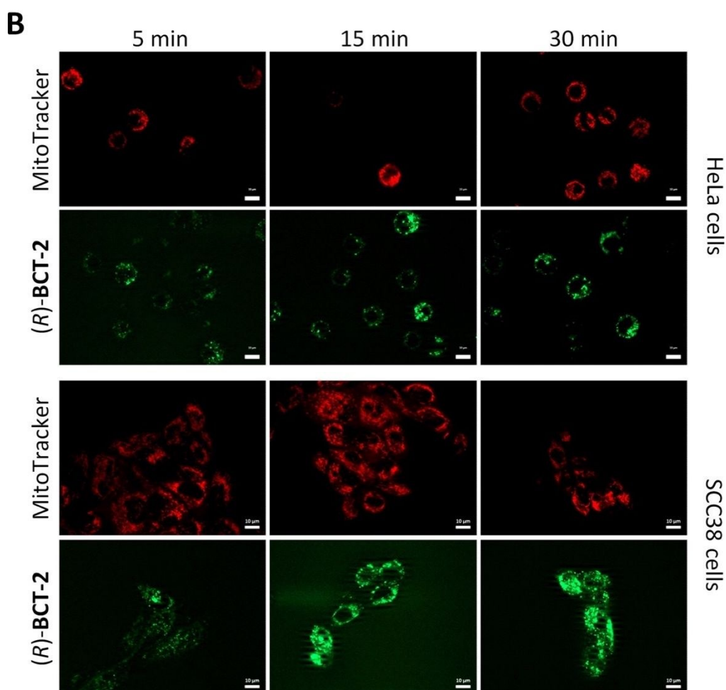
Figure 4. Mitochondria staining by ( R )-BCT-2 is time-dependent. HeLa or SCC38 cells were incubated with either 50 nM ( R )-BCT-2 or 50 nM MitoTracker Red CMXRos for the indicated times before cell washing and analysis by flow cytometry (A) or microscopy (B). Scale bars, 10 \mu m.
