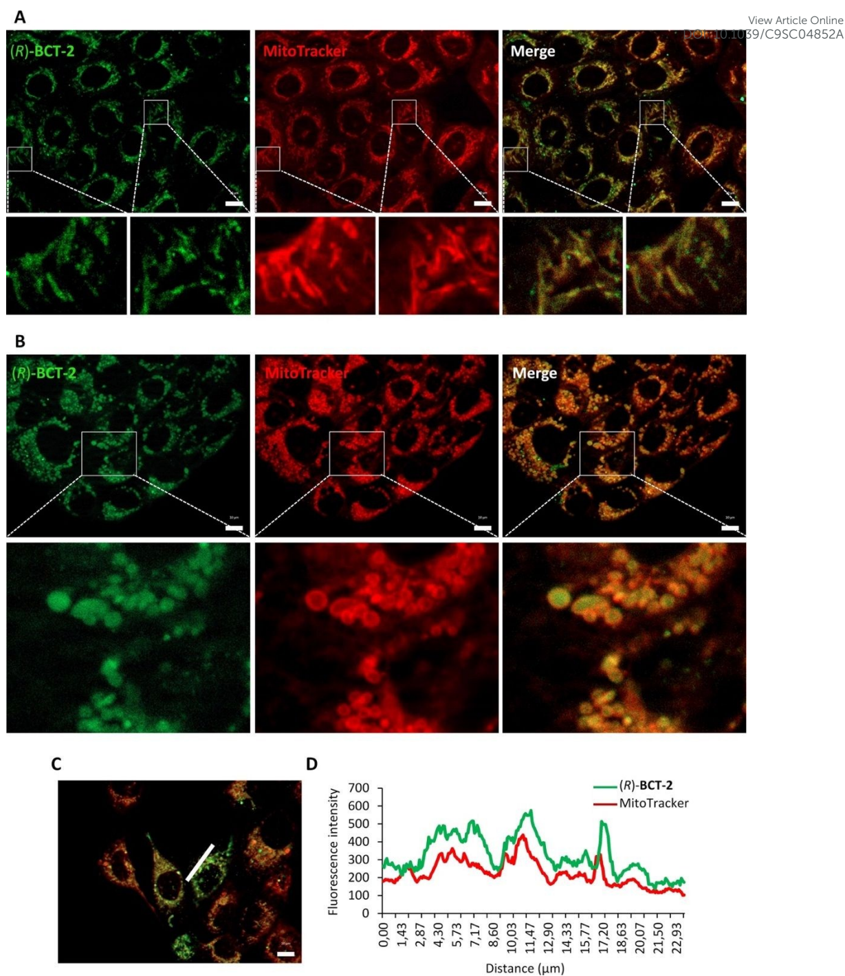
Figure 3. Colocalization of (R)-BCT-2 and MitoTracker Red CMXRos fluorescence signals in SCC38 cells. (A, B, C) Representative fluorescence images of SCC38 cells co-labelled with 50 nM (R)-BCT-2 and 50 nM MitoTracker Red CMXRos for 30 minutes before microscopic analysis. Magnified images of the areas indicated in panels A and B are shown to better visualize the staining of tubular (A) and spherical (B) mitochondria. (D) Graphic shows the fluorescence intensity profiles of the region of interest indicated with a white line in panel C. Scale bars, 10 \mu\text{m} .
