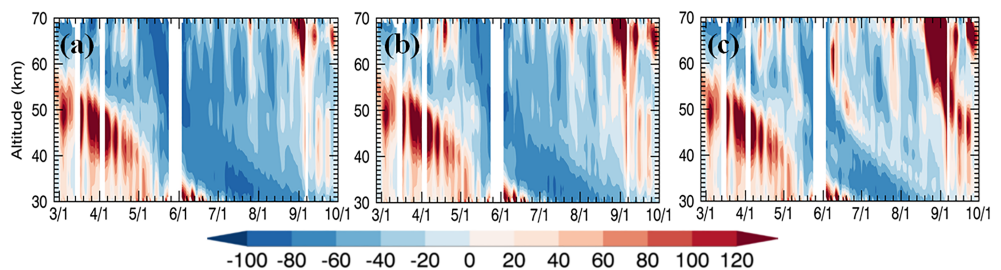
Figure 5. Differences between Michelson Interferometer for Passive Atmospheric Sounding (MIPAS) and Whole Atmosphere Community Climate Model (WACCM) \text{NO}_x mixing ratios [100 \times (\text{WACCM} - \text{MIPAS}) / \text{MIPAS}] for (a) the baseline, (b) Coupled Model Intercomparison Project version 6 (CMIP6), and (c) MP15 simulations. All panels are averaged from 70^\circ\text{S} to 90^\circ\text{S} . Model results are taken at the MIPAS times and satellite locations.
