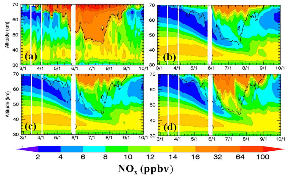
Figure 6. \text{NO}_x mixing ratios averaged over 40\text{--}50^\circ\text{S} , from (a) Michelson Interferometer for Passive Atmospheric Sounding (MIPAS) and from (b) the baseline, (c) Coupled Model Intercomparison Project version 6 (CMIP6) and (d) MP15 Whole Atmosphere Community Climate Model (WACCM) simulations at the times and locations of the MIPAS measurements. The dashed black line denotes the MIPAS 16 ppbv \text{NO}_x contour.
