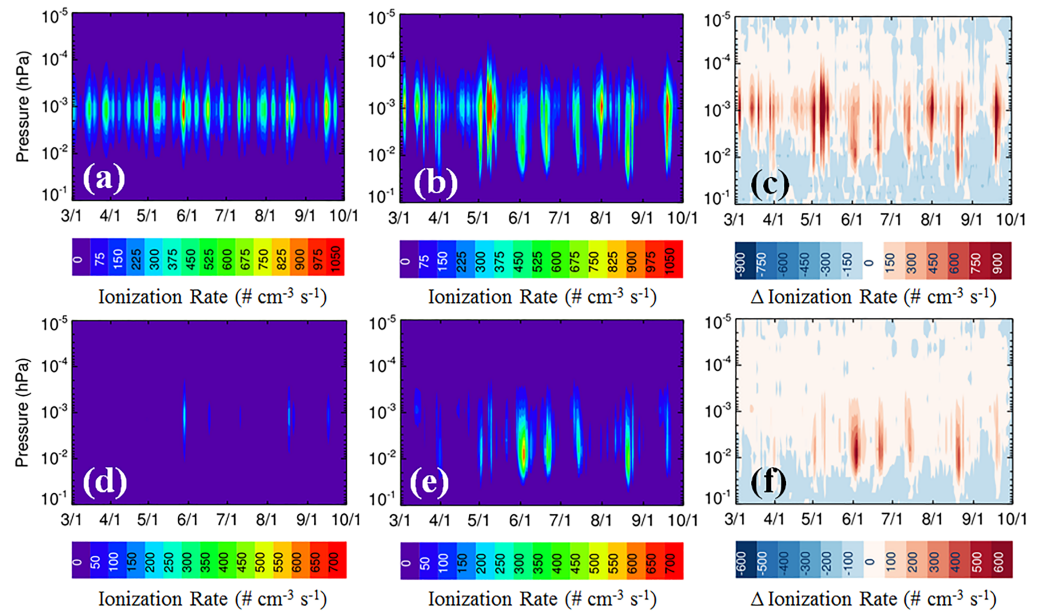
Figure 2. Energetic electron ionization rates for 2003, averaged from (top) 50–80°S and (bottom) 30–50°S, from (a and d) Coupled Model Intercomparison Project version 6 (CMIP6) and (b and e) MP15. (c and f) The ionization rate differences are shown.
