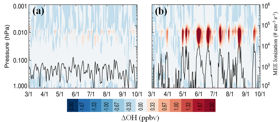
Figure 3. (a) Coupled Model Intercomparison Project version 6 (CMIP6) and (b) MP15 model simulations minus the baseline simulation for OH mixing ratios averaged from 50–80°S. The black line indicates the medium energy electron ionization at 0.01 hPa for the respective simulations.
