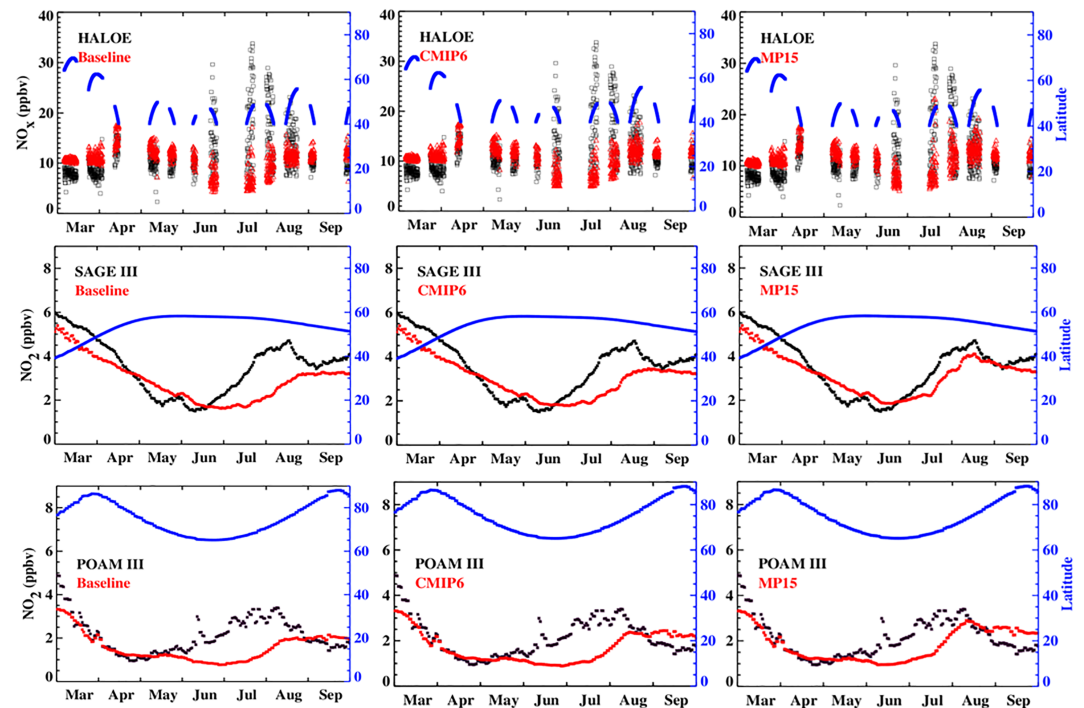
Figure 7. Comparisons of observations of (top row) \text{NO}_x at 45-km altitude from Halogen Occultation Experiment (HALOE), and \text{NO}_2 at 40 km from (middle row) Stratospheric Aerosol and Gas Experiment (SAGE) III and (bottom row) Polar Ozone and Aerosol Measurement (POAM) III, with results from the (left column) baseline, (middle) Coupled Model Intercomparison Project version 6 (CMIP6) and (right) MP15 simulations at the corresponding measurement locations and times. HALOE plots show all individual measurements poleward of 40^\circ\text{S} , POAM and SAGE plots show 7-day running means, measurement latitudes are shown in blue and referenced to the right axis.
