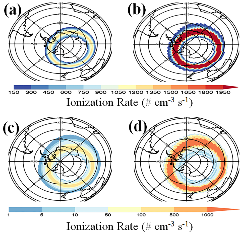
Figure 1. Energetic electron ionization rates at 90 km (top) for 11 May 2003 from (a) Coupled Model Intercomparison Project version 6 (CMIP6) and (b) MP15 and 75 km (bottom) for 2 May 2003 from (c) CMIP6 and (d) MP15.
