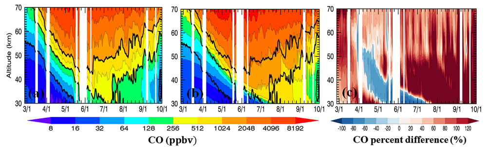
Figure 8. CO mixing ratios from (a) Michelson Interferometer for Passive Atmospheric Sounding (MIPAS) and (b) baseline Whole Atmosphere Community Climate Model (WACCM) and (c) CO percent differences, 100 \times (\text{WACCM-MIPAS}) / \text{MIPAS} . Panels show averages from 70 to 90°S during March–September 2003. Model results are taken at the MIPAS times and satellite locations. The black lines indicate the MIPAS 32, 256, and 1,024 ppbv CO contours for reference.
