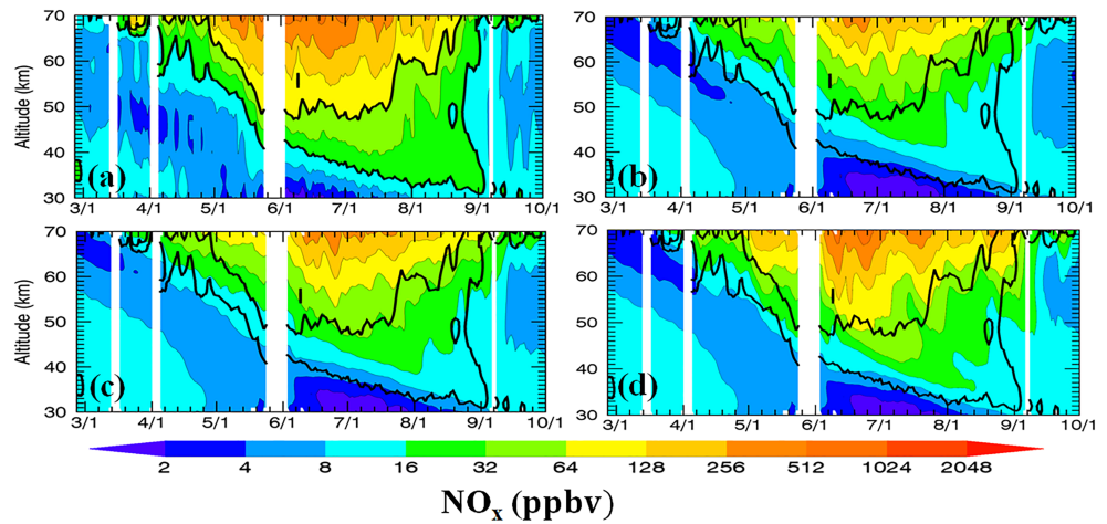
Figure 4. \text{NO}_x mixing ratios averaged over latitudes from 70^\circ\text{S} - 90^\circ\text{S} , from (a) Michelson Interferometer for Passive Atmospheric Sounding (MIPAS) and from (b) the baseline, (c) Coupled Model Intercomparison Project version 6 (CMIP6), and (d) MP15 Whole Atmosphere Community Climate Model (WACCM) simulations at the times and locations of the MIPAS measurements. The black lines denote the MIPAS 16 and 64 ppbv \text{NO}_x contours. White regions indicate missing MIPAS data or regions where MIPAS errors were >200\% .
