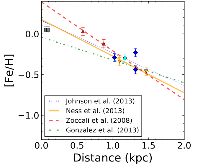
Fig. 9. Metallicity measurements at different latitudes reported by previous studies: red triangles correspond to (l, b) = (+1, -4) and (0, -6) fields from Zoccali et al. (2008), blue diamonds are from Johnson et al. (2013) and correspond to (l, b) = (8.5, 9), (-5.5, -7) and (-4, -9) , the inverted yellow triangles correspond to (l, b) = (0, -7.5) and (0, -10) from Ness et al. (2013), the cyan circle corresponds to (0, -8) from Johnson et al. (2011), and the grey squares are from this work. The lines show several metallicity gradients obtained by the authors in the legend. The lines and points share the same colour if they are part of the same work.
