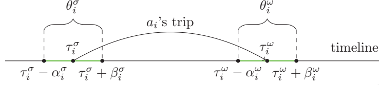
Figure 5: Example of departure and arriving time constraints.
