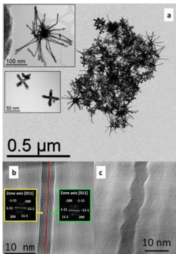
Fig. 2 (a) TEM image of the nano-objects obtained at 100°C (24 h of reaction). In the insets magnifications of the two types of objects obtained: multipods and octopods with outgrown domains on the branches. (b), (c) two HRTEM images corresponding to two different orientations of the multipods branches. The red line in (b) corresponds to a twin (111) type plane.
