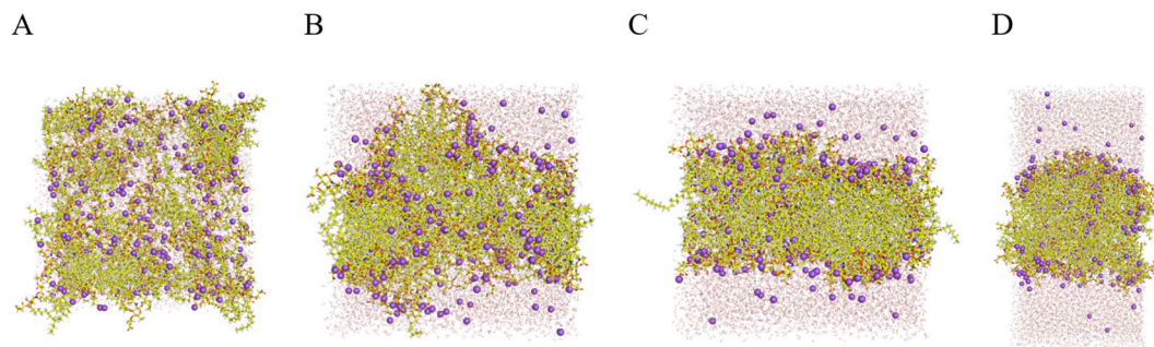
Figure 6. Representation of the evolution of the FP15-water mixture over time, t = 0 ns (A), t = 50 ns (B), t = 200 ns (C) and t = 1000 ns (D). FP15 is represented in CPK colored sticks, ion \text{Na}^+ in violet spheres and the water molecules in thin grey and red lines.
