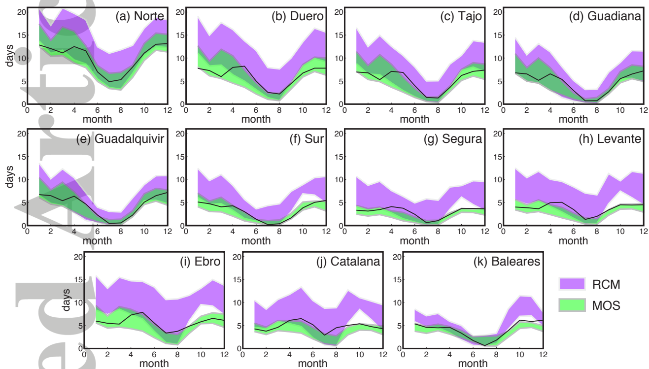
Figure 5. Seasonal cycle of the spatially averaged R1 index (in days) for each river basin (according to Fig. 1). The black line represents the observed (Spain02) climatology. The violet shaded band spans the values for the RCMs while the green one spans the respective MOS downscaled values.
