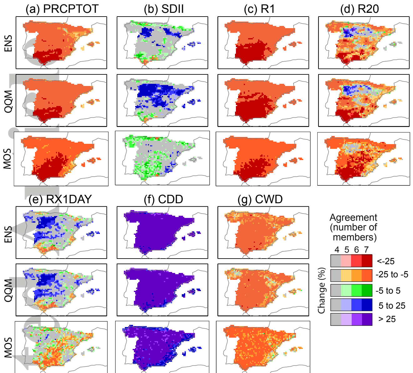
Figure 7. Future climate change signals (expressed as percentage of change with regards the baseline control period 1971-2000) for the period 2071-2100 for the precipitation indices shown in Table 2. The different rows correspond to the results for the seven-member ensemble (ENS), the quantile mapping bias correction method (QQM), and the MOS-Analog downscaling method. The colour saturation level shows the percentage agreement in the direction of change among the ensemble members.
