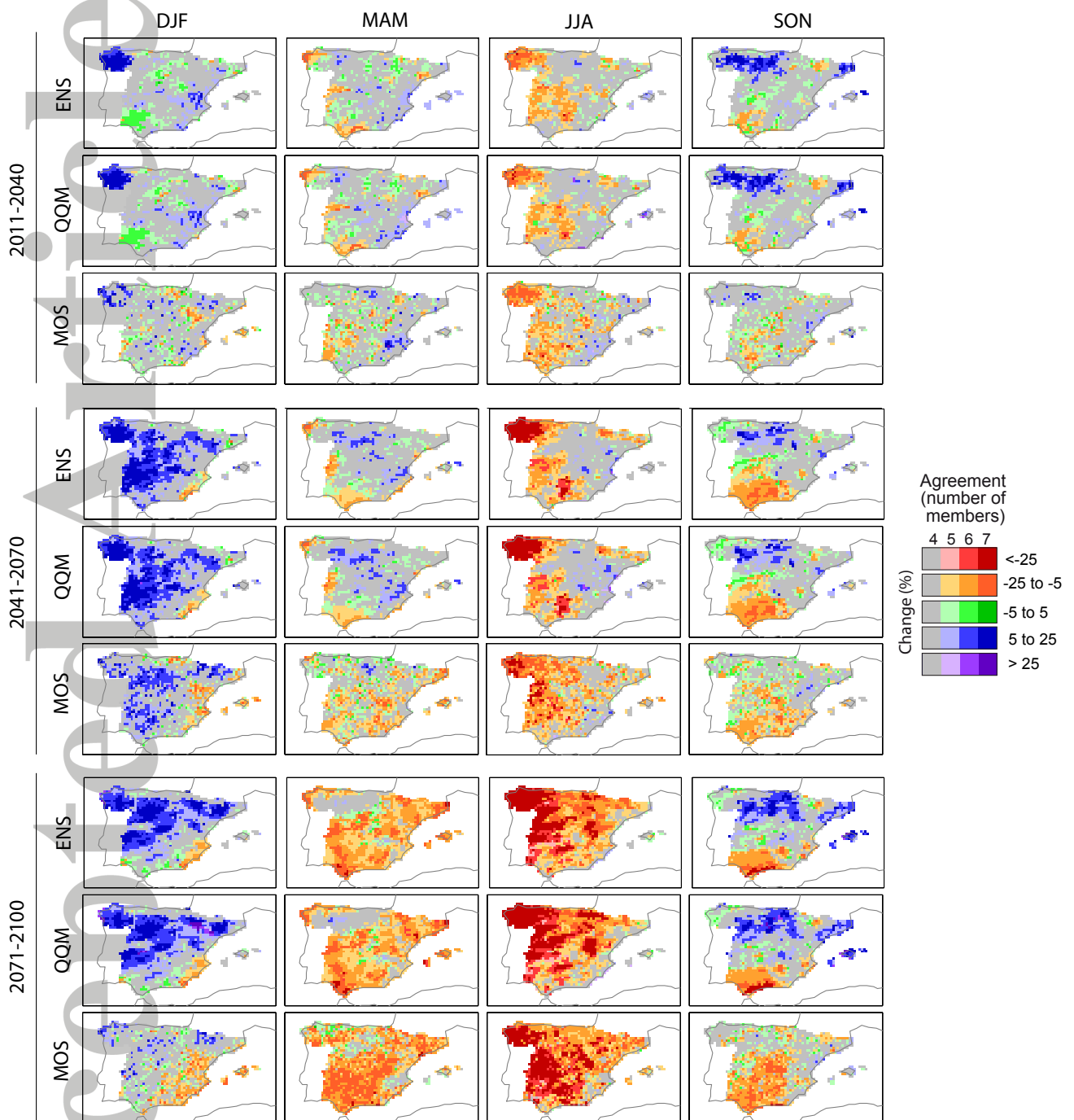
Figure 9. The same as Fig. 8 but for RX1DAY index.
