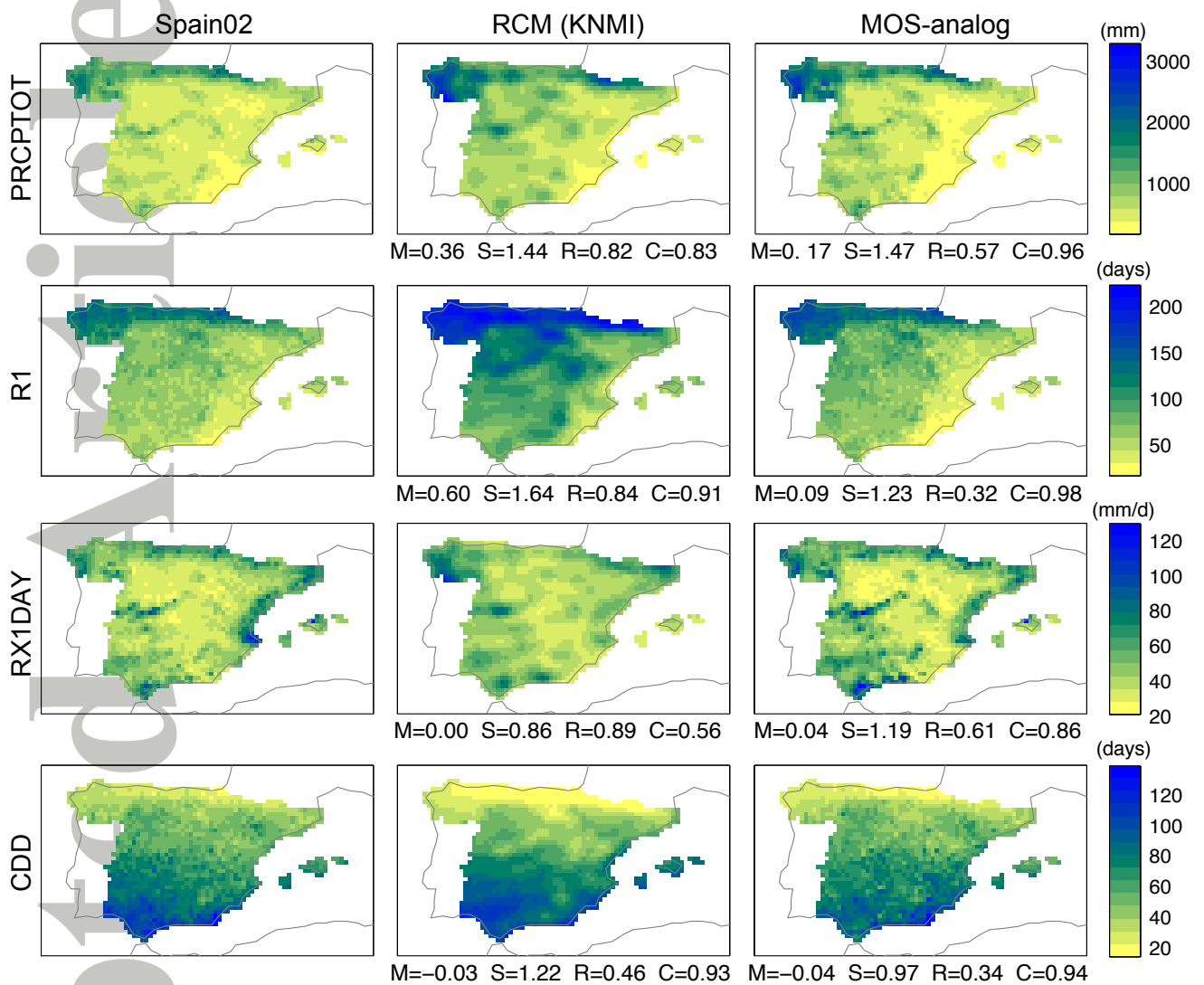
Figure 3. Spatial distribution of the observed (Spain02, left), RCM (central) and MOS-Analog (right) mean values (averaged over the baseline period 1971-2000) for some of the precipitation indices shown in Table 2. The spatial validation scores for the RCM and MOS-Analog simulated values are given below the corresponding panels: mean error M (in % w.r.t. the observed mean); the relative standard deviation S ; the centred root-mean-square R ; the correlation C .
