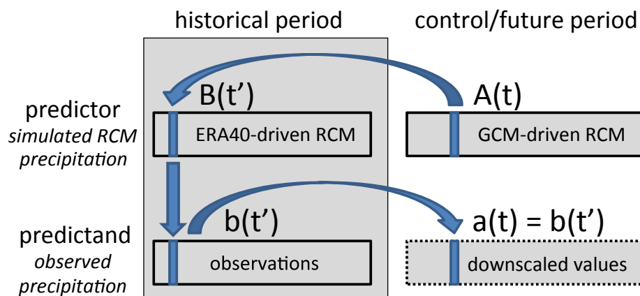
Figure 2. Schematic illustration of the MOS-Analog method (adapted from Fernandez and Saenz, 2003 ). See the text for details.
