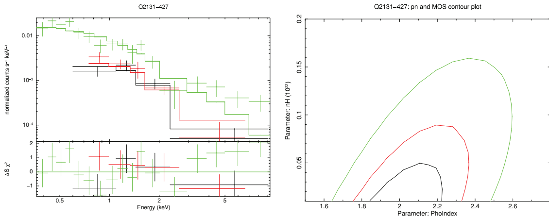
Figure 4. XMM-Newton observation of Q2131–427. Left-hand panel: the EPIC pn, MOS1 and MOS2 spectra, best-fitting models and \Delta\chi^2 deviations. Right-hand panel: column density versus photon index contour plots at 68, 90 and 99 per cent confidence level for two interesting parameters.
