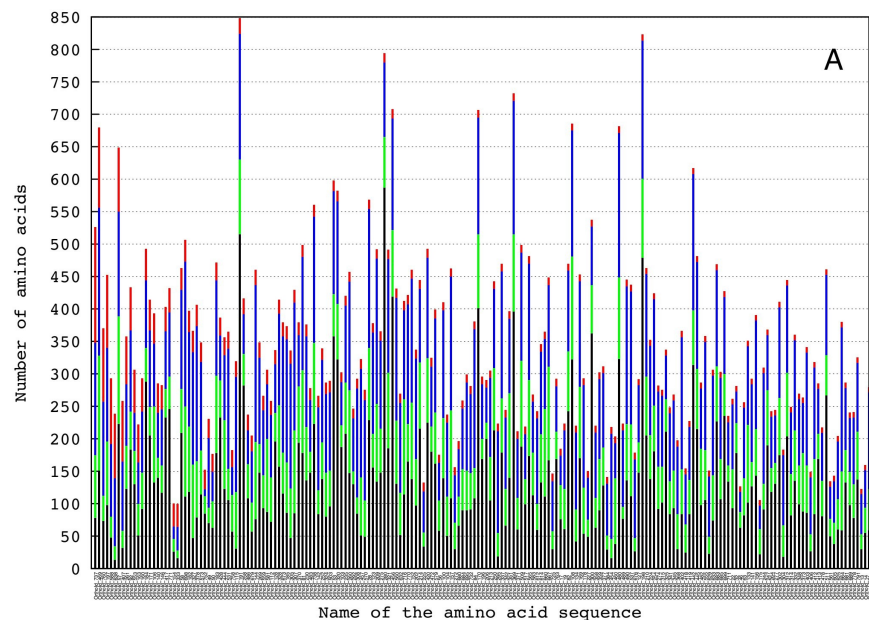
Figure S1. Amino-acids from the studied sequences: black – constant, green – variable parsimony-uninformative, blue – parsimony-informative, red – variable within aciculiferum/malmogiense clade.
