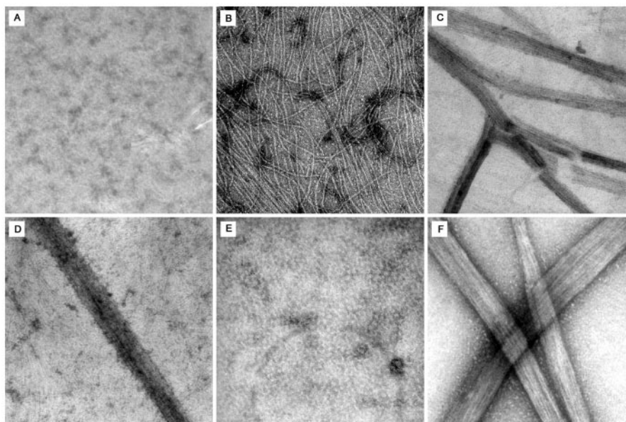
FIG. 3. Electron microscopy analysis of FtsZ assembly in the absence and in the presence of macromolecular crowders. Top row, left-hand side: electron micrograph of negative stained FtsZ (1.0 g/liter) samples in 50 mM Tris-HCl, 100 mM NaCl, pH 7.4, buffer (which does not contain potassium and does not promote FtsZ assembly, see Ref. 13) plus 1 mM GTP and 200 g/liter Ficoll 70. The other electron micrographs correspond to negatively stained FtsZ samples in KGA buffer. Top row, center: FtsZ (0.5 g/liter) plus 1 mM GTP. Top row, right-hand side: FtsZ (0.2 g/liter) plus 2 mM GTP and 220 g/liter Ficoll 70. Bottom row, left-hand side: FtsZ (0.1 g/liter) plus 2 mM GTP and 200 g/liter dextran T70. Bottom row, center: FtsZ (0.5 g/liter) plus 0.5 mM GTP and 200 g/liter Ficoll 70 after 1-h incubation at 30 °C. Bottom row, right-hand side: FtsZ (0.5 g/liter) plus 0.1 mM GMPCPP and 200 g/liter Ficoll 70. In all cases, the bar scale is 100 nm.
