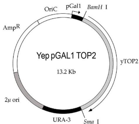
Figura M1. Yep pGAL1-TOP2
